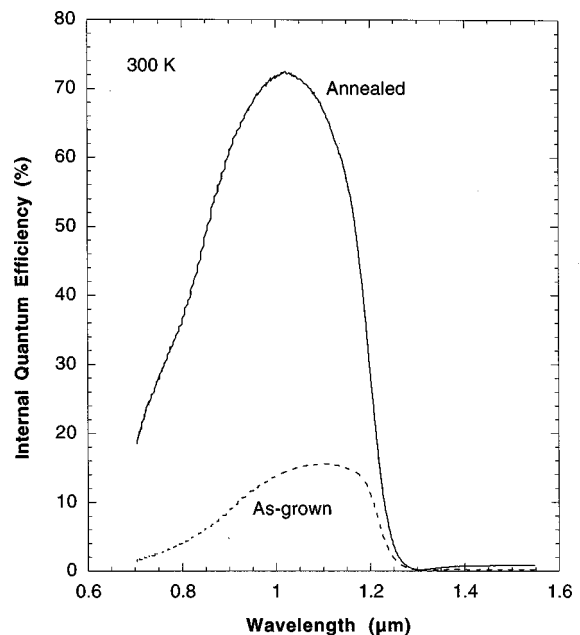
FIG. 2. Internal quantum efficiency curves for as-grown (0 V bias, 0.15 \mu\text{m} depletion width) and ex situ annealed (0 V bias, 0.26 \mu\text{m} depletion width) \text{In}_{0.07}\text{Ga}_{0.93}\text{As}_{0.98}\text{N}_{0.02} solar cells with 1.0 \mu\text{m} thick, n -type emitters.
