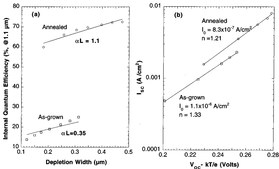
FIG. 3. (a) Internal quantum efficiency vs depletion width for the as-grown and annealed solar cells. Model (solid lines) assumes that the ratio of the n - and p -type doping concentrations is unchanged by annealing. (b) Measured solar cell open-circuit voltage ( V_{oc} ) and short-circuit current ( I_{sc} ) for various light intensities.
