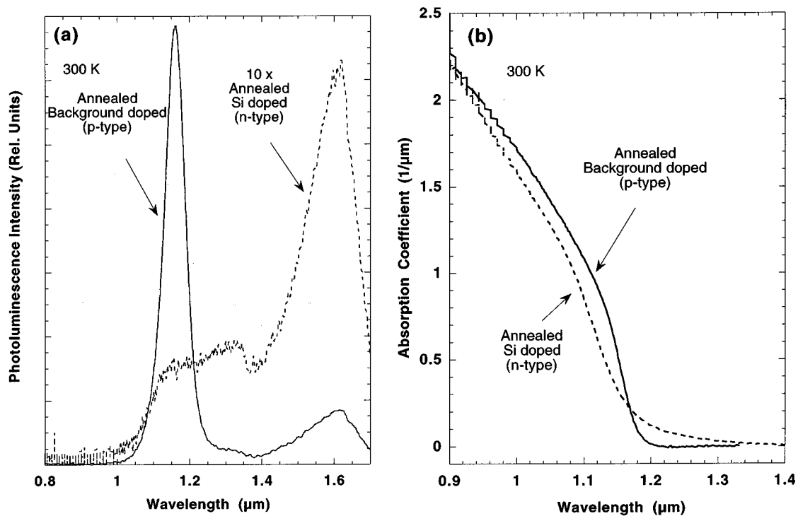
FIG. 1. (a) Photoluminescence spectra for ex situ annealed, p -type (background doped, 4 \times 10^{16}/\text{cm}^3 ) and n -type (Si doped, 2 \times 10^{17}/\text{cm}^3 ) \text{In}_{0.07}\text{Ga}_{0.93}\text{As}_{0.98}\text{N}_{0.02} epitaxial films. (b) Absorption spectra for the samples in (a).
