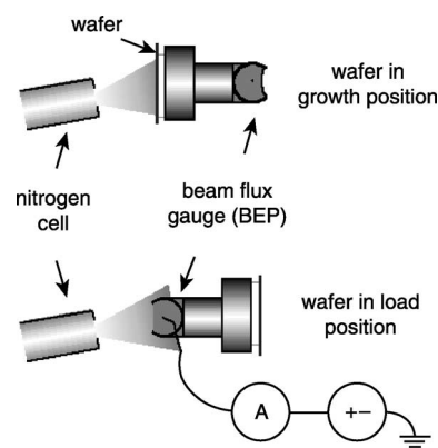
Fig. 6 Schematic of MBE substrate holder/beam flux monitor and its use to measure ion/electron currents from RF N plasma source
