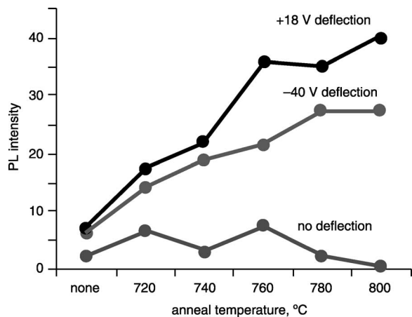
Fig. 8 Photoluminescence for samples grown with different voltages applied to one deflection plate
