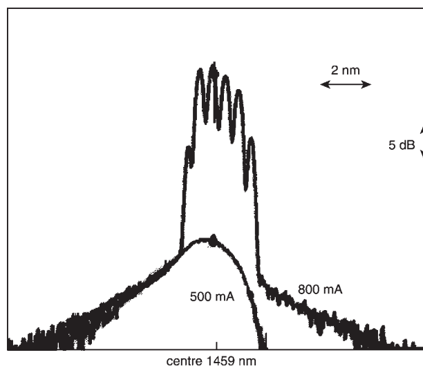
Fig. 11 Spectra of the first monolithic \lambda > 1.45 \mu\text{m} VCSEL on GaAs operating just below and about 1.6 times threshold
