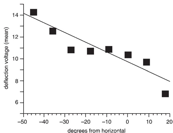
Fig. 7 Deflection of ions with applied bias on a single deflection plate
