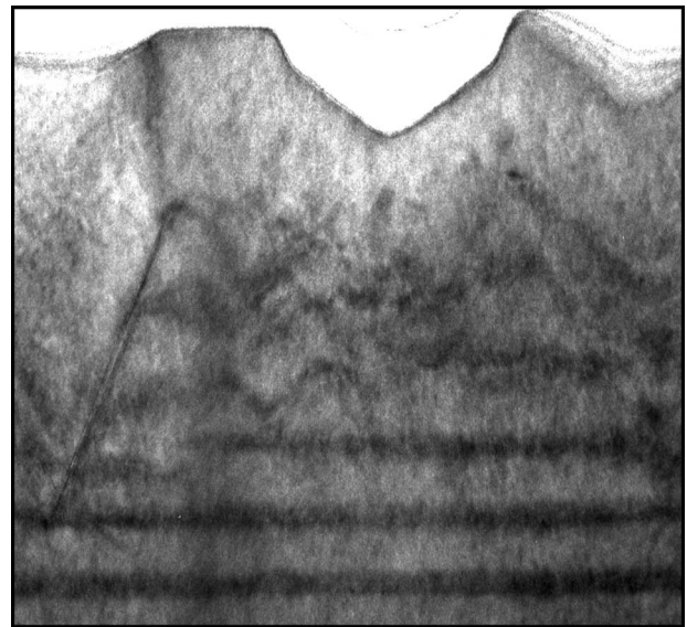
Fig. 2 TEM cross-section image of 3-QW 35% In GaInNAs-GaAs barrier sample where 3-D growth and phase segregation have occurred in the 3rd QW
