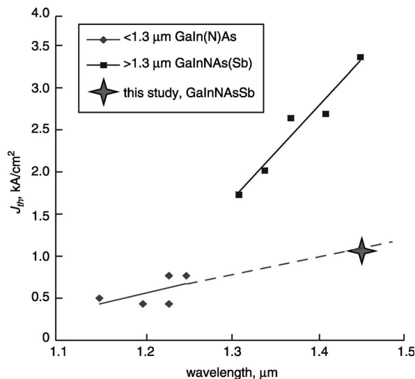
Fig. 10 Threshold current of GaInNAs lasers ( 1.15 < \lambda < 1.25 \mu\text{m} ) from several groups and our earlier GaInNAsSb lasers ( \lambda > 1.30 \mu\text{m} ) and most recent result at 1.46 \mu\text{m} with optimised growth conditions
