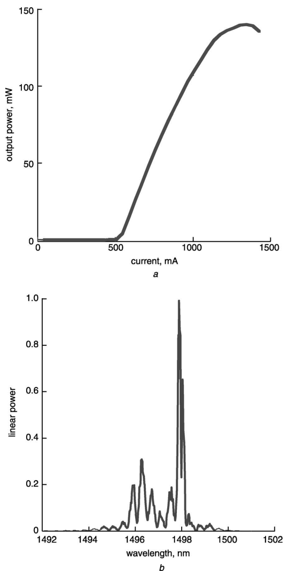
Fig. 9 Light output power and emission spectra of 20- \mu\text{m} -wide \times 2450- \mu\text{m} -long ridge waveguide edge-emitting laser for CW operation at room temperature
