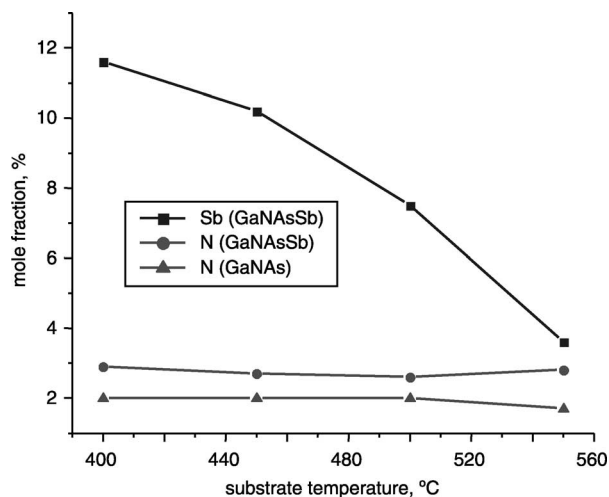
Fig. 5 SIMS results of N and Sb for GaNAs and GaNAsSb as a function of substrate temperature
