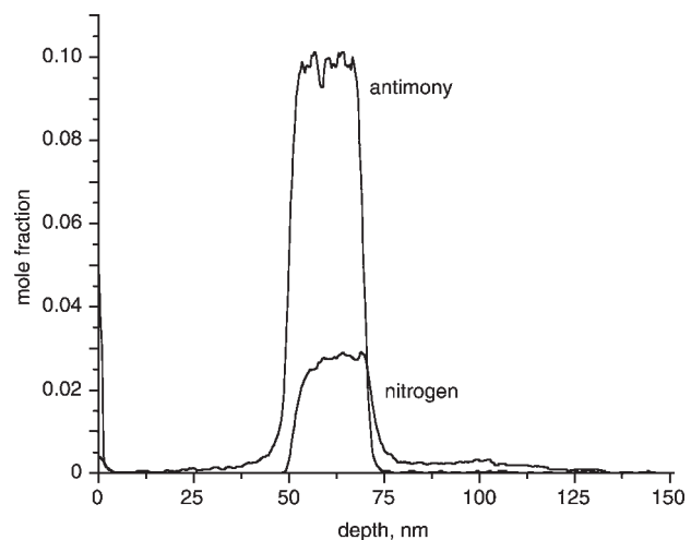
Fig. 4 Nitrogen and antimony SIMS profiles of \text{GaN}_{0.029}\text{As}_{0.873}\text{Sb}_{0.098} sample illustrating both the incorporation and surface accumulation nature of Sb
