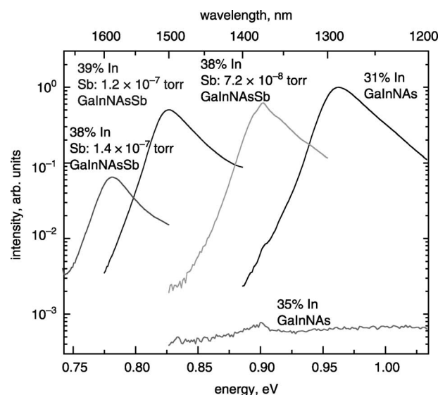
Fig. 3 Photoluminescence of GaInNAs(Sb) comparing the best 1.3\ \mu\text{m} material grown without Sb and the dramatic improvement in PL at even longer wavelengths by adding Sb
