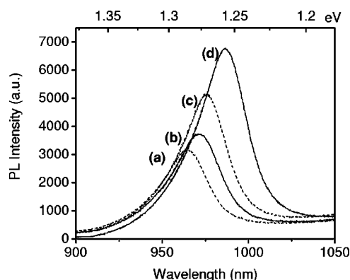
FIG. 6. PL spectra of the GaNAs(Sb) samples showing a redshift and increase in intensity with increasing antimony flux. (a) \text{GaN}_{0.0063}\text{As}_{0.9937} , (b) \text{GaN}_{0.0071}\text{As}_{0.9869}\text{Sb}_{0.006} , (c) \text{GaN}_{0.008}\text{As}_{0.978}\text{Sb}_{0.014} , and (d) \text{GaN}_{0.0091}\text{As}_{0.9709}\text{Sb}_{0.02} .
