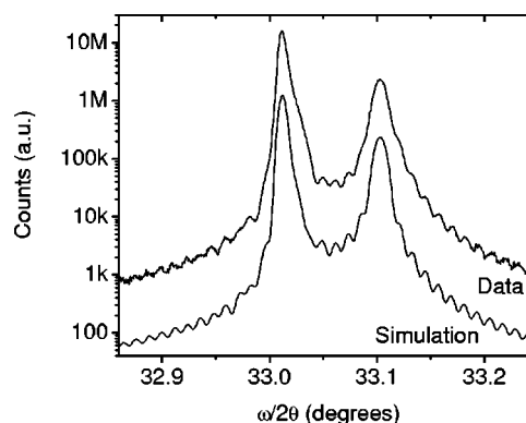
FIG. 2. (004) \omega/2\theta HRXRD spectrum of the \text{GaN}_{0.0063}\text{As}_{0.9937} sample with its corresponding simulated spectrum.
