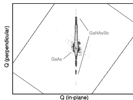
FIG. 7. Reciprocal space map of the \text{GaN}_{0.029}\text{As}_{0.873}\text{Sb}_{0.098} sample grown at a high temperature (575 ^{\circ}\text{C} ). No in-plane components from the QW are seen in the diffraction pattern.
