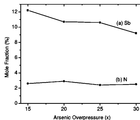
FIG. 5. SIMS results from the arsenic overpressure study. (a) Antimony composition and (b) nitrogen profile.
