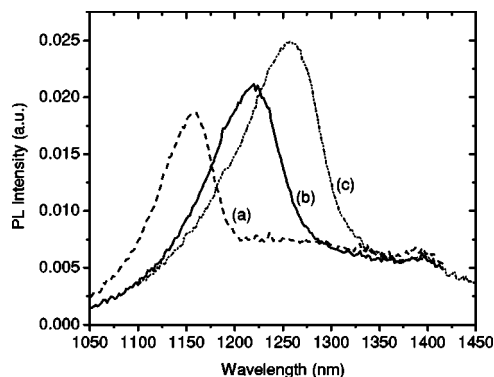
FIG. 9. PL spectra from the \text{GaN}_{0.029}\text{As}_{0.873}\text{Sb}_{0.098} sample grown at different substrate temperatures. (a) +150 °C (575 °C), (b) +100 °C (525 °C), and (c) +50 °C (475 °C). The small peak at 1400 nm is the water present in the testing environment.
