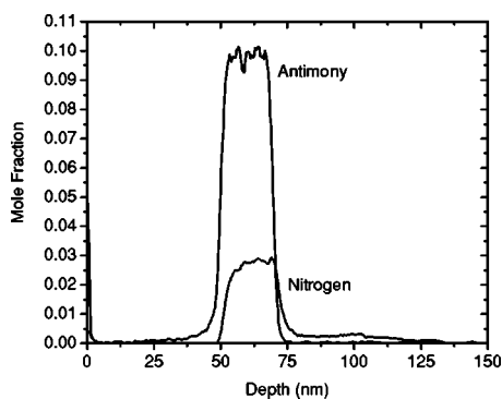
FIG. 3. SIMS depth profile of antimony and nitrogen for a \text{GaN}_{0.029}\text{As}_{0.873}\text{Sb}_{0.098} sample.
