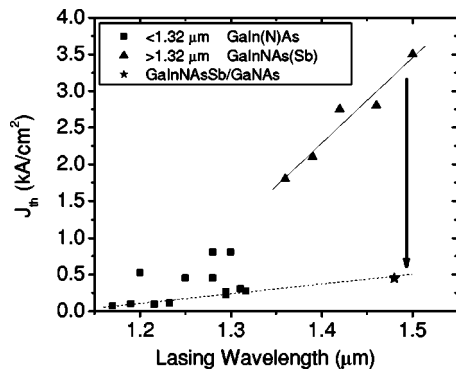
FIG. 10. Compilation of the long-wavelength edge-emitting GaAs lasers threshold current-lasing densities vs wavelength from literature. Utilizing the GaNAs barriers has allowed for the greatly reduced threshold current densities, as shown by the star data point.
