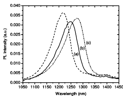
FIG. 6. PL spectra from the \text{GaN}_{0.029}\text{As}_{0.873}\text{Sb}_{0.098} sample grown at different arsenic-to-gallium overpressures. (a) 30\times , (b) 25\times , and (c) 15\times .
