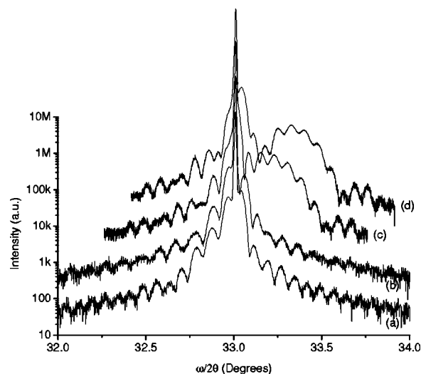
FIG. 2. (004) \omega/2\theta XRD spectra showing the amount of strain in the samples. (a) \text{GaN}_{0.029}\text{As}_{0.873}\text{Sb}_{0.098} , (b) \text{GaN}_{0.034}\text{As}_{0.867}\text{Sb}_{0.099} , (c) \text{GaN}_{0.019}\text{As}_{0.981} , and (d) \text{GaN}_{0.027}\text{As}_{0.973} . (a) and (c) are grown under the 1.3 \mu\text{m} device growth conditions, whereas (b) and (d) are grown under the 1.55 \mu\text{m} device growth conditions.
