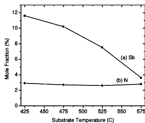
FIG. 8. SIMS results from the substrate temperature study. (a) Antimony composition and (b) nitrogen profile.
