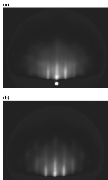
FIG. 1. RHEED pictures showing the streaky patterns from (a) GaNAs and the spotty patterns from (b) GaNAsSb.
