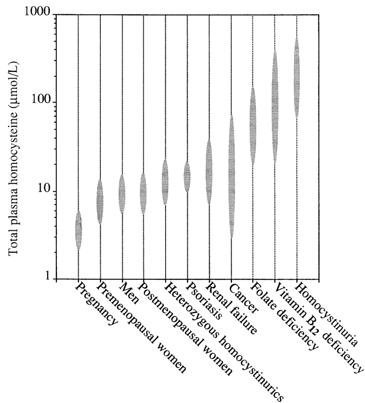
Fig. 7. Conditions causing elevated plasma homocysteine.
