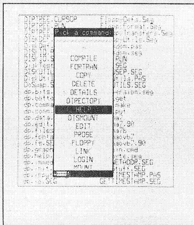
Figure 6. A pop-up menu over a background of a directory listing. The command HELP will be executed.
