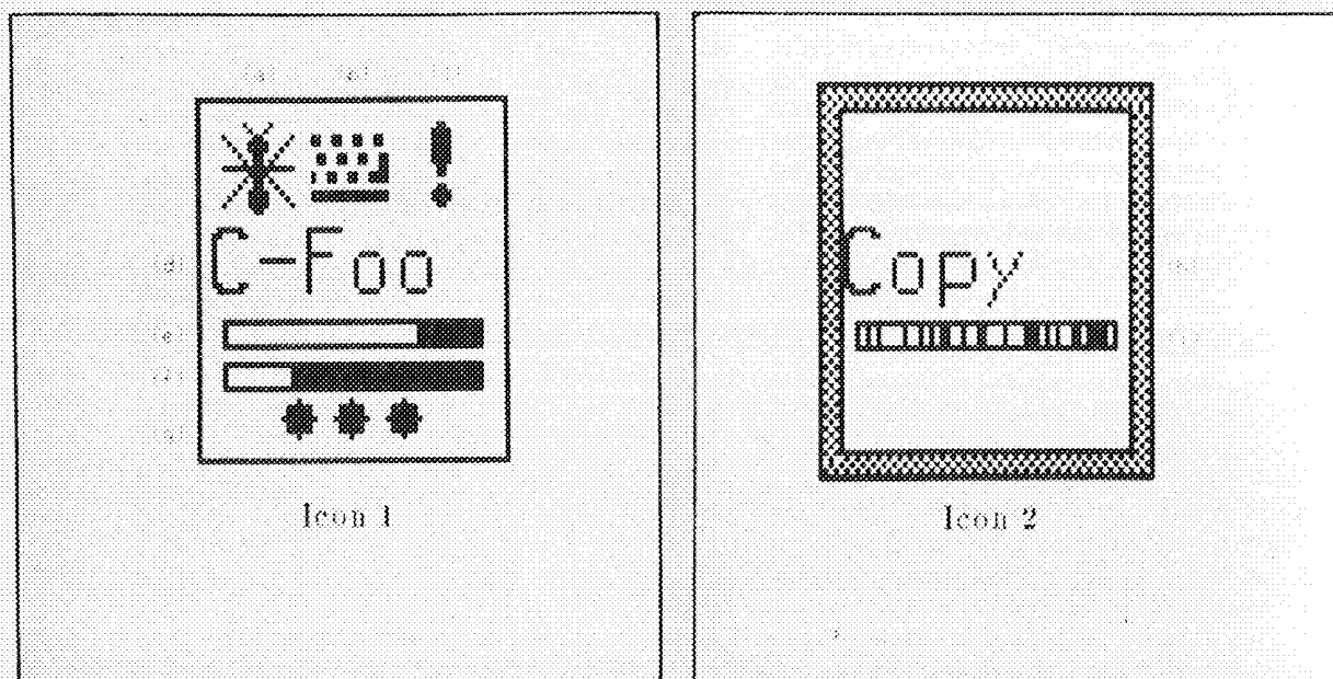
Figure 4. Expanded view of icons in Sapphire. In icon 1, (a) is the error signal, (b) shows that the process is waiting for user input, and (c) is the application-defined attention signal. (e) and (f) are two "percent-done progress bars," and (g) shows that the associated window is offscreen. Icon 2 corresponds to the Listener (the border is shown in gray), and it has its first progress bar (i) showing random progress. The process associated with icon 2 is "Copy" (h). In icon 1, the compiler has shown (d) the name of the program being processed ("C" for compiler, and "Foo" is the name of the program).
