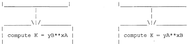
Figure 3. The Diffie/Hellman Key Exchange
