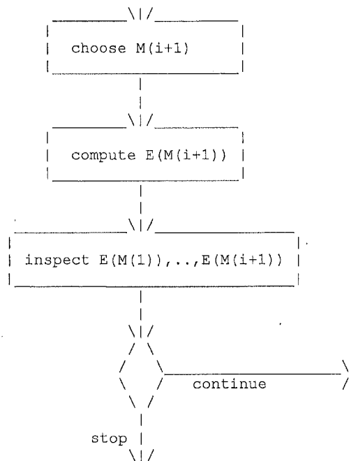
Figure 1. Adaptive Chosen Plaintext Attack
