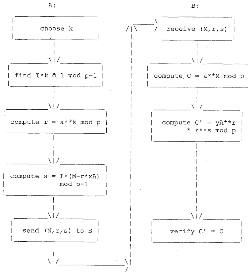
Figure 7. The ElGamal Signature Algorithm
