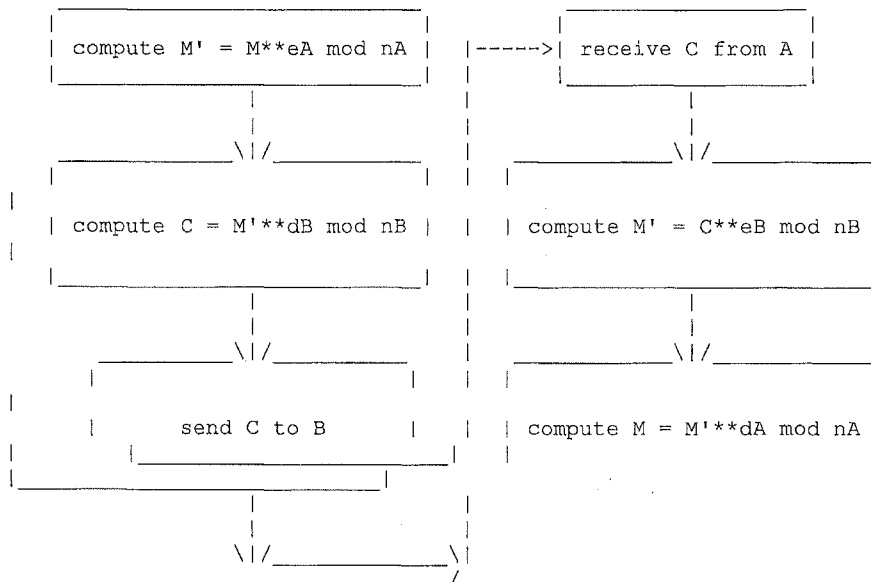
Figure 6. Using RSA for Authenticity and Secrecy
