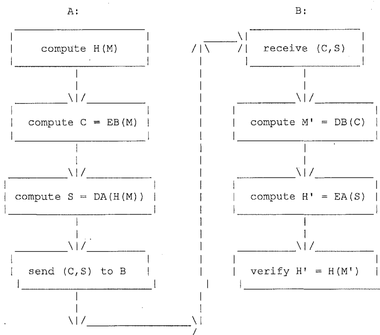
Figure 2. Using Public-Key for Secrecy and Authenticity
