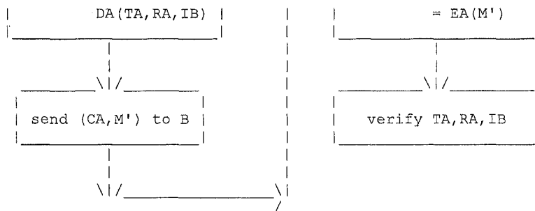
Figure 8. One-Way Authentication Protocol
