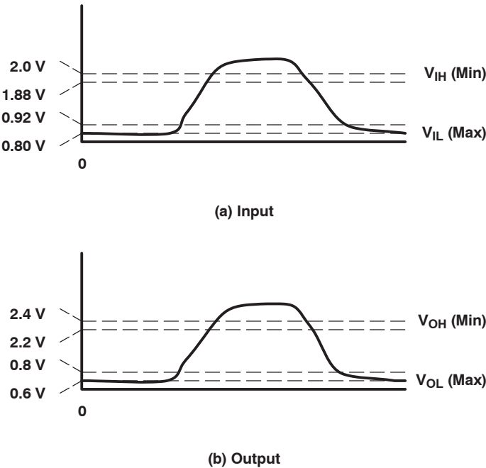
Figure 4. Voltage Reference Levels
