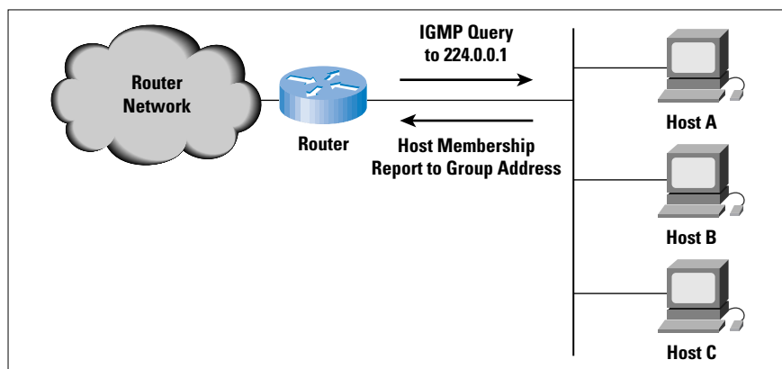
Figure 2: IGMPv1 Dialog
