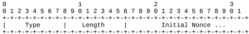
Figure 1: ECP 3DESE Configuration Option
