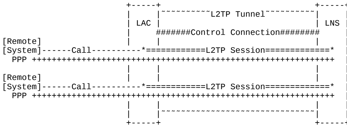
Figure 5.1 Tunneling PPP
