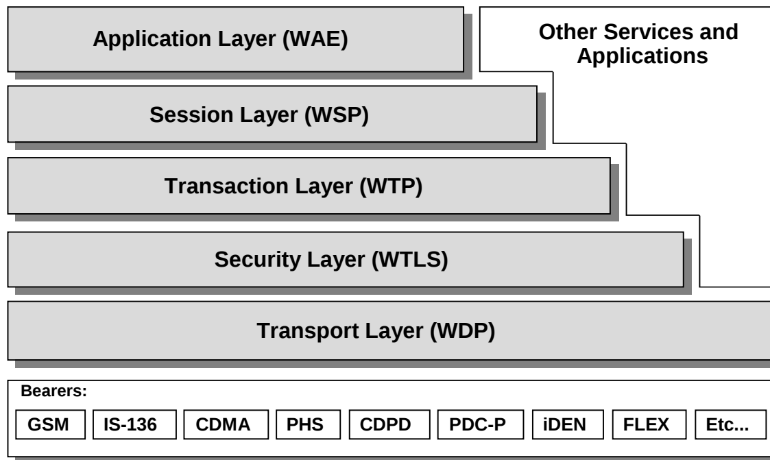
Figure 4. WAP Architecture
