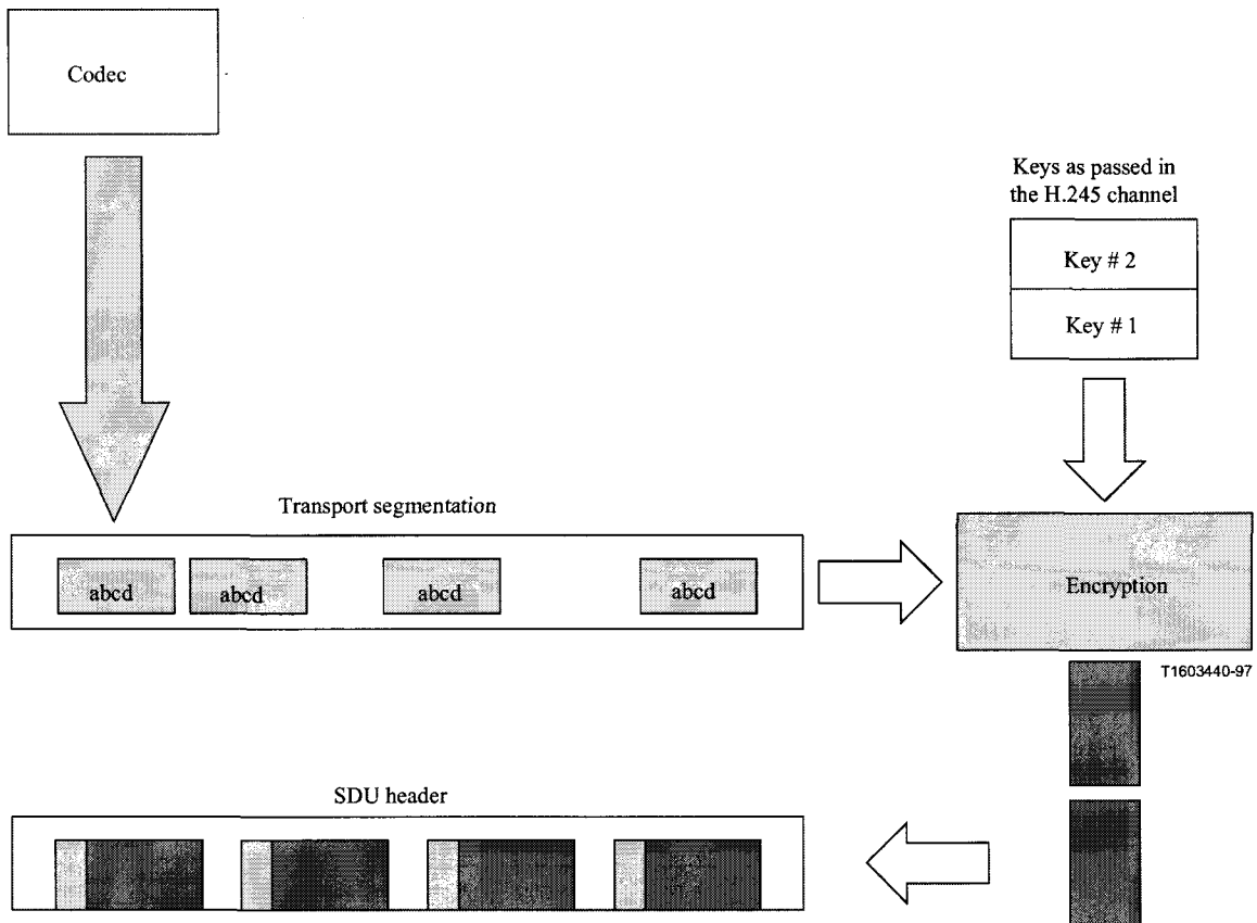
Figure 5/H.235 – Encryption of media
