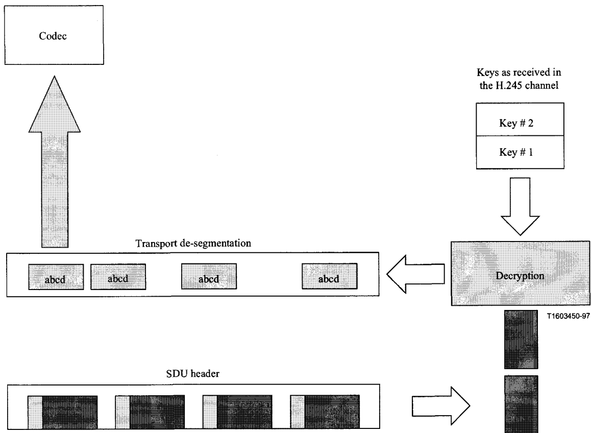
Figure 6/H.235 – Decryption of media
