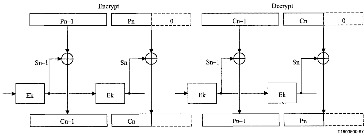
Figure I.4/H.235 – Zero padding in OFB mode
