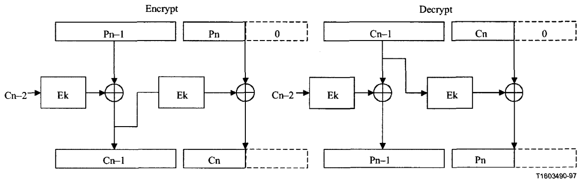
Figure I.3/H.235 – Zero padding in CFB mode
