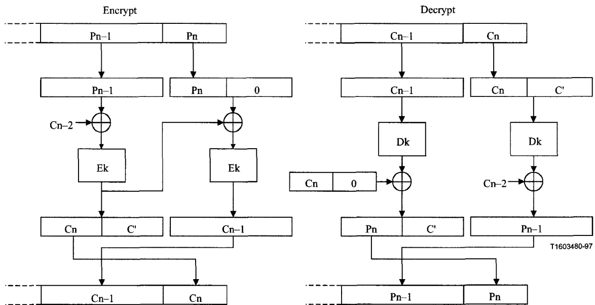
Figure I.2/H.235 – Ciphertext stealing in CBC mode
