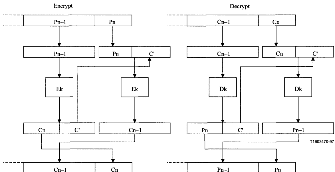
Figure I.1/H.235 – Ciphertext stealing in ECB mode
