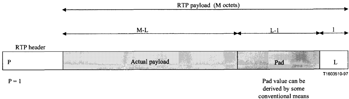
Figure I.5/H.235 – Padding as prescribed by RTP
