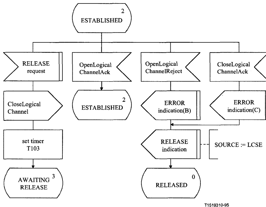
Figure 18.iii/H.245 – Outgoing B-LCSE SDL (continued)
