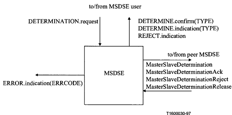
Figure 3/H.245 – Primitives and messages in the MSDSE
