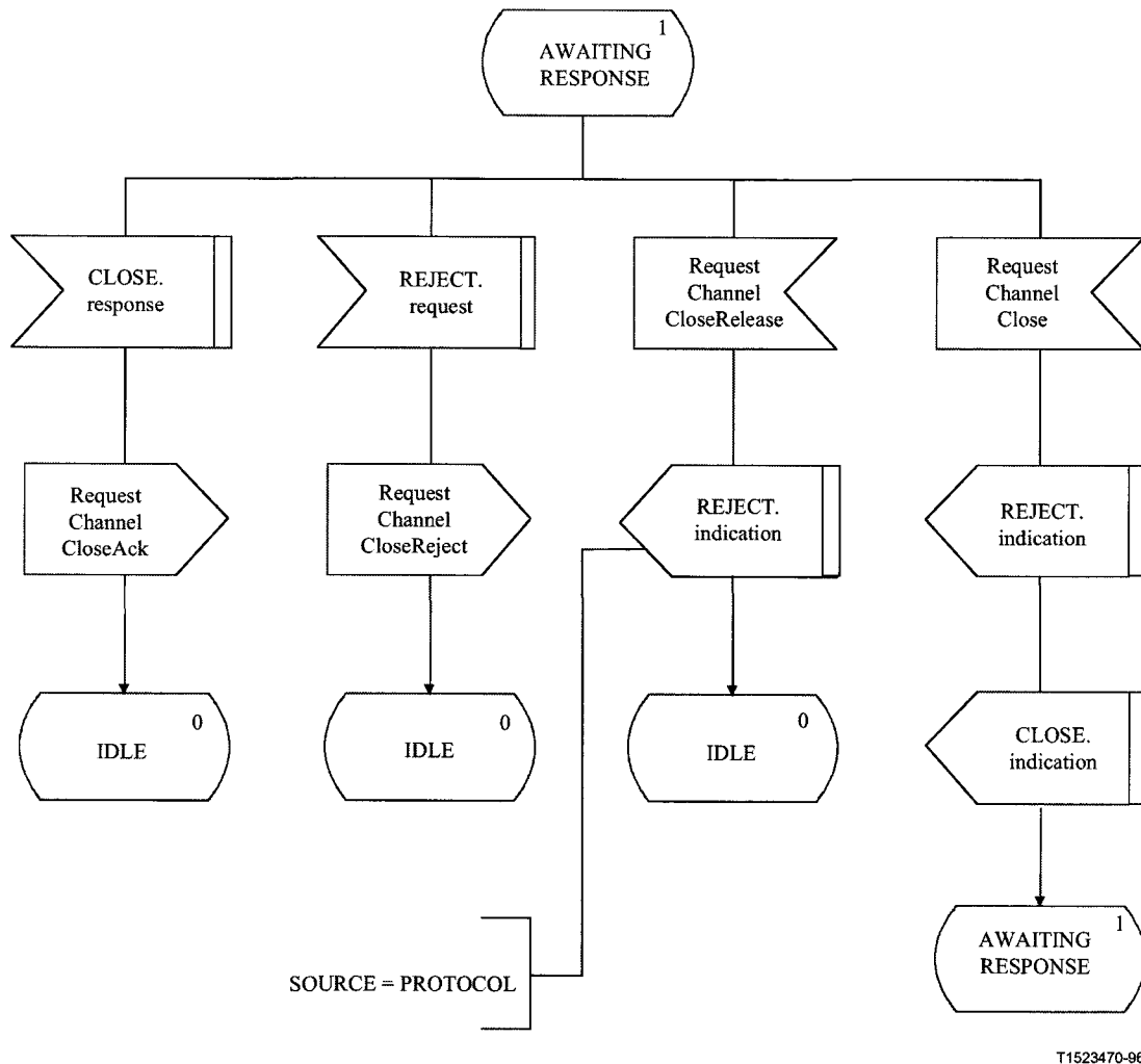
Figure 24.ii/H.245 – Incoming CLCSE SDL (concluded)
