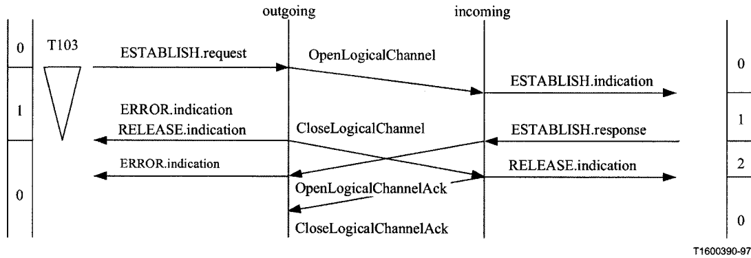
Figure II.9-6/H.245 – Bi-directional logical channel establishment request with expiry of timer T103 at the outgoing side. Timer T103 at the outgoing side has expired after transmission of the OpenLogicalChannelAck message at the incoming B-LCSE, but before reception of the OpenLogicalChannelAck message at the outgoing B-LCSE
