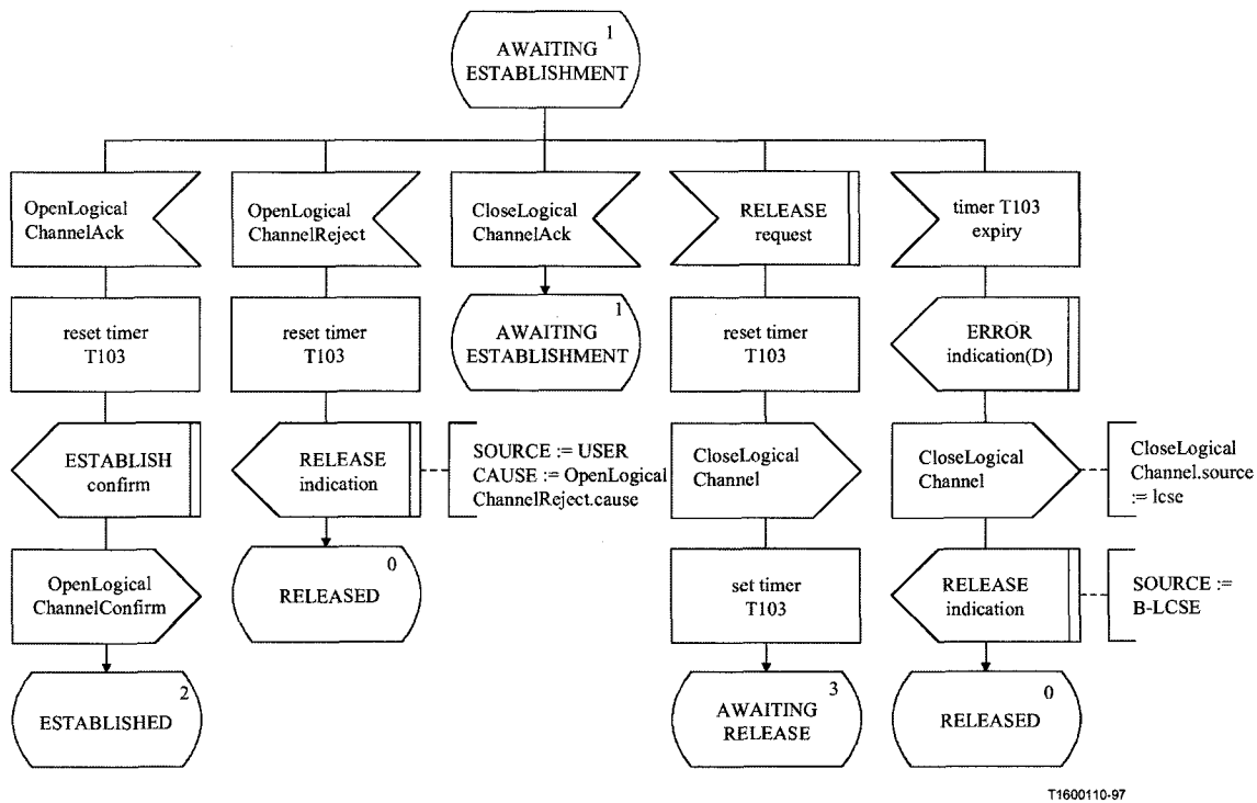
Figure 18.ii/H.245 – Outgoing B-LCSE SDL (continued)
