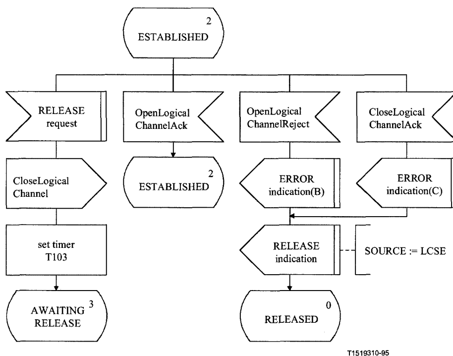
Figure 13.iii/H.245 – Outgoing LCSE SDL (continued)
