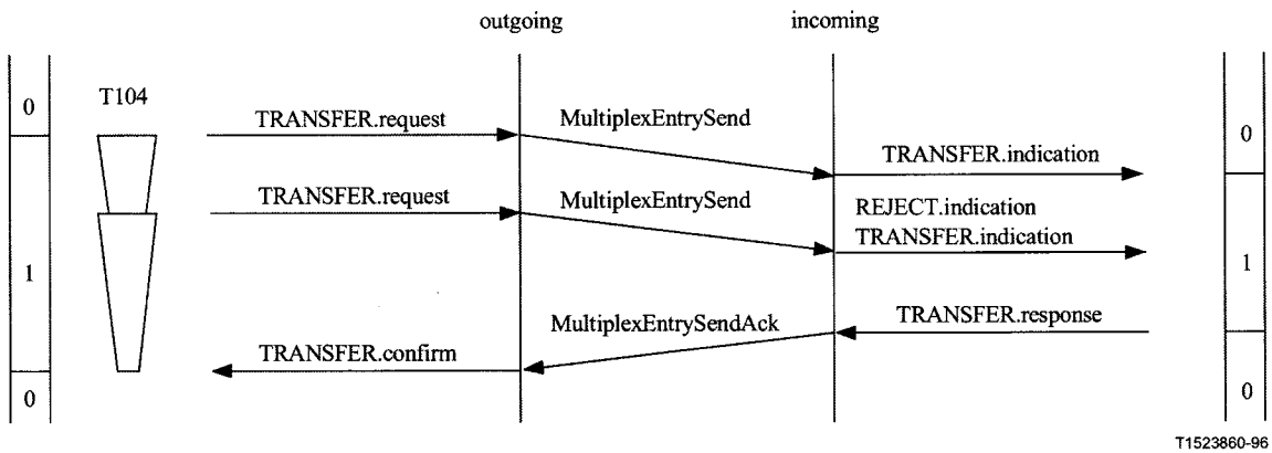
Figure II.6-3/H.245 – Multiplex table send request with a second multiplex table send request before acknowledgement of the first request. The first request was unsuccessful
