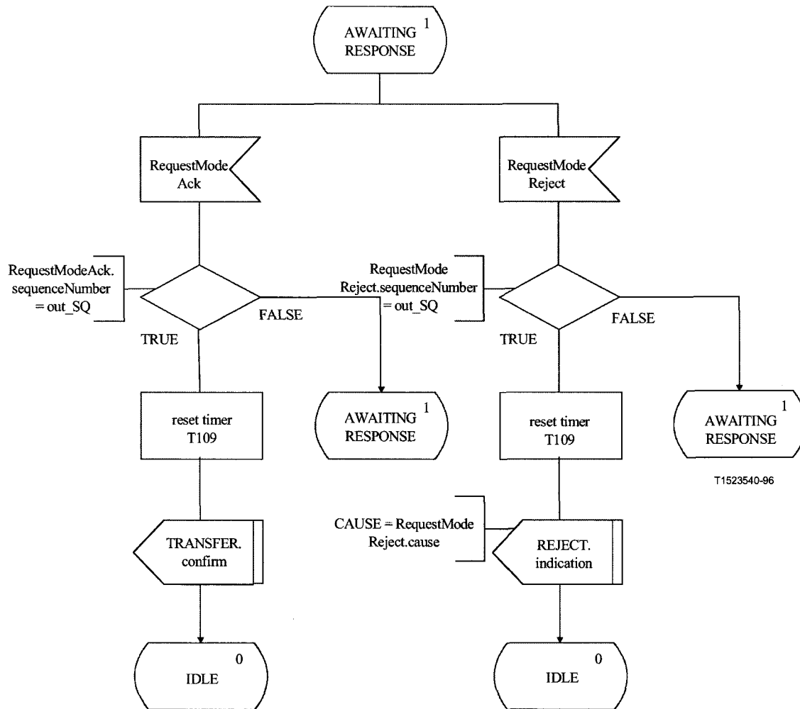
Figure 38.ii/H.245 – Outgoing MRSE SDL (continued)
