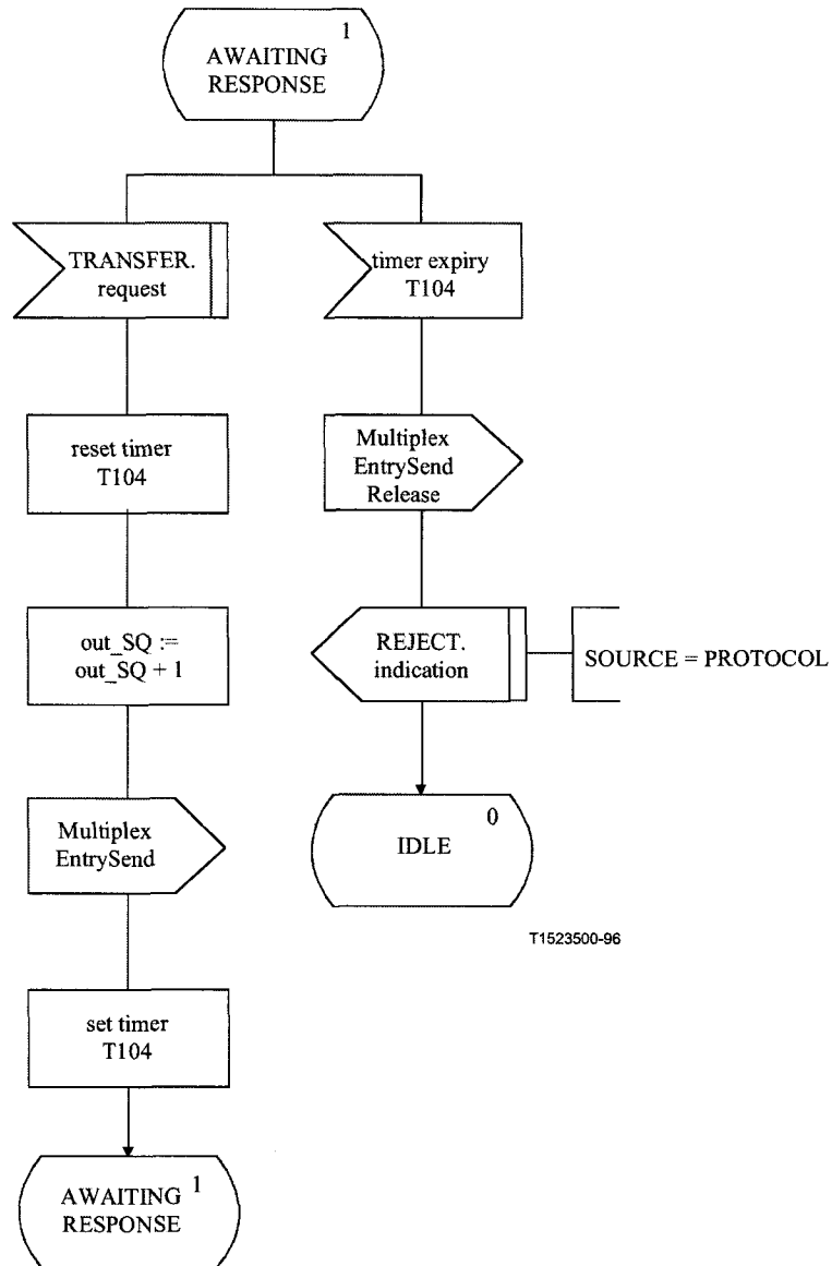
Figure 28.iii/H.245 – Outgoing MTSE SDL (concluded)
