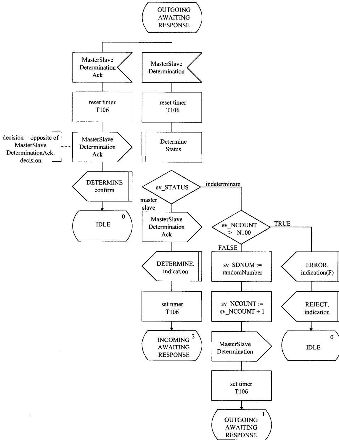
Figure 4.ii/H.245 – MSDSE SDL (continued)
