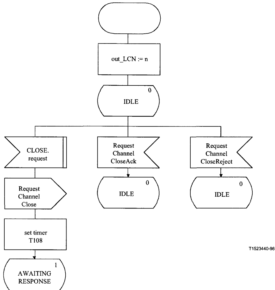
Figure 23.i/H.245 – Outgoing CLCSE SDL
