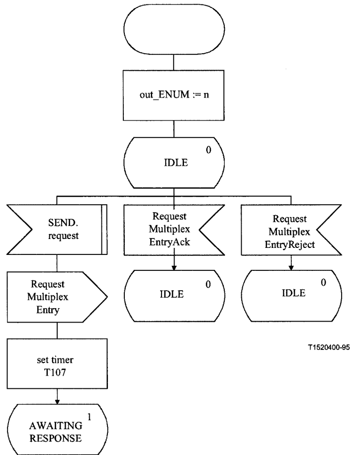
Figure 33.i/H.245 – Outgoing RMESE SDL
