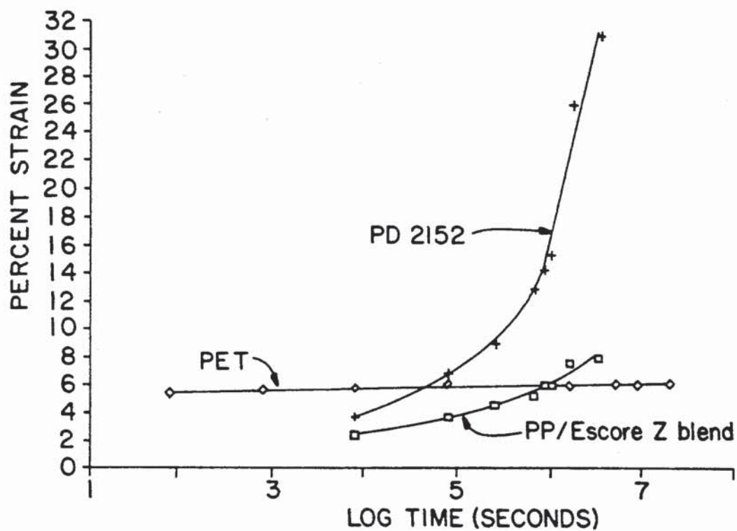
FIG. 1A CREEP RESISTANCE - 20% LOADING
