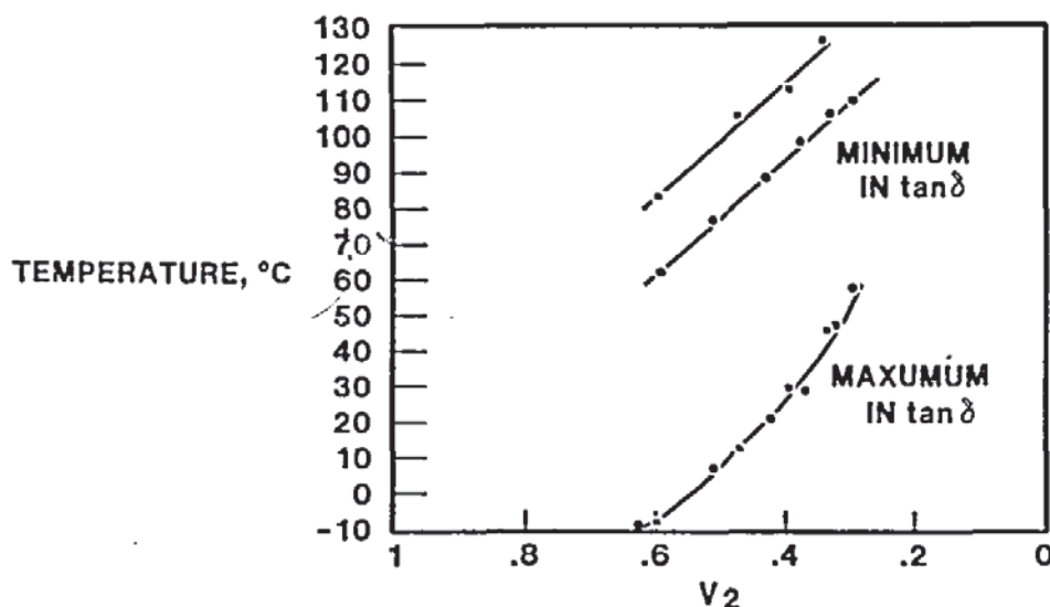
FIGURE 7 Positions of maxima and minima in loss tangent (35 Hz). Solprene 418 with Foral 85 (●) and Wingtack 95 (■).
