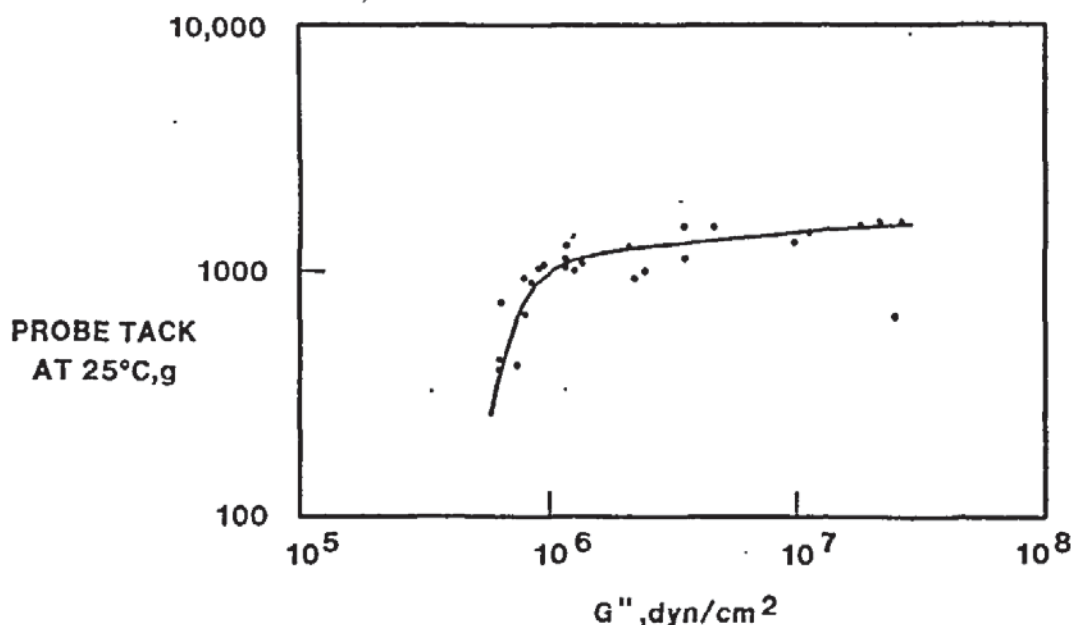
FIGURE 8 Tack vs. 35 Hz loss modulus.
