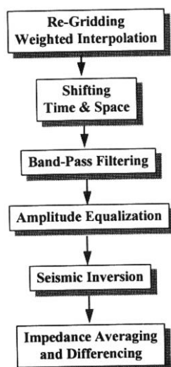
Figure 3. Differencing Methodology
