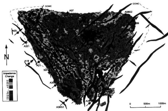
Figure 4. Change in Fulmar reservoir impedance between 1977 and 1992.
