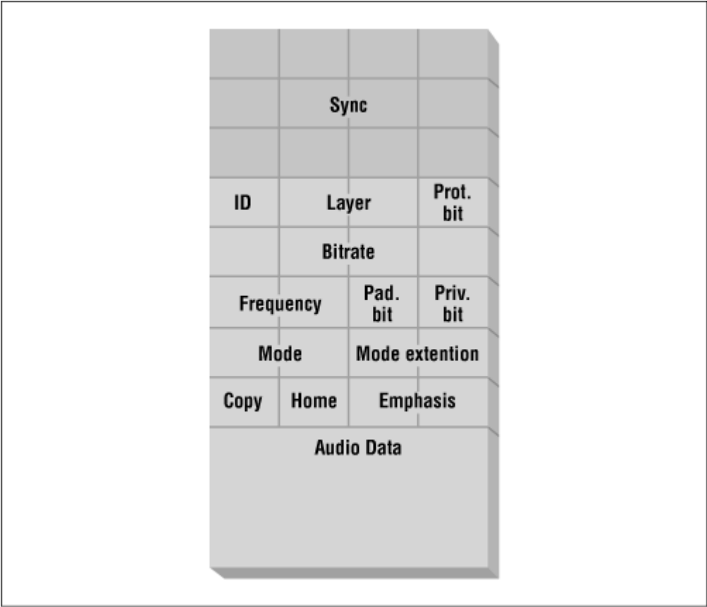
Figure 2.5. The MP3 frame header represented visually
