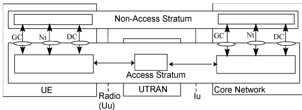
Figure 1: Assumed UMTS Architecture
