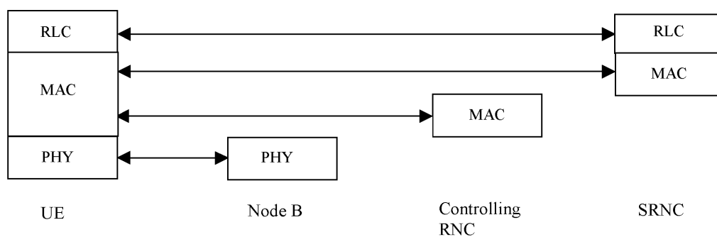
Figure 15: Protocol Termination for RACH/FACH, user plane
