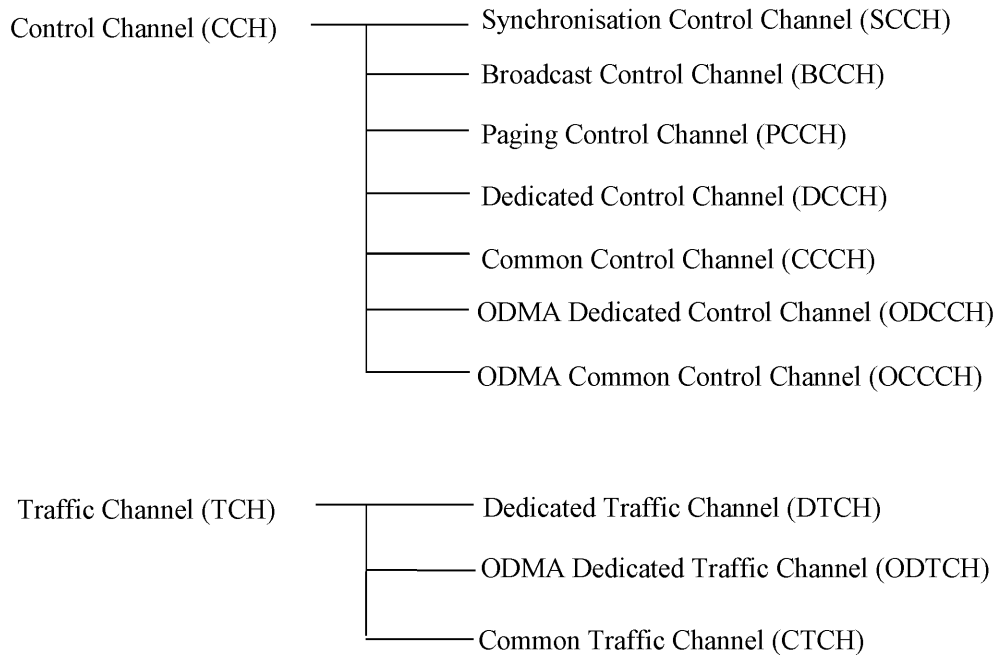
Figure 3: Logical channel structure
