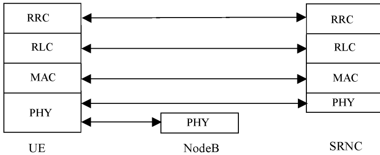
Figure 12: Protocol Termination for DCH, control plane
