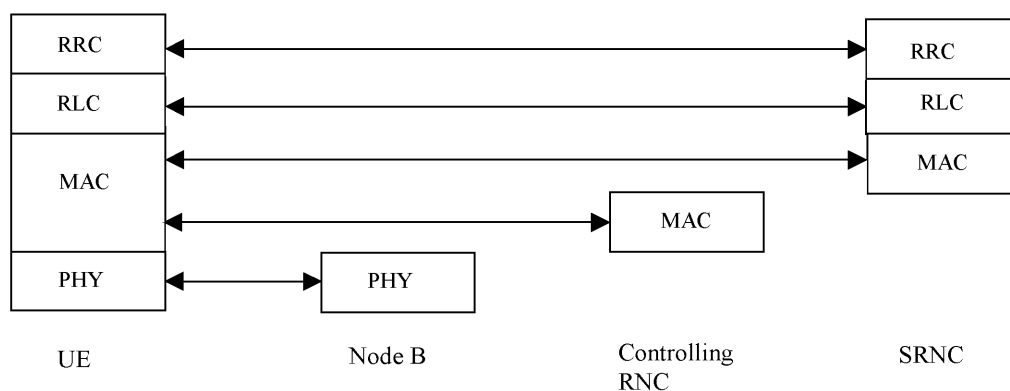
Figure 14: Protocol Termination for RACH/FACH, control plane
