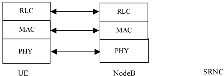
Figure 26: Protocol Termination for DCH, user plane
