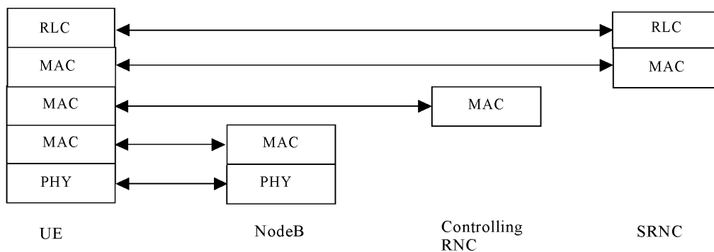
Figure 28: Protocol Termination for RACH/FACH, user plane
