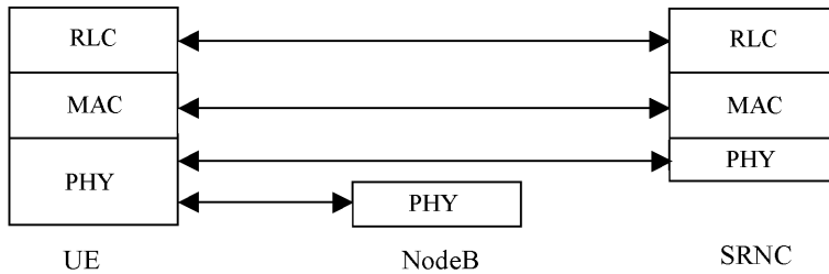
Figure 13: Protocol Termination for DCH, user plane
