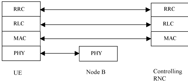
Figure 20: Protocol termination for PCH
