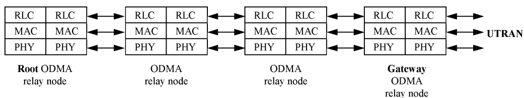
Figure 22: Protocol Termination for the ODCH in the User Plane
