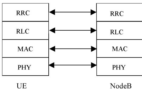
Figure 19: Protocol termination for BCH.
