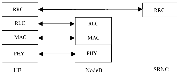
Figure 25: Protocol Termination for DCH, control plane
