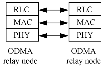
Figure 24: Protocol Termination for ORACH user plane
