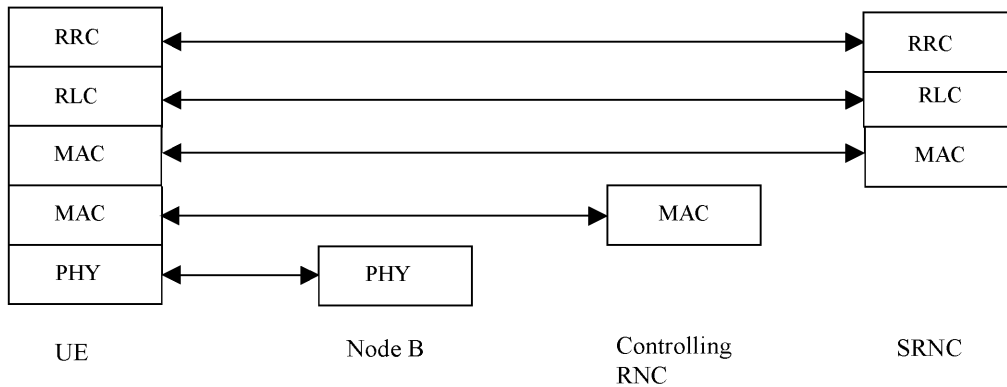
Figure 17: Protocol termination points for DSCH, control plane.
