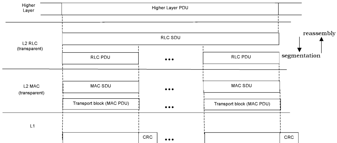
Figure 7: Data flow for transparent RLC and MAC
