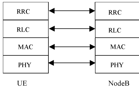
Figure 29: Protocol termination for PCH
