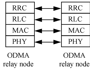
Figure 23: Protocol Termination for ORACH control plane
