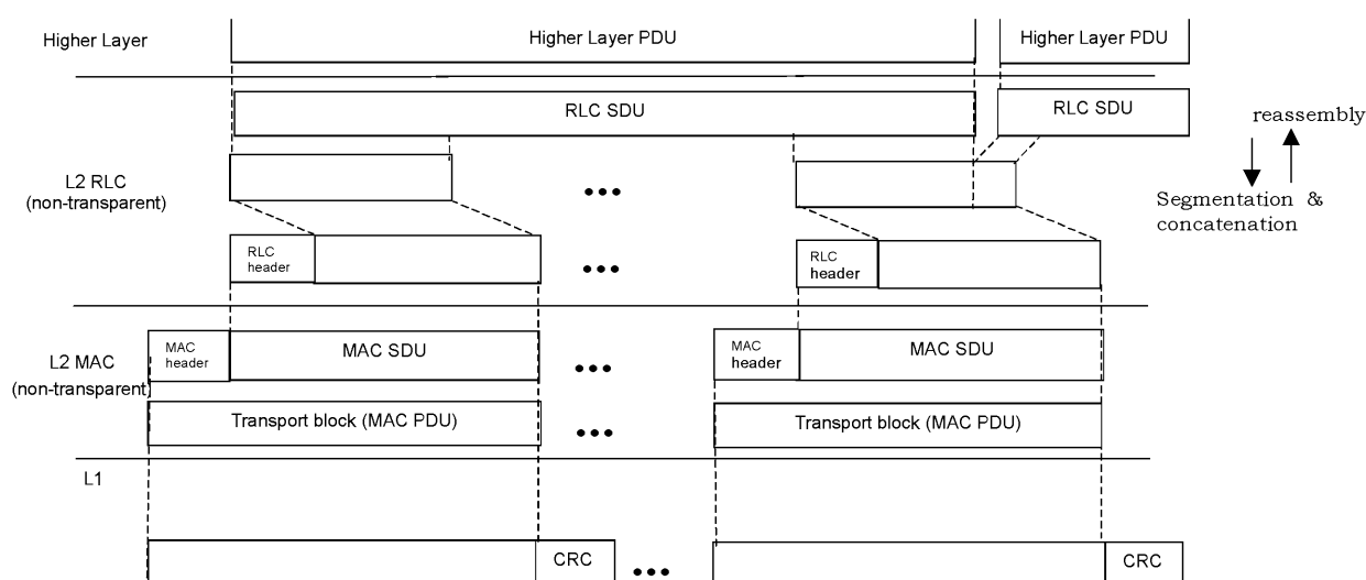
Figure 10: Data flow for non-transparent RLC and MAC
