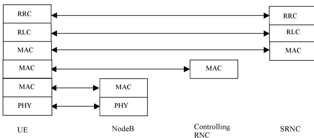
Figure 27: Protocol Termination for RACH/FACH, control plane
