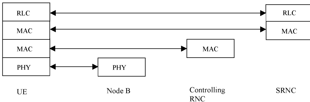
Figure 18: Protocol termination points for DSCH, user plane.
