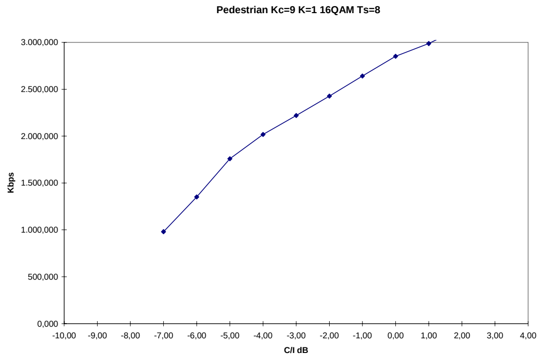
Figure 1-22 UDD 2048 kbit/s UL and DL Pedestrian 3 km/h, 1 User per TS, 9 Codes and 8 TS per user, 16QAM, code rates 1, 2/3, 1/2, 1/3 and 1/4
