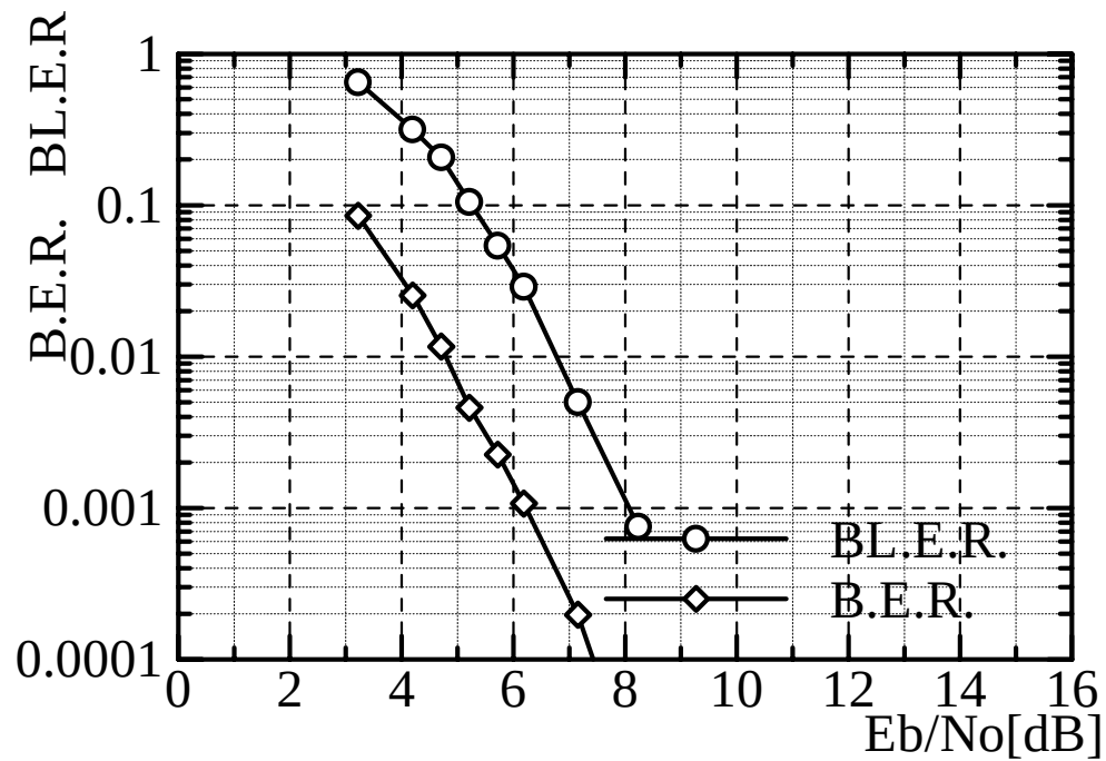
Figure 32 E_b/N_0 vs BL.E.R. ( Mode A, Vehicular)
