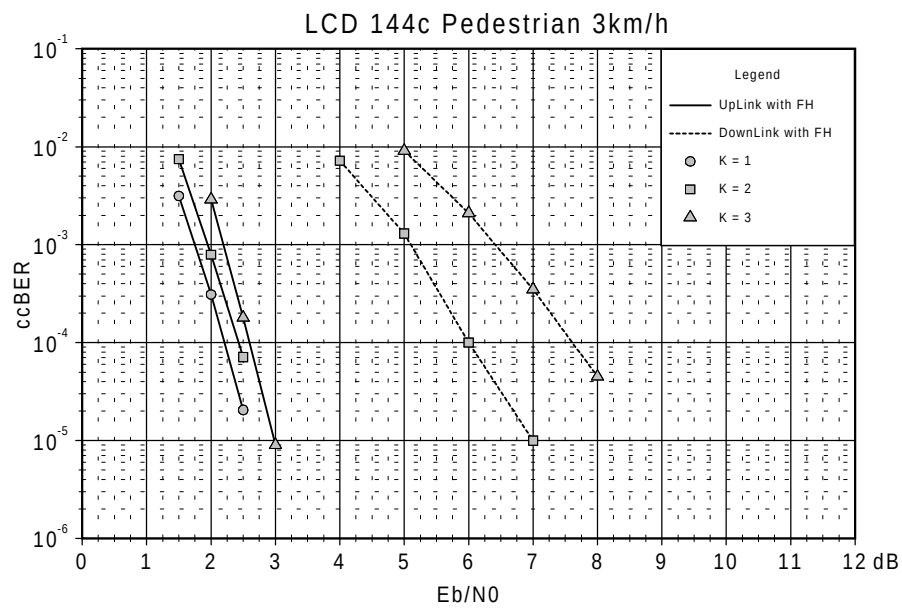
Figure 1-9 LCD 144 c UL and DL Pedestrian 3 km/h, 1, 2 and 3 Users per TS, 3 Codes and 4 TS per user
