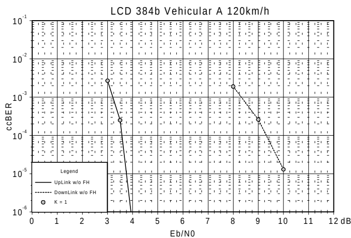
Figure 1-12 LCD 384 b UL and DL Vehicular 120 km/h, 1 User per TS, 9 Codes and 3 TS per user
