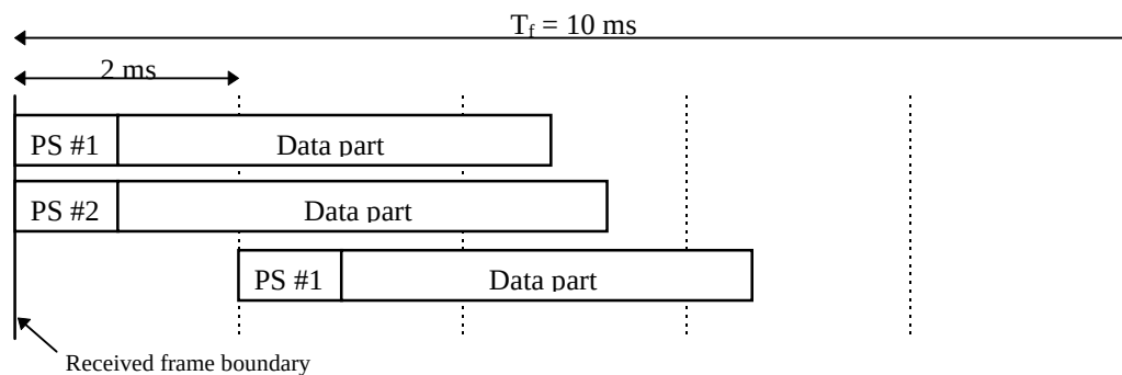
Figure 21 Possible transmission timing for parallel Random-Access attempts
