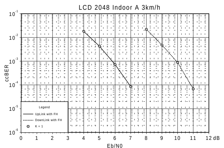
Figure 1-15 LCD 2048 UL and DL Indoor 3 km/h, 1 User per TS, 9 Codes and 8 TS per user
