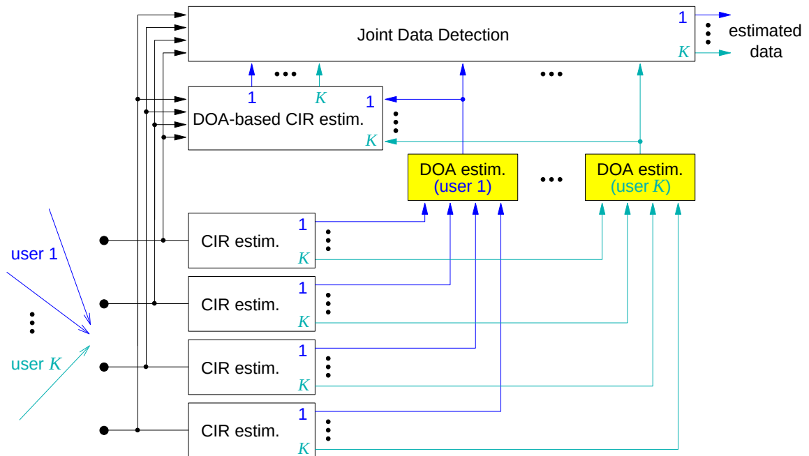
Figure 2-2 Joint detection receiver structure for K simultaneously active users using an adaptive antenna array and direction of arrival (DOA)-based channel impulse response (CIR) estimation. In the depicted example, an antenna array with K_a = 4 antenna elements is used.
