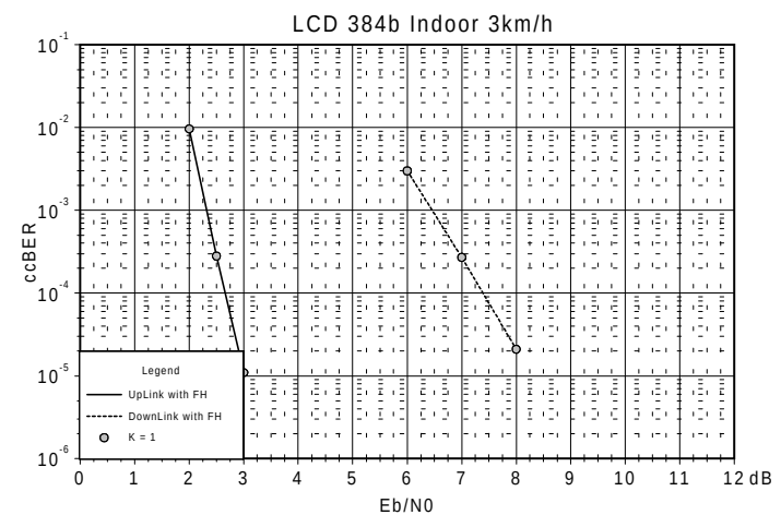
Figure 1-13 LCD 384 b UL and DL Indoor 3 km/h, 1 User per TS, 9 Codes and 3 TS per user
