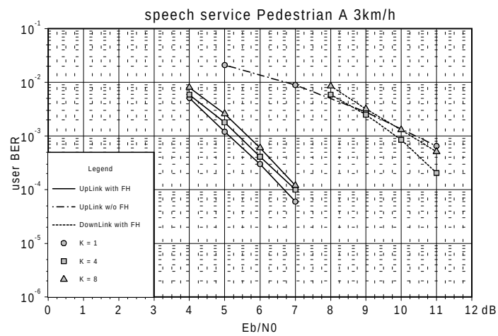
Figure 1-3 Speech UL and DL Pedestrian A 3 km/h, 1, 4 and 8 Users per TS, 1 Code and 1 TS per user
