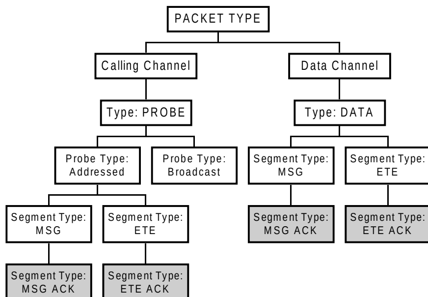
Figure 13 ODMA Packet Structures
