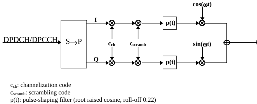
Figure 3 Spreading/modulation for downlink dedicated physical channels
