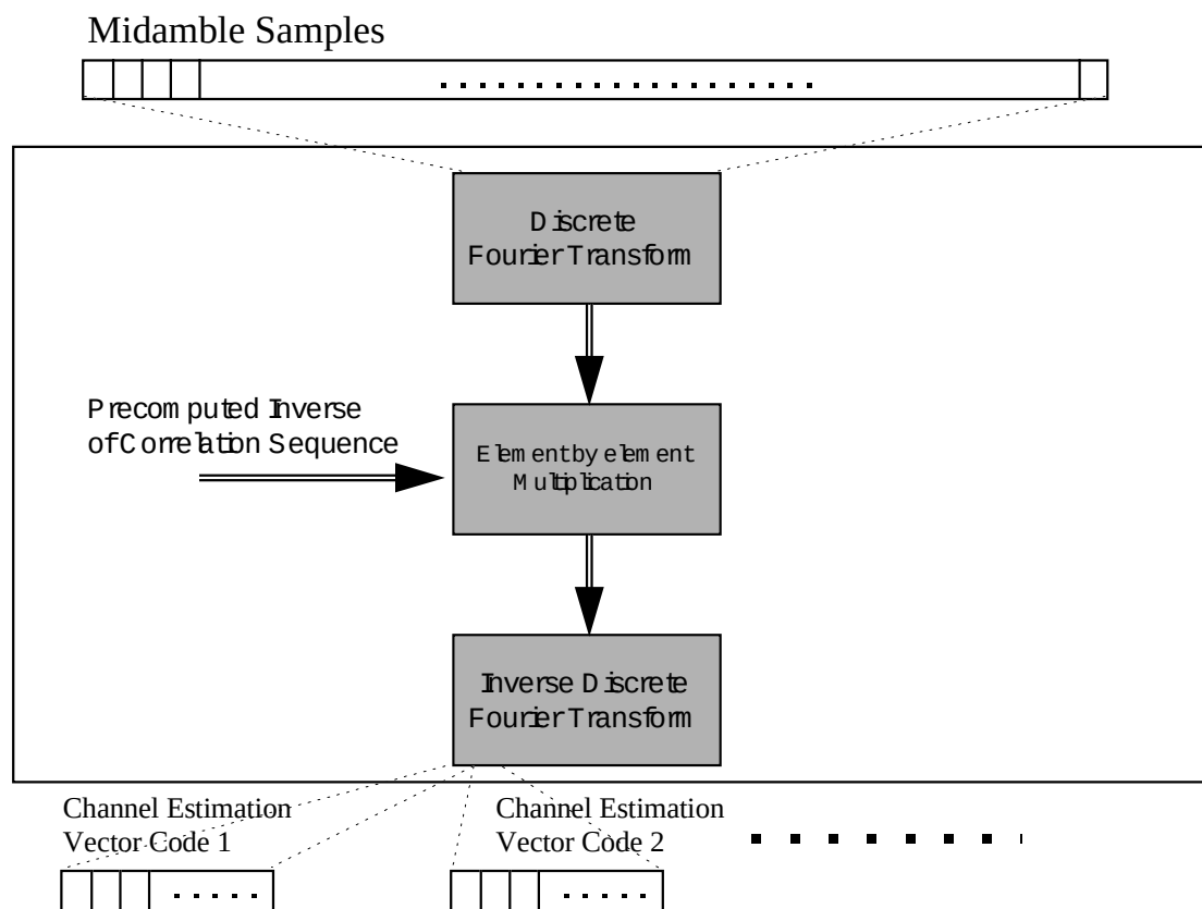
Figure 24 WB-TDMA/CDMA Fast Correlator
