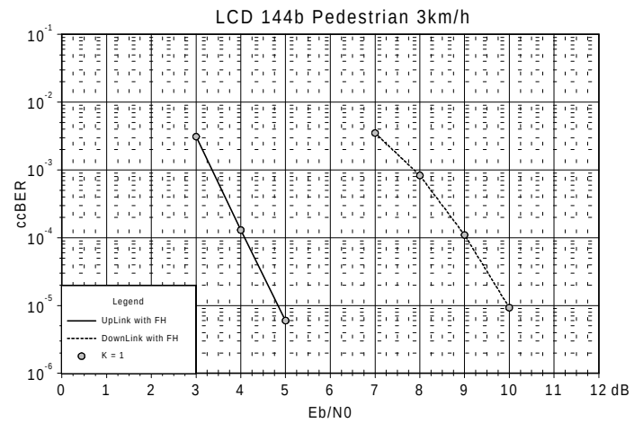
Figure 1-8 LCD 144 b UL and DL Pedestrian 3 km/h, 1 User per TS, 9 Codes and 1 TS per user
