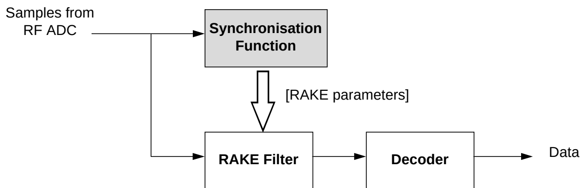
Figure 21 WCDMA Receiver
