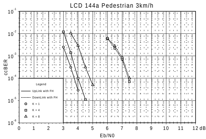
Figure 1-7 LCD 144 a UL and DL Pedestrian 3 km/h, 1, 4 and 8 Users per TS, 1 Code and 8 TS per user
