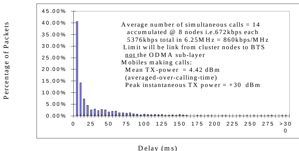
Figure 21 Packet Delay Distribution for Manhattan 3x3 Block LCD 384kbps Capacity
