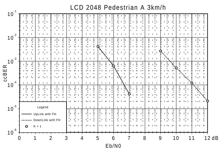
Figure 1-14 LCD 2048 UL and DL Pedestrian 3 km/h, 1 User per TS, 9 Codes and 8 TS per user
