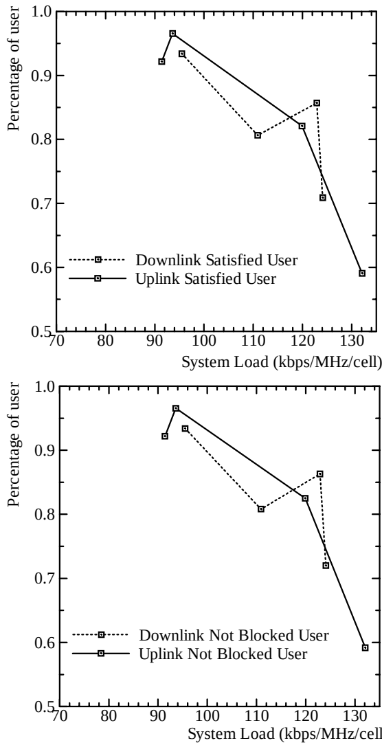
Figure 48 System Bandwidth 3.2 MHz
