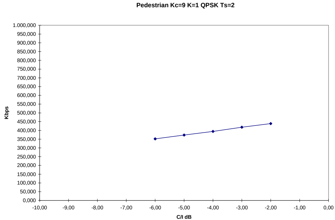
Figure 1-20 UDD 384 kbit/s UL and DL Pedestrian 3 km/h, 1 User per TS, 9 Codes and 2 TS per user, QPSK, code rates 1, 2/3, 1/2, 1/3 and 1/4
