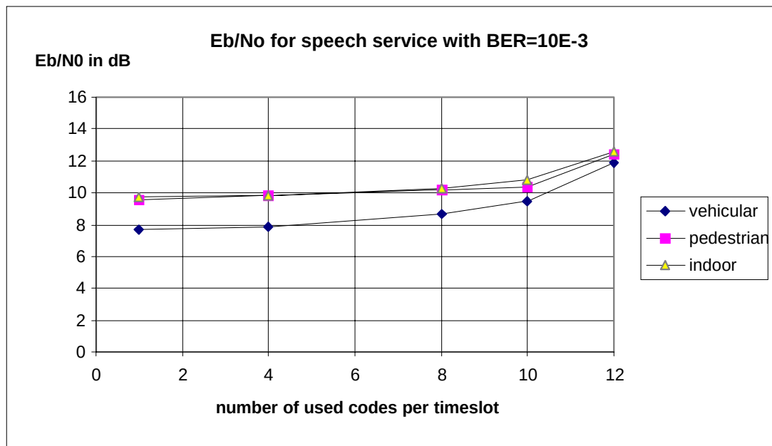
Figure 1-1. Dependence of the required values for E_b/N_0 for speech 8 kbit/s in order not to exceed a BER of 10^{-3} as a function of the number K of active users per time slot in the downlink for Indoor A, Pedestrian A and Vehicular A
