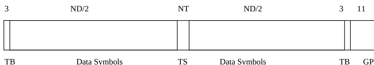
Figure 3-9 Structure of Flexible Burst
