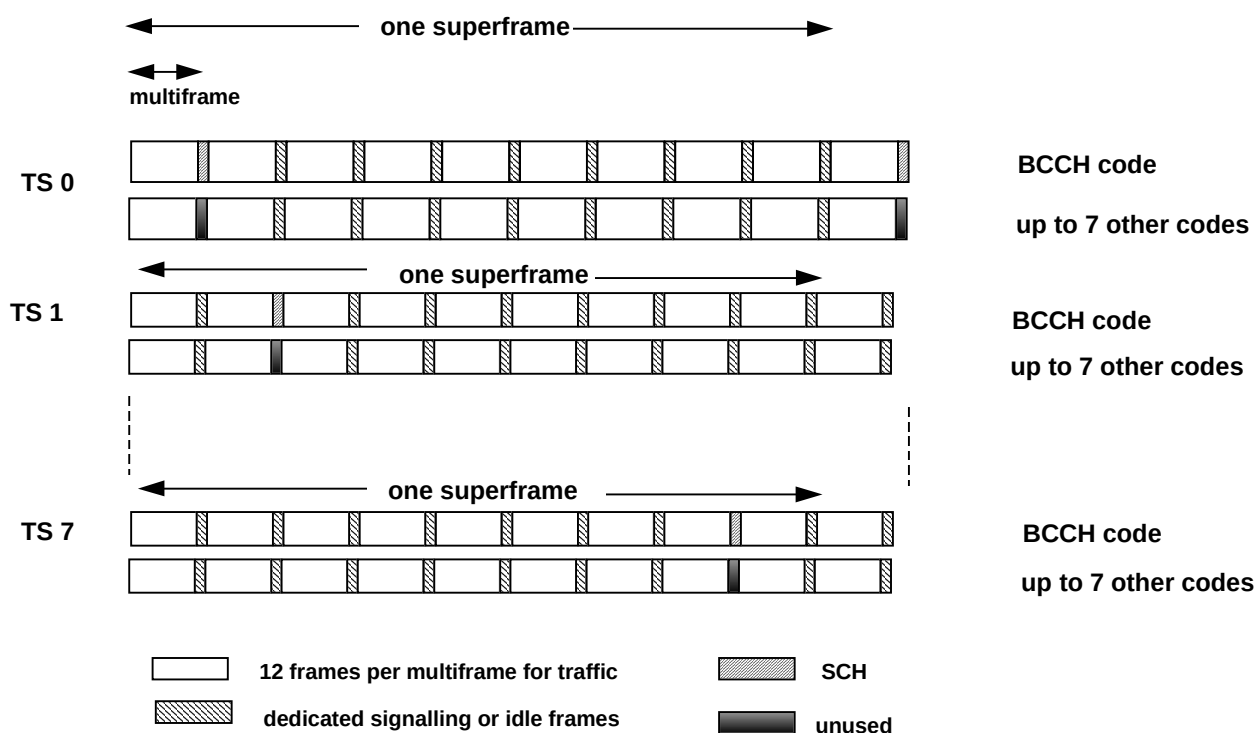
Figure 3-1: Mapping of the SCH channel
