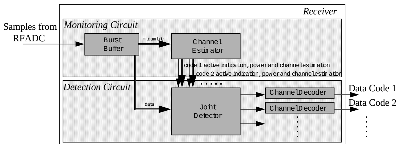
Figure 22 WB-TDMA/CDMA - ODMA Enabled Receiver
