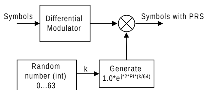
Figure 13: Random Phase Shift Technique
