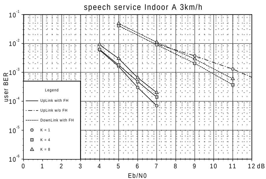
Figure 1-4 Speech UL and DL Indoor 3 km/h, 1, 4 and 8 Users per TS, 1 Code and 1 TS per user
