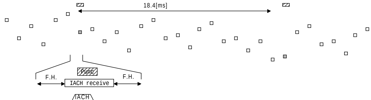
Figure 19 Puncturing Scheme (1 of 4 Time slot usage)
