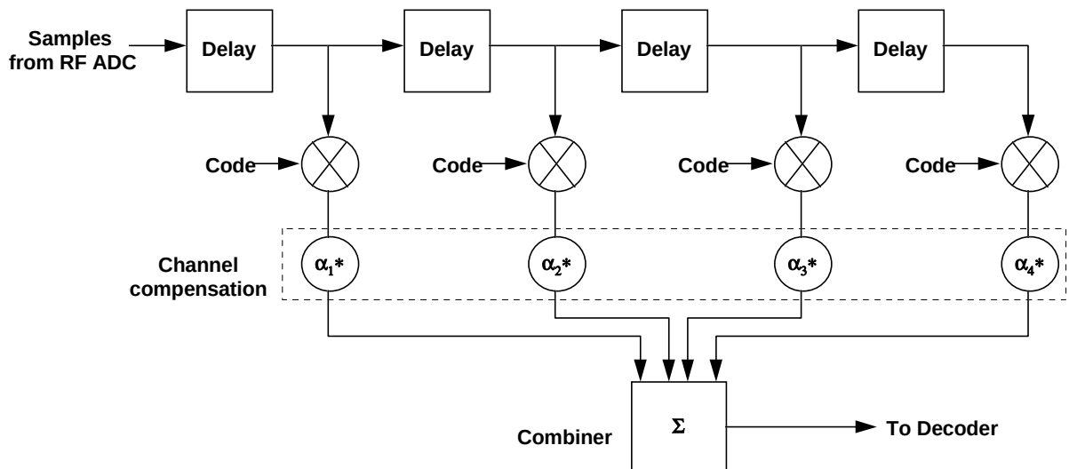
Figure 24 WCDMA Rake Receiver
