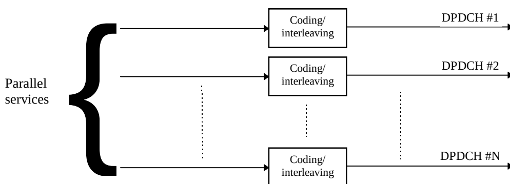
Figure 12 Alternative service multiplexing
