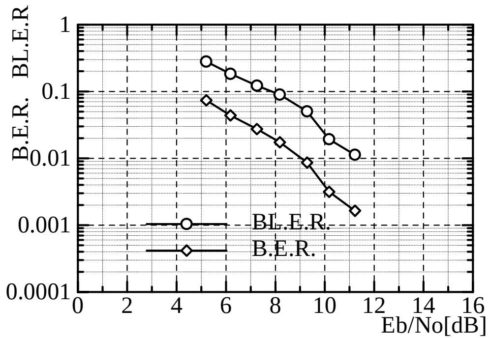
Figure 31 E_b/N_o vs BL.E.R. ( Mode A, Pedestrian)
