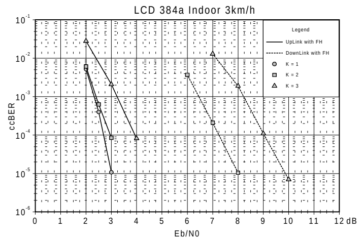
Figure 1-11 LCD 384 a UL and DL Indoor 3 km/h, 1, 2 and 3 Users per TS, 3 Codes and 8 TS per user
