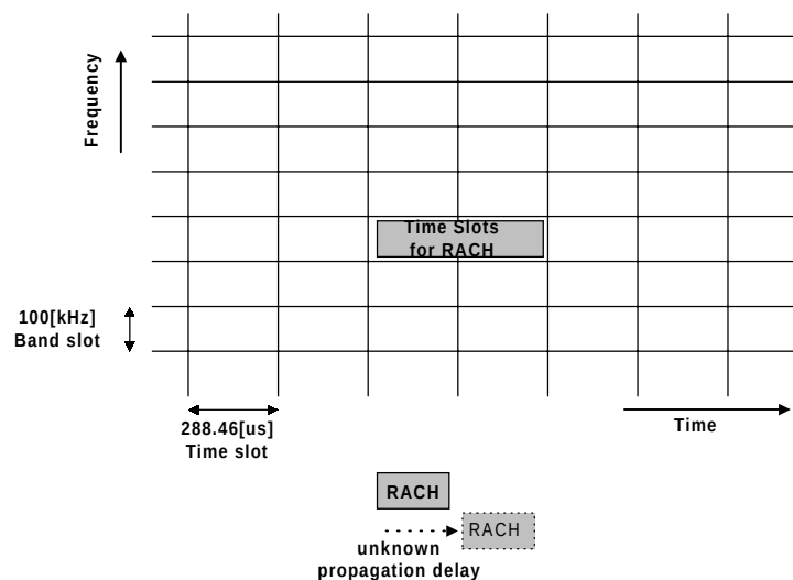
Figure 4: RACH Structure
