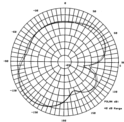
Figure 7: Antenna Pattern (Patch)
