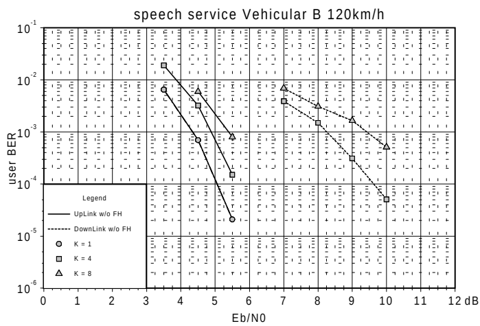
Figure 1-5 Speech UL and DL Vehicular B 120 km/h, 1, 4 and 8 Users per TS, 1 Code and 1 TS per user
