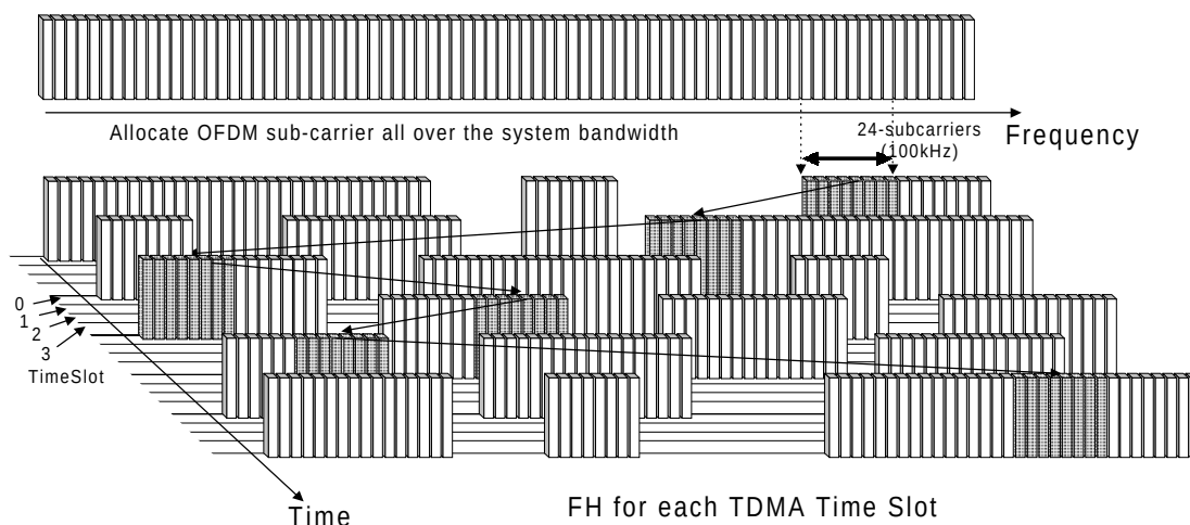
Figure 1: OFDMA Outline (SFH-TDMA)
