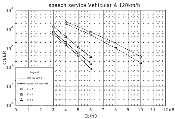
Figure 1-2 Speech UL and DL Vehicular A 120 km/h, 1, 4 and 8 Users per TS, 1 Code and 1 TS per user
