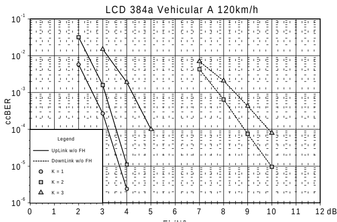
Figure 1-10 LCD 384 a UL and DL Vehicular 120 km/h, 1, 2 and 3 Users per TS, 3 Codes and 8 TS per user
