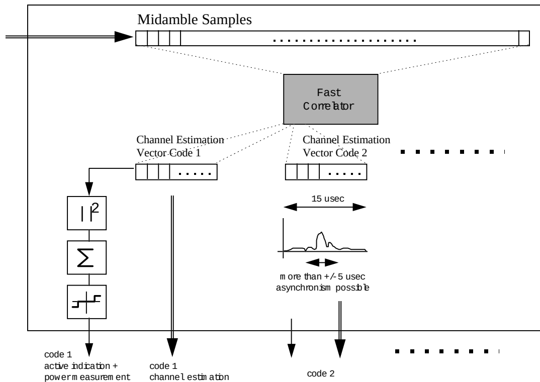
Figure 23 WB-TDMA/CDMA Channel Estimator Function
