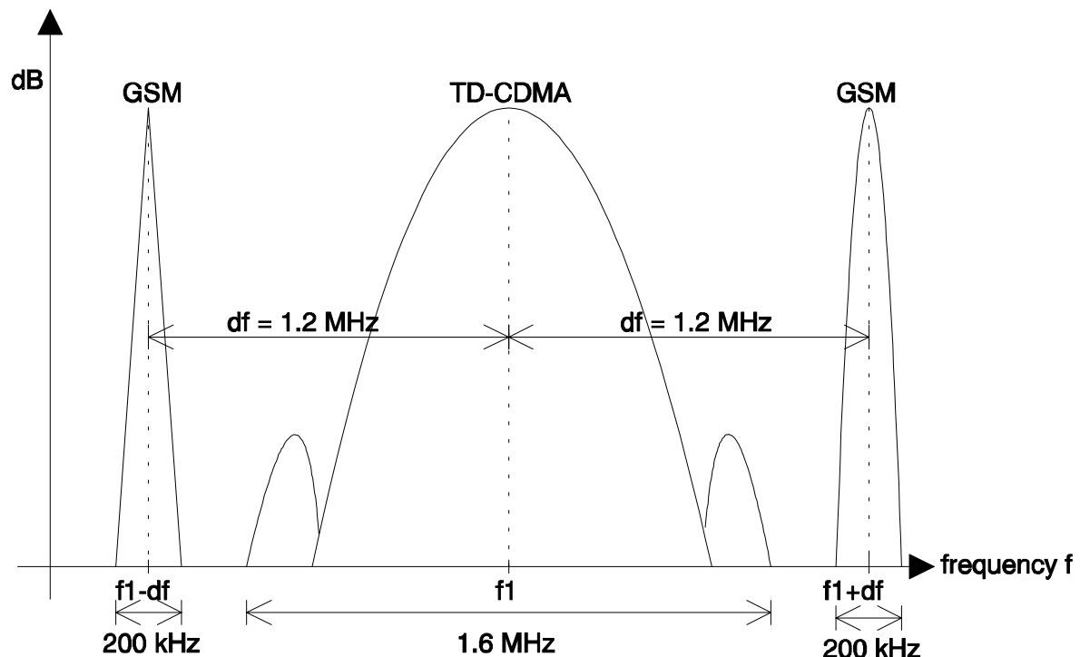
Figure 2-1 WB-TDMA/CDMA and GSM900/1800 carriers use adjacent channels
