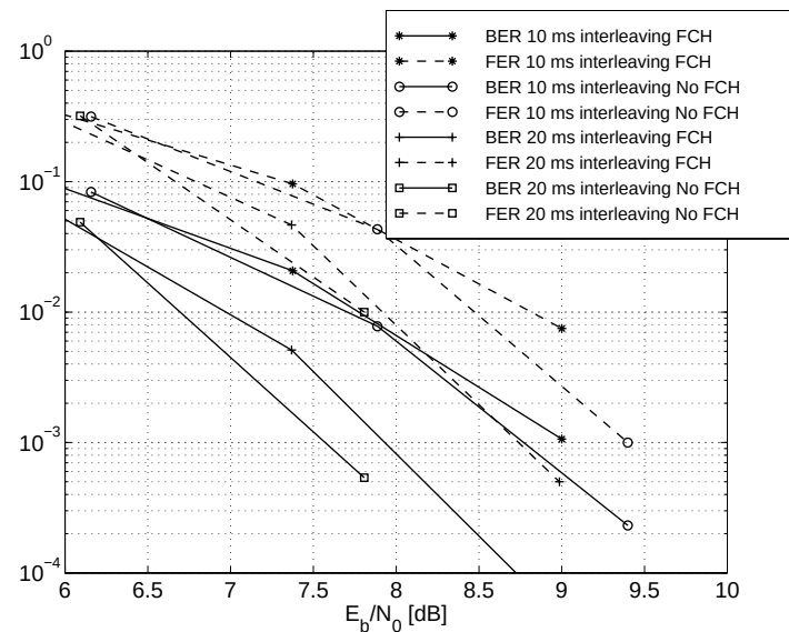
Figure 6. Speech, Vehicular A 120 km/h, without antenna diversity.
