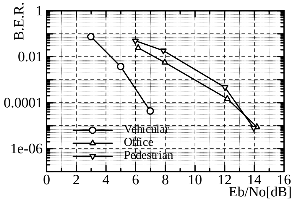
Figure 27: E_b/N_0 vs BER (SPEECH)
