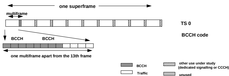
Mapping of the BCCH logical channel
