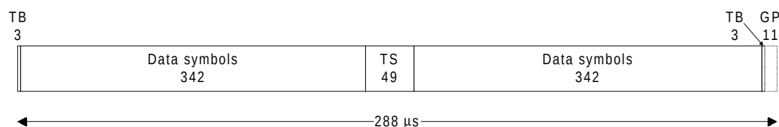
Figure 3-5 Burst structure of the Data burst. TB stands for burst tail symbol, TS for training sequence and GP for guard period.
