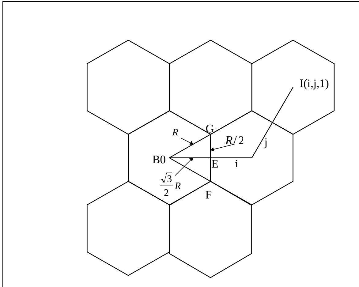
Figure 7: Geometry of interferers
