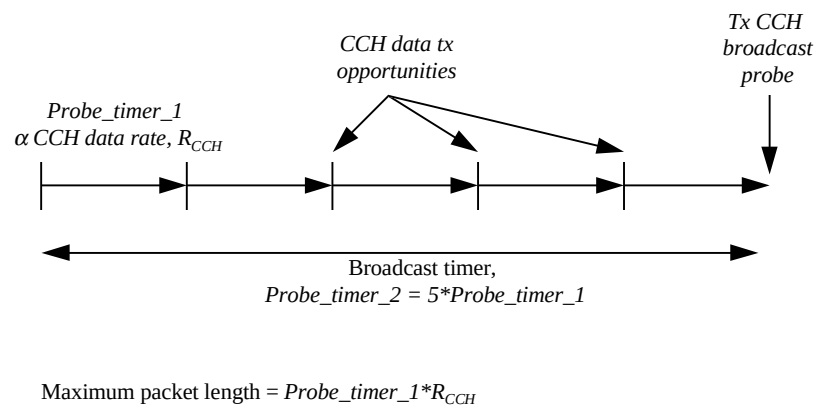
Figure 12. CCH Timer Relationships.
