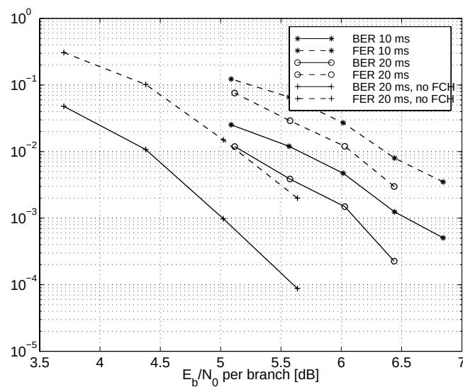
Figure 5. Speech, Vehicular A 120km/h, with antenna diversity.
