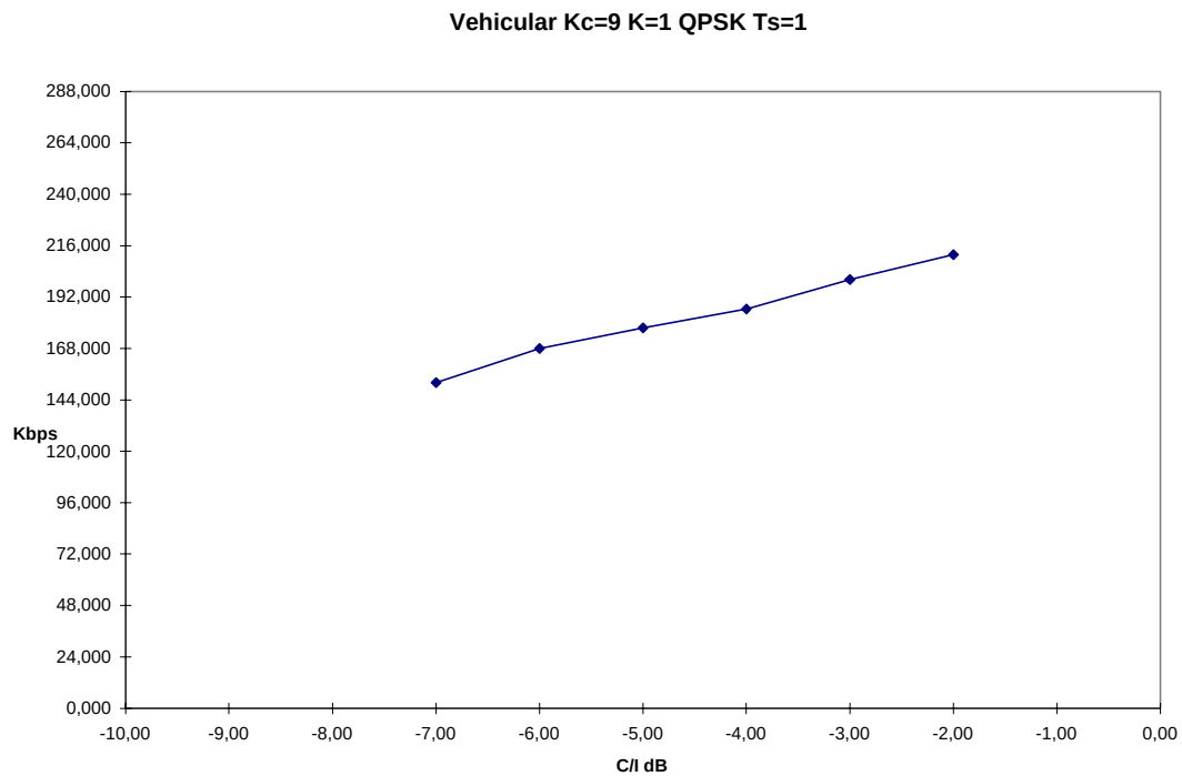
Figure 1-16 UDD 144 kbit/s UL and DL Vehicular 120 km/h, 1 User per TS, 9 Codes and 1 TS per user, QPSK, code rates 1, 2/3, 1/2, 1/3 and 1/4
