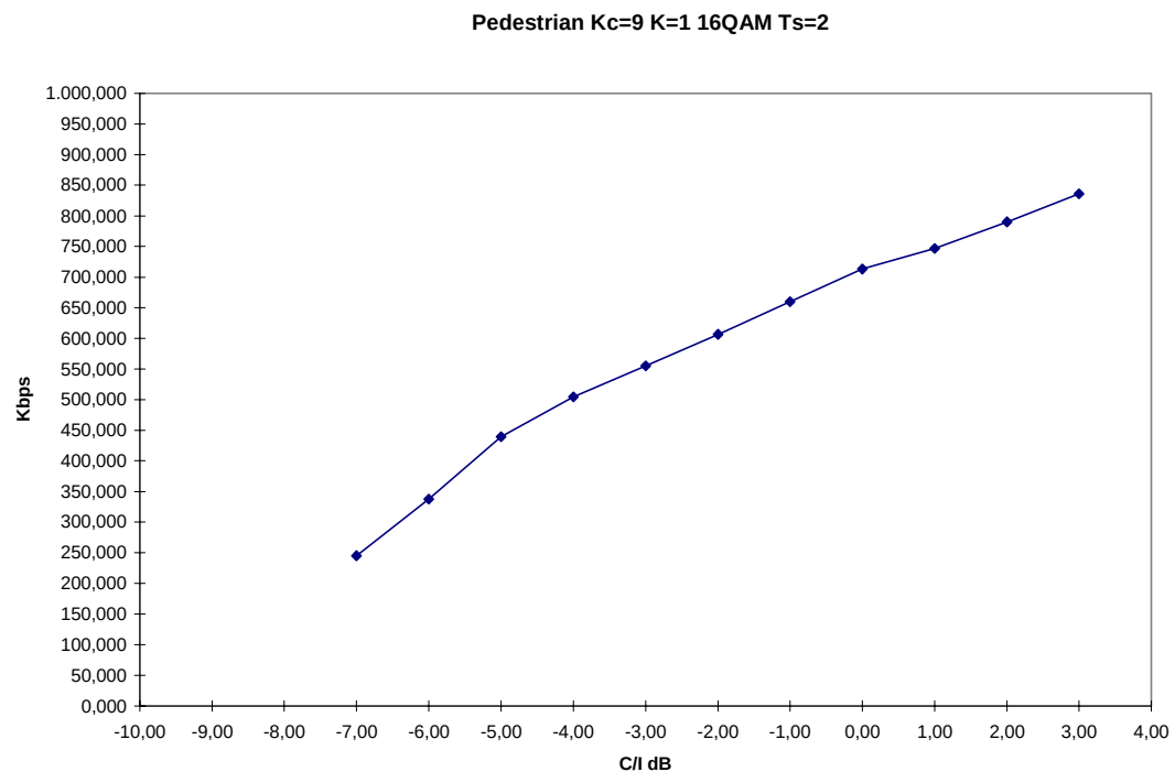
Figure 1-21 UDD 384 kbit/s UL and DL Pedestrian 3 km/h, 1 User per TS, 9 Codes and 2 TS per user, 16QAM, code rates 1, 2/3, 1/2, 1/3 and 1/4
