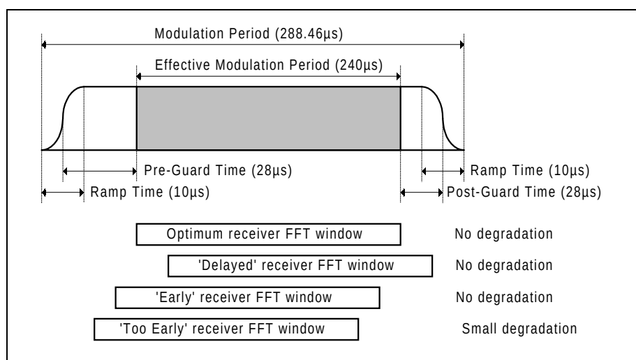
Figure 14: OFDMA burst and synchronisation requirements
