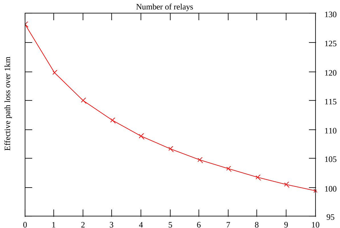
Figure 3 Effective Pathloss v Number of Relays
