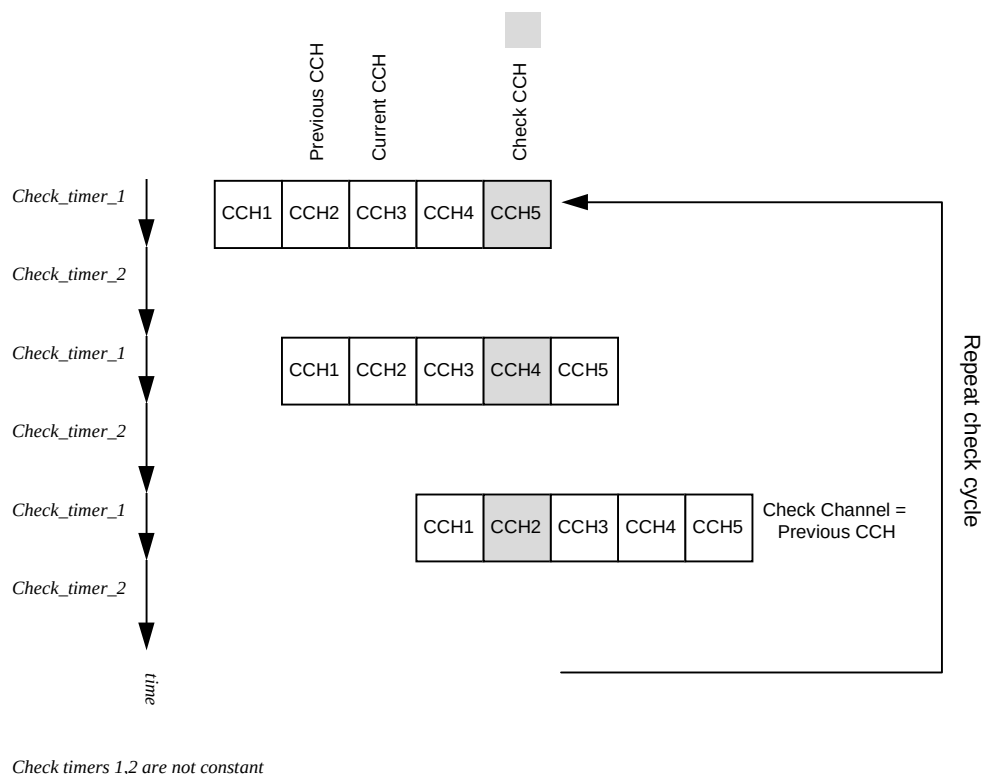
Figure 11. Check channel cycle.
