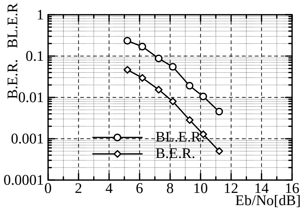
Figure 30 E_b/N_o vs BL.E.R. ( Mode A, Office)
