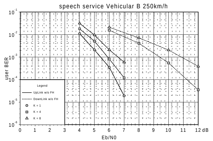
Figure 1-6 Speech UL and DL Vehicular B 250 km/h, 1, 4 and 8 Users per TS, 1 Code and 1 TS per user
