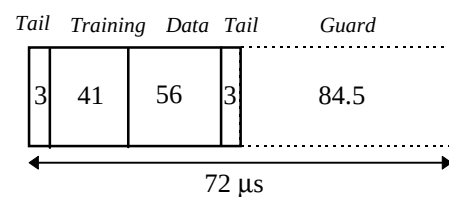
Figure 3-16 The 1/64-slot Access burst.
