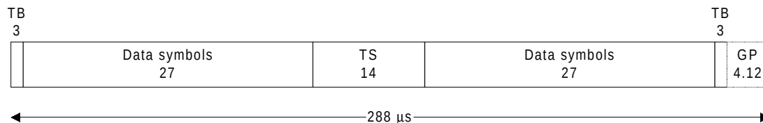
Figure 3-11 : Burst structure of the 1/16 burst for 200 kHz carrier. TB stands for burst tail bit, TS for training sequence and GP for guard period.
