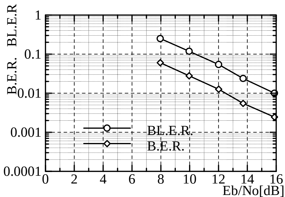
Figure 36 E_b/N_0 vs B.L.E.R. ( UUD2048, Office )
