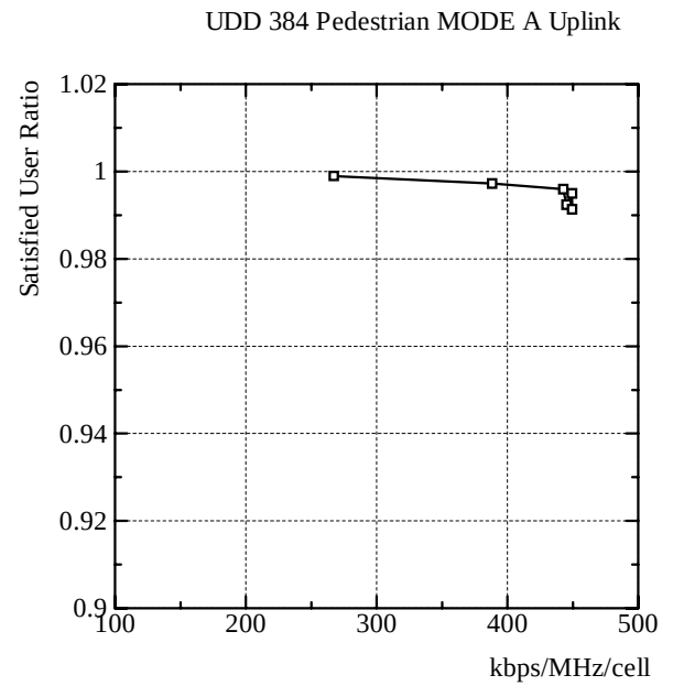
Figure 60: UDD 384 Mode A - Percentage of satisfied users (UL)
