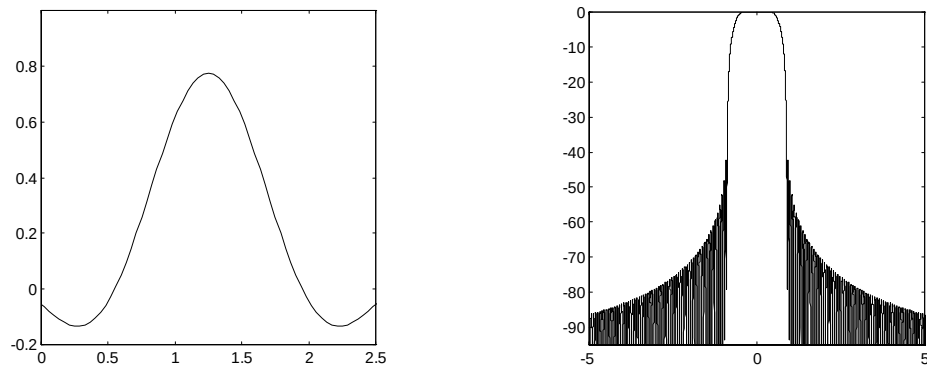
Figure 3-19 Binary Offset QAM basic impulse h(t) and the corresponding energy density spectrum of h(t) with the roll-off factor \alpha=0.35 for a symbol duration 0.38 \mu\text{s} ( 1/2.6 \text{ Msymbol/s} ).
