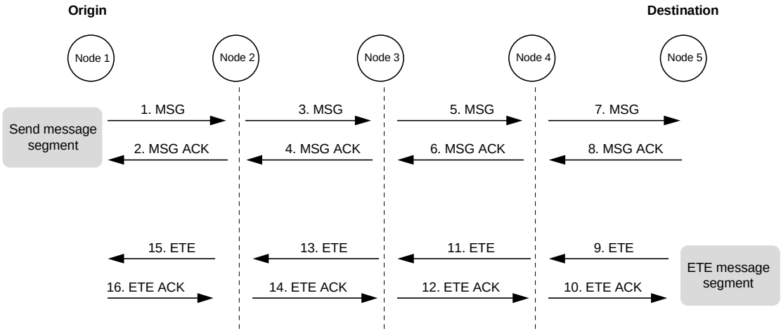
Figure 17. ODMA Layer 2 RLP.
