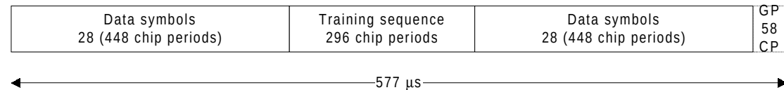
Figure 4-4 Burst structure of the Spread Speech/Data burst 1. GP stands for guard period and CP for chip periods.
