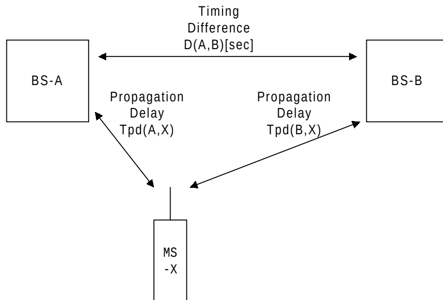
Figure 11: Pseudo Synchronisation
