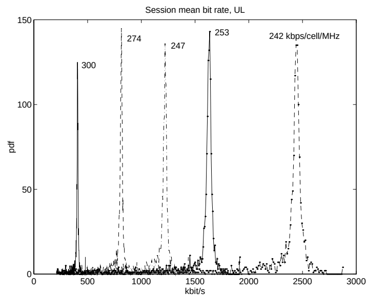
Figure 20. Pdf of uplink session mean bit rate for the UDD 2048 service in the Indoor A environment for 1, 2, 3, 4 and 6 codes. The maximum information bit-rate for one code is 480 kbps. The maximum spectrum efficiency in the uplink is when a single 480 kbps bearer is used (one code), but the other bearers (multicode) show also very good performance.
