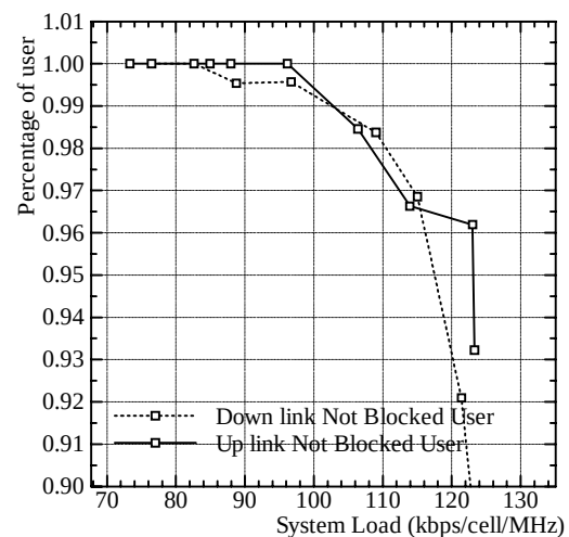
Figure 43: System Bandwidth 3.2MHz
