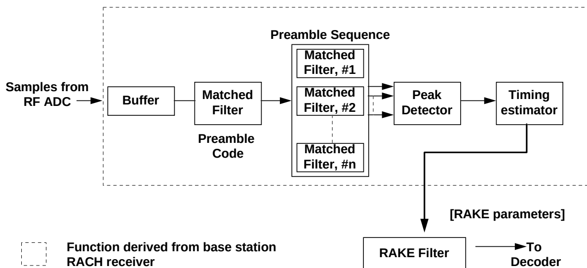
Figure 22 Synchronisation Function
