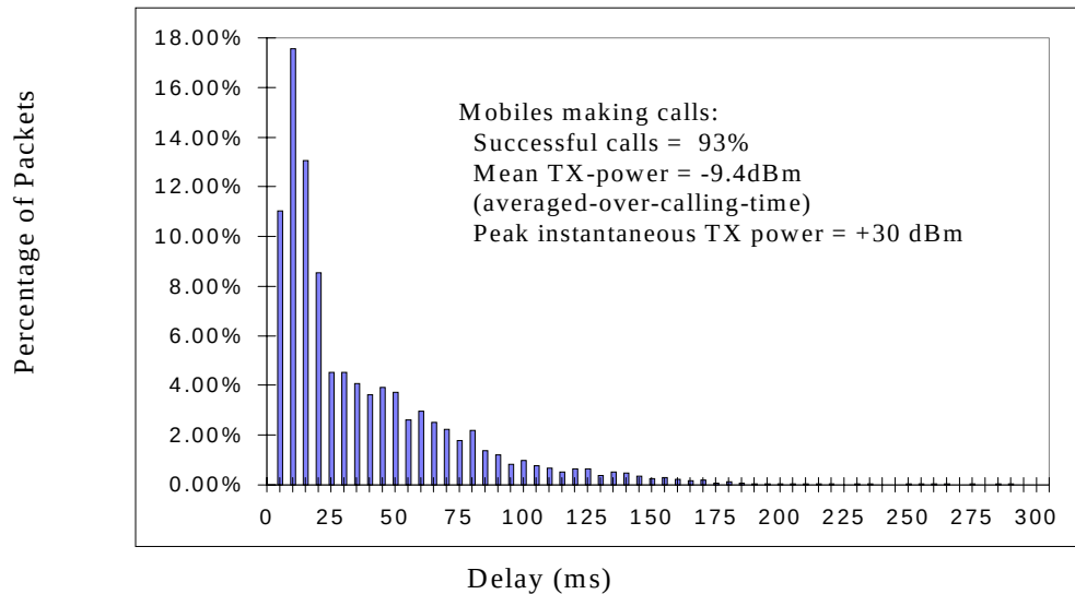
Figure 18 Packet Delay Distribution for Indoor Office (x60) LCD 384kbps Coverage
