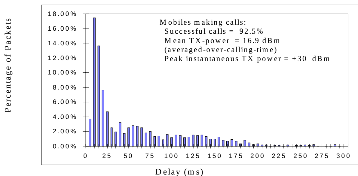
Figure 18 Packet Delay Distribution for Manhattan (10x10) LCD 384kbps Coverage
