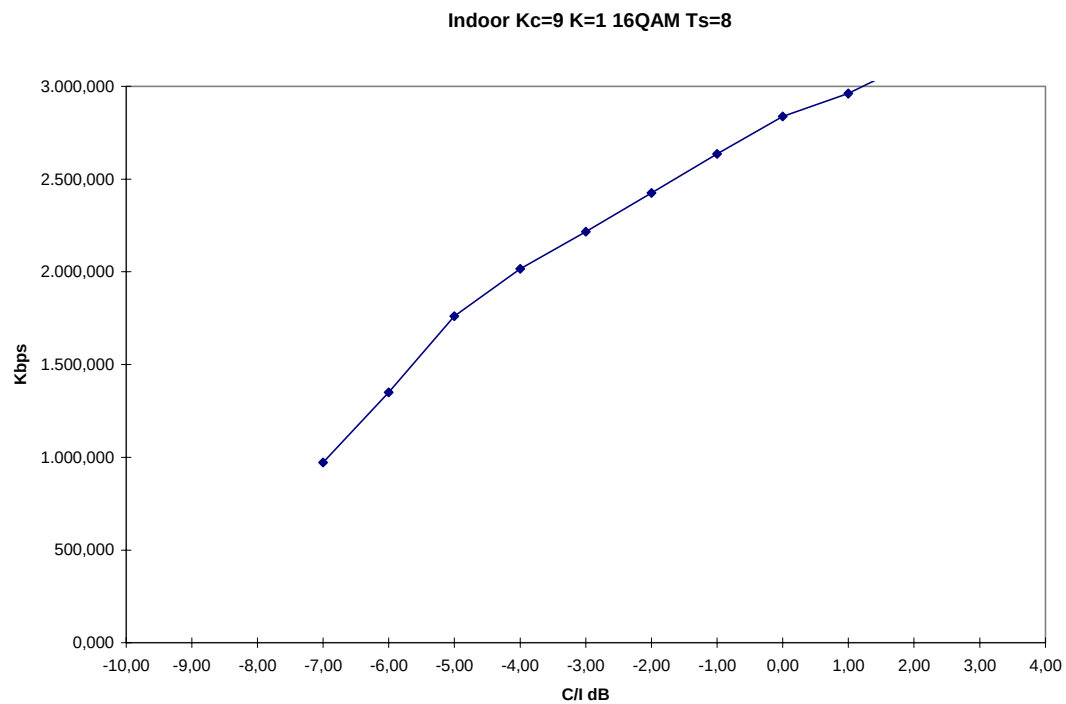
Figure 1-23 UDD 2048 kbit/s UL and DL Indoor 3 km/h, 1 User per TS, 9 Codes and 8 TS per user, 16QAM, code rates 1, 2/3, 1/2, 1/3 and 1/4
