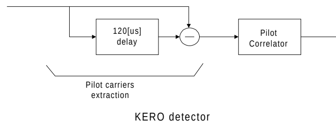
Figure 3: KERO detector
