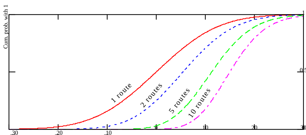
Figure 4 Benefits of Path Selection - Space Diversity
