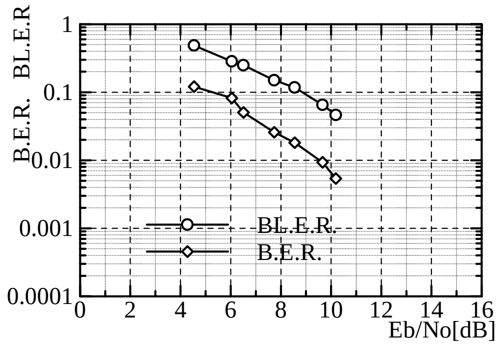
Figure 35 E_b/N_o vs BL.E.R. ( Mode B, Vehicular)
