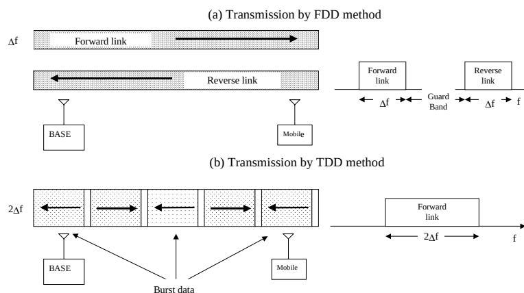
Figure 32 Principle for FDD and TDD operation
