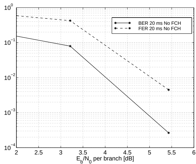
Figure 7. Speech, Vehicular B 120 km/h, with antenna diversity.
