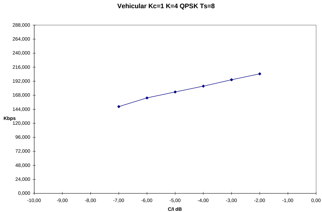
Figure 1-18 UDD 144 kbit/s UL Vehicular 120 km/h, 4 Users per TS, 1 Code and 8 TS per user, QPSK, code rates 1, 2/3, 1/2, 1/3 and 1/4
