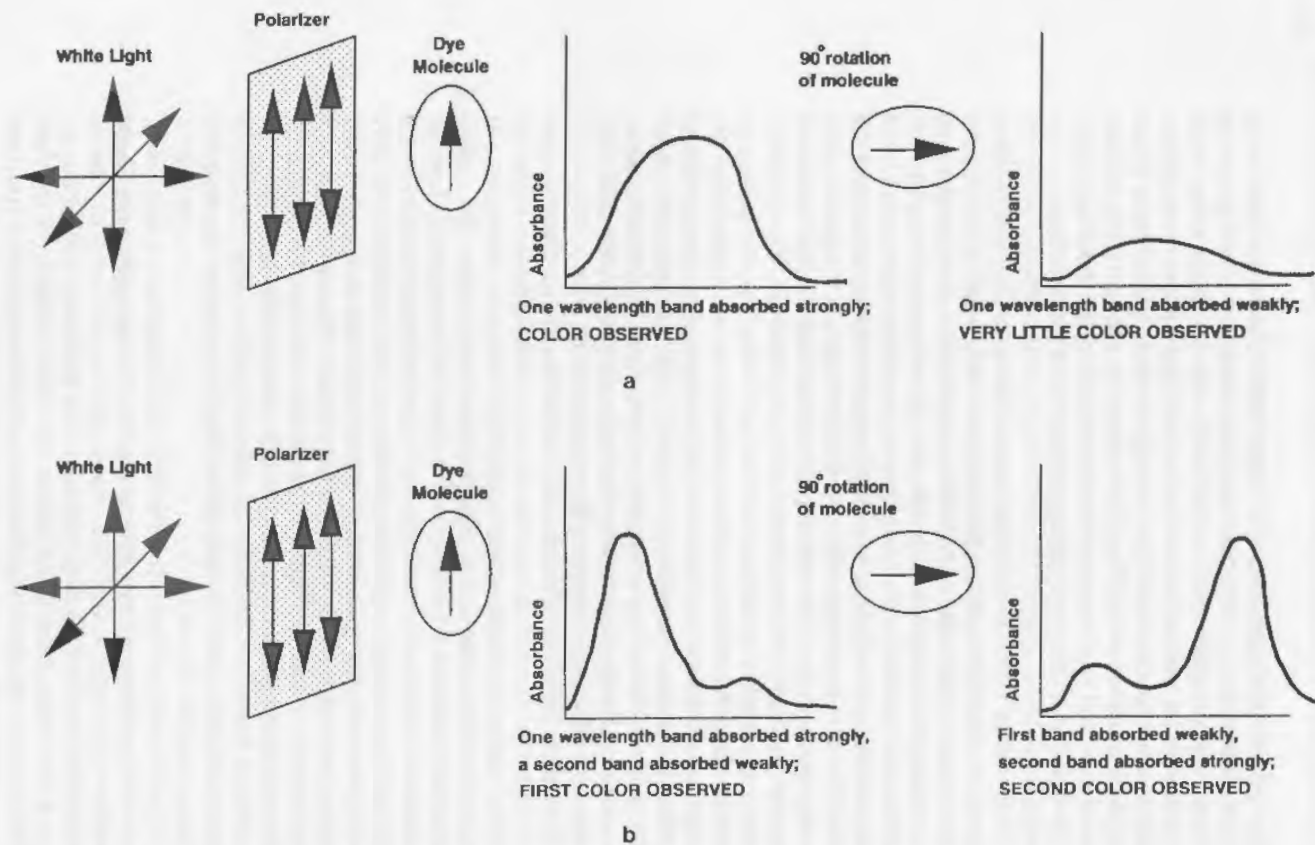
Figure 8.13 Optical characteristics of dichroic and pleochroic dyes. (a) Dichroic dye: Absorption spectra in two orientations with respect to polarized light. (b) Pleochroic dye: Absorption spectra in two orientations with respect to polarized light.
