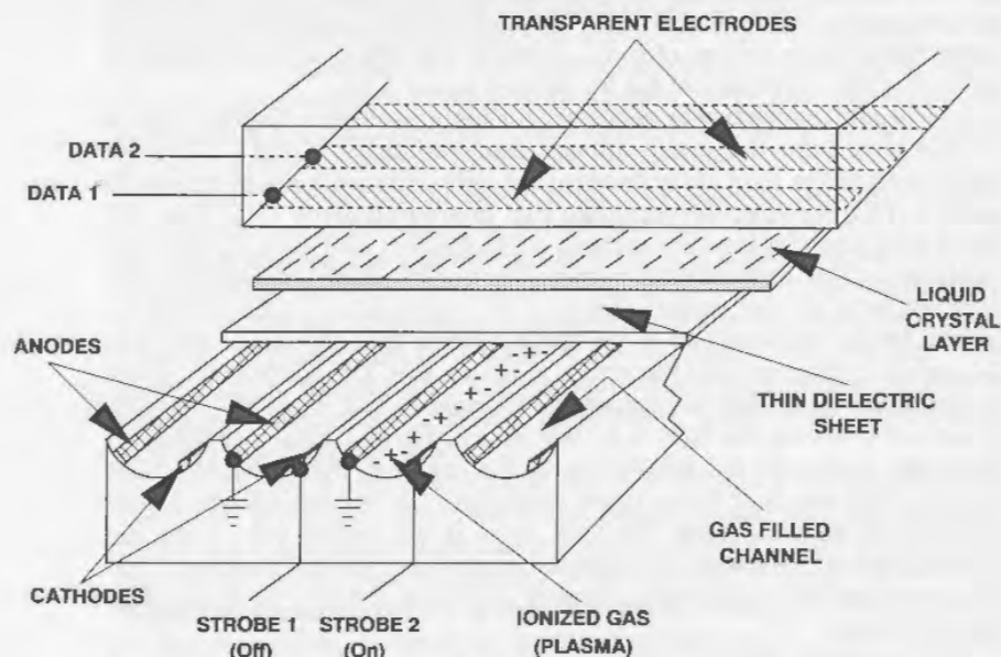
Figure 8.12 Plasma addressed LCD structure and operation.
