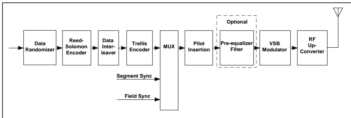
Figure 1. VSB transmitter.
