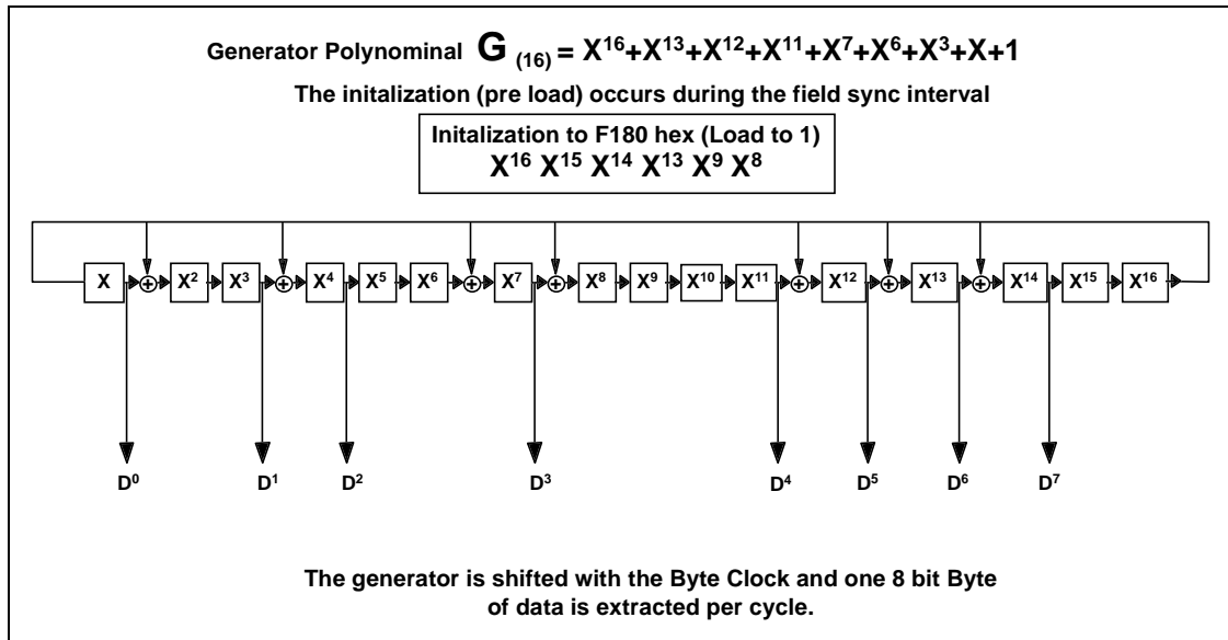
Figure 4. Randomizer polynomial.
