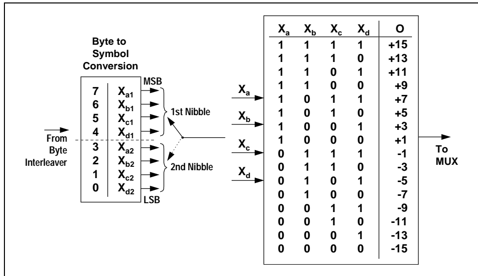
Figure 15.16 VSB mapper.
