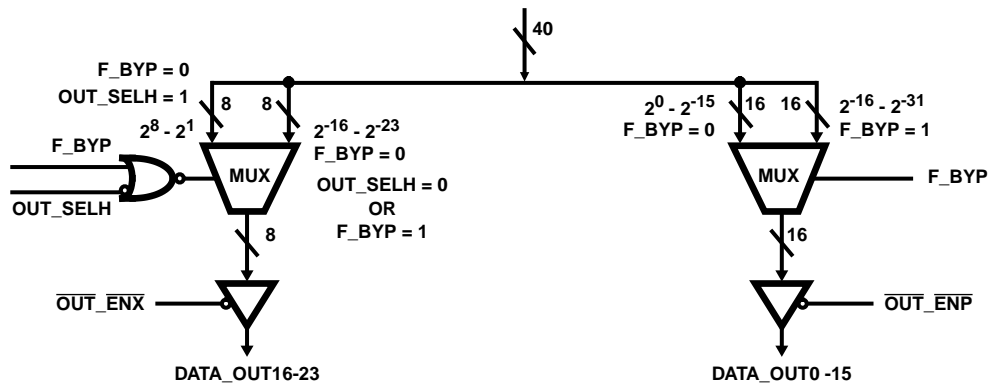
FIGURE 10. FIR OUTPUT FORMATTER
