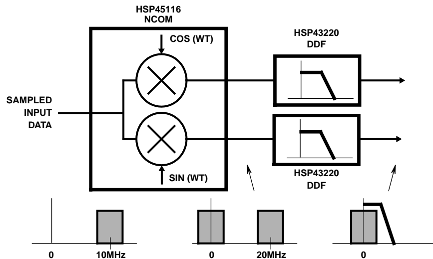
FIGURE 14. DIGITAL CHANNELIZER
