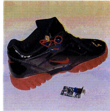
PAN transmitter and PAN III RS232-to-body modem.
