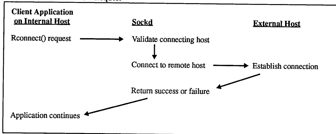
FIGURE 3. CONNECT Request
