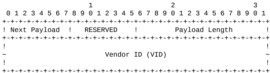
Figure 17: Vendor ID Payload Format
