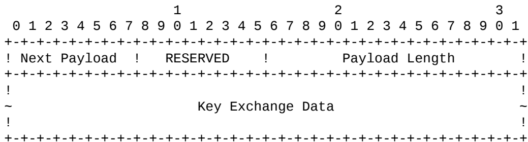
Figure 8: Key Exchange Payload Format
