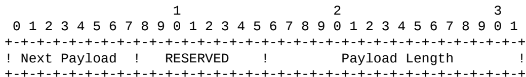
Figure 3: Generic Payload Header
