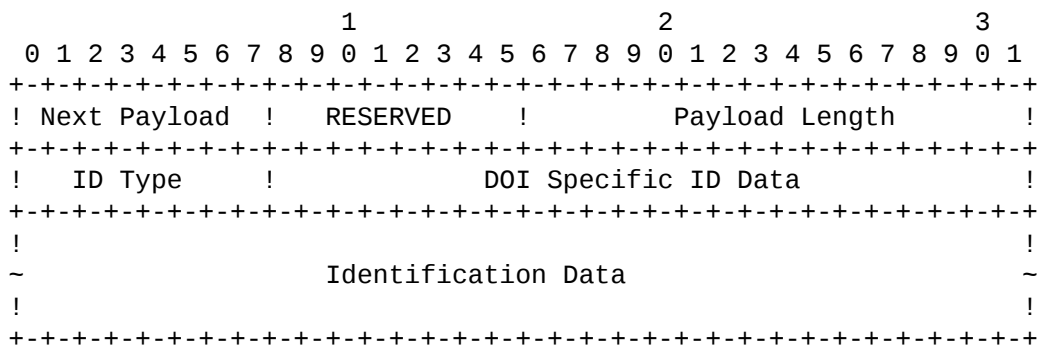
Figure 9: Identification Payload Format
