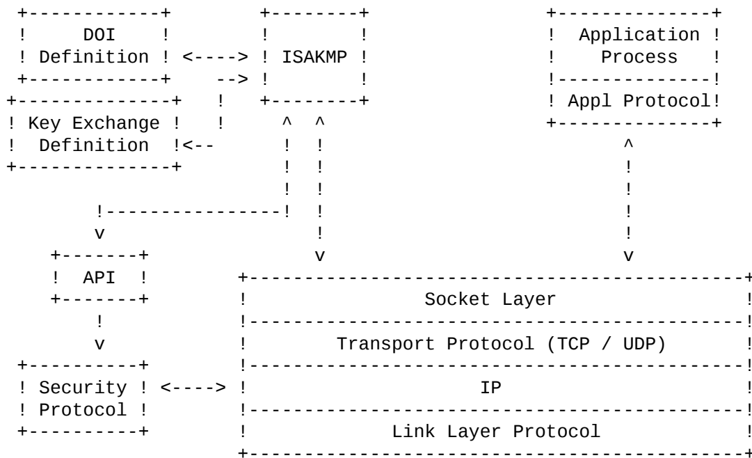
Figure 1: ISAKMP Relationships
