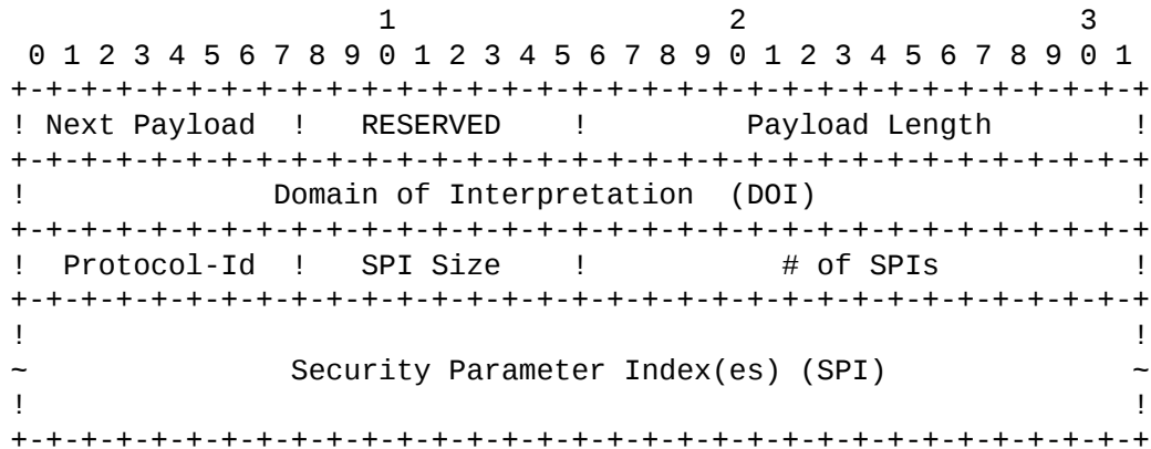
Figure 16: Delete Payload Format
