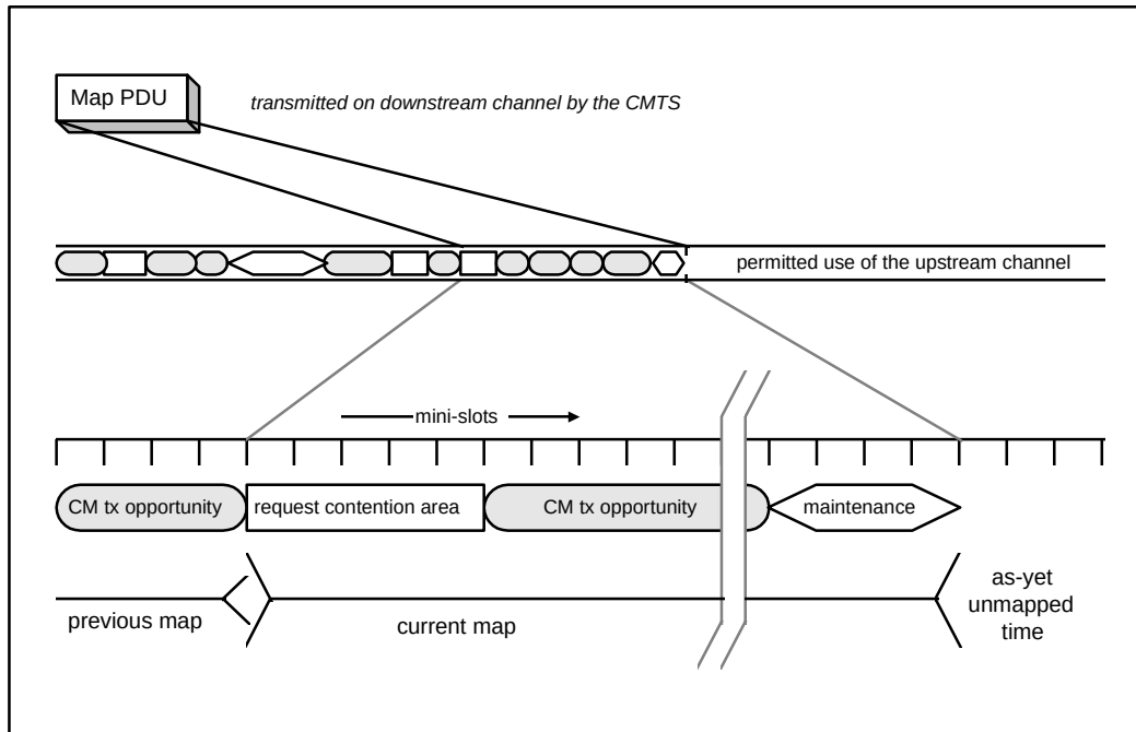
Figure 0-31. Allocation Map
