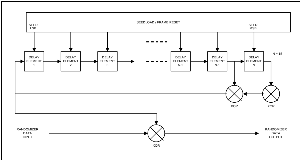
Figure 0-4. Scrambler Structure
