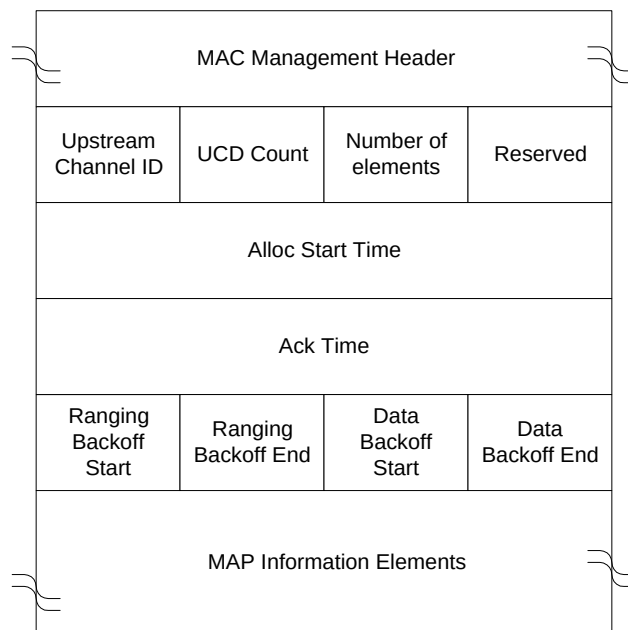
Figure 0-18. MAP Format
