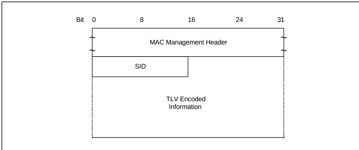
Figure 0-25. Registration Request
