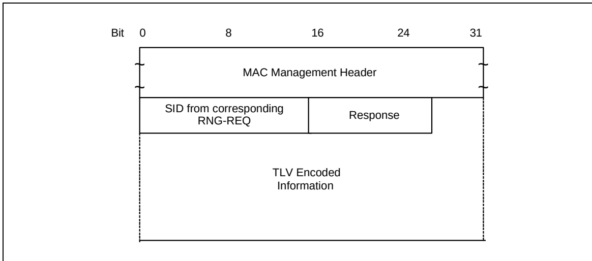
Figure 0-27. Registration Response Format
