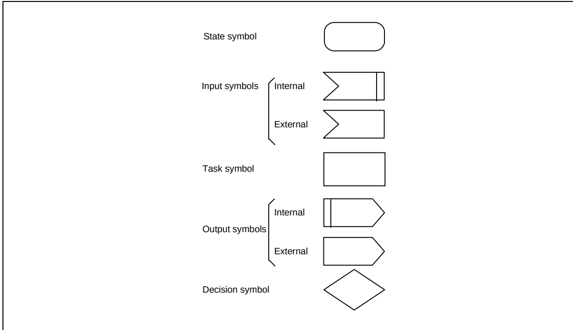
Figure 0-2. SDL Notation
