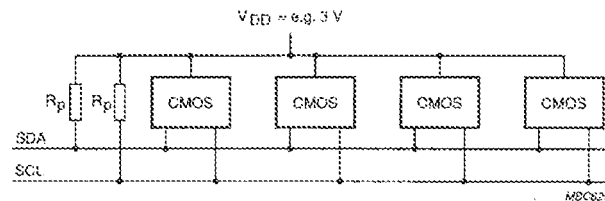
Fig. 22 Devices with wide supply voltage range connected to the I 2 C-bus
