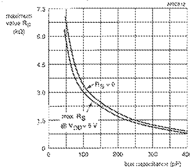
Fig.38 Maximum value of R_p as a function of bus capacitance for meeting the t_{R\text{ max}} requirement for a fast-mode I 2 C-bus
