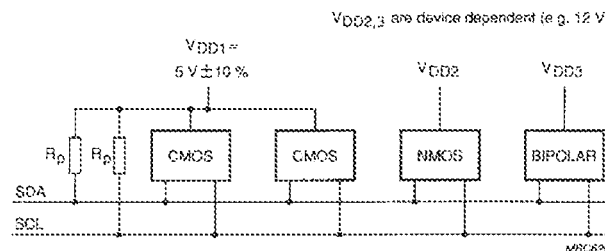
Fig. 23 Devices with input levels related to V DD (supply V DD1 ) mixed with fixed input level devices (supply V DD2,3 ) on the I 2 C-bus
