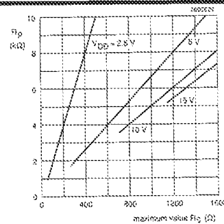
Fig.26 Maximum values of R_s as a function of the value of R_p with supply voltage as a parameter
