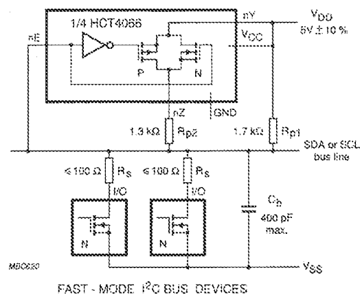
Fig.37 Switched pull-up circuit
