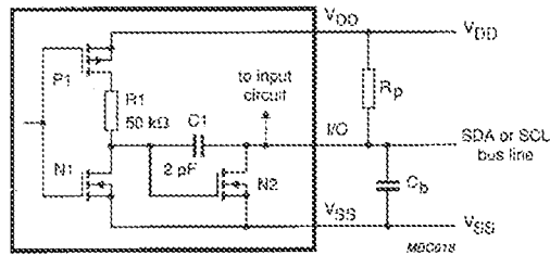
Fig.35 Slope-controlled output stage in CMOS technology
