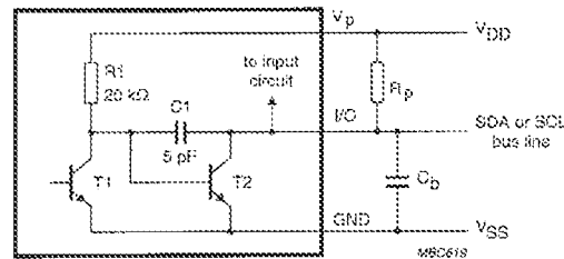
Fig.36 Slope-controlled output stage in bipolar technology
