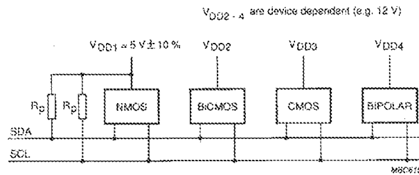
Fig. 21 Fixed input level devices connected to the I 2 C-bus
