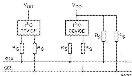
Fig. 24 Series resistors (R s ) for protection against high-voltage spikes
