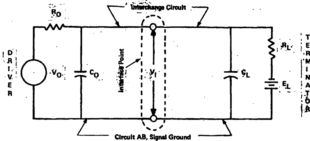
FIGURE 2.1 - INTERCHANGE EQUIVALENT CIRCUIT
