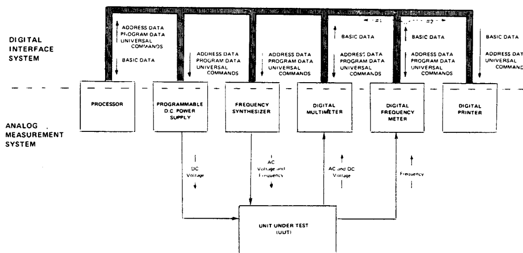
Figure A.1—Typical System Showing Capability of Interface System to Handle Variety of Instrumentation System Needs
