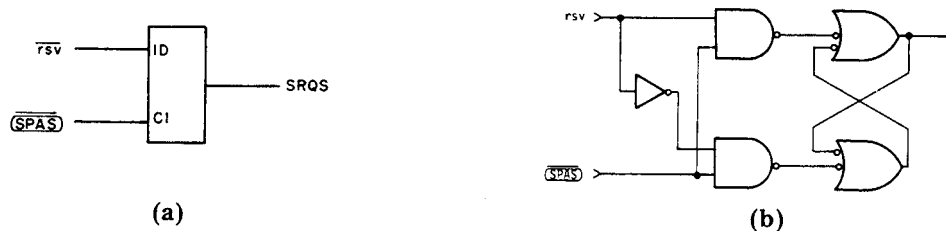
Figure F.1—Partial SR Function — (a) Composite Logic; (b) Gate Level Logic
