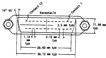
Figure 17—Receptacle Dimensions
