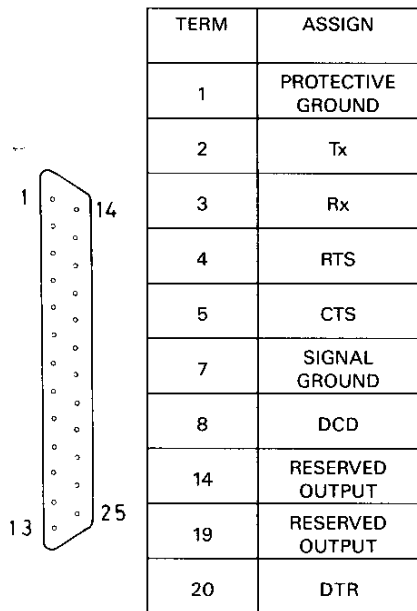
Figure 2.2.1 RS232C
