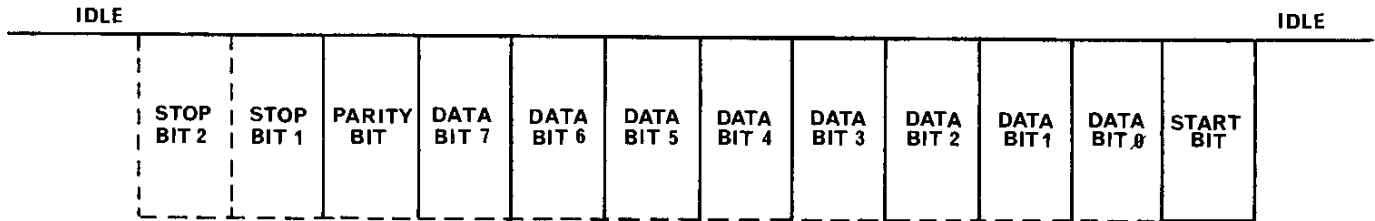
(a) 1 start, 8 data, 1 parity, 2 stop
