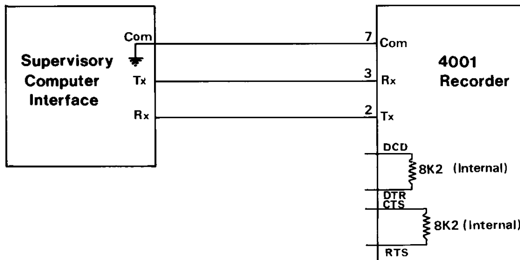
Figure 1.1.2 Typical RS232 Data Bus Connections
