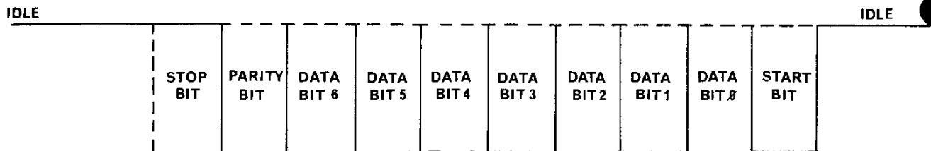
(c) 1 start, 7 data, 1 parity, 1 stop
