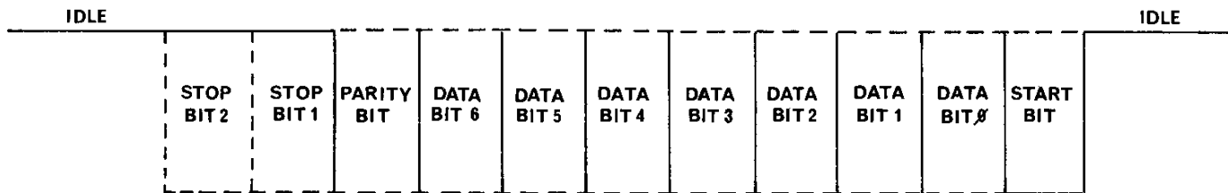
(b) 1 start, 7 data, 1 parity, 2 stop
