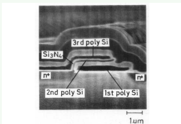
Fig. 2. SEM cross section of a stacked capacitor cell fabricated using 3\mu\text{m} nMOS technology.
