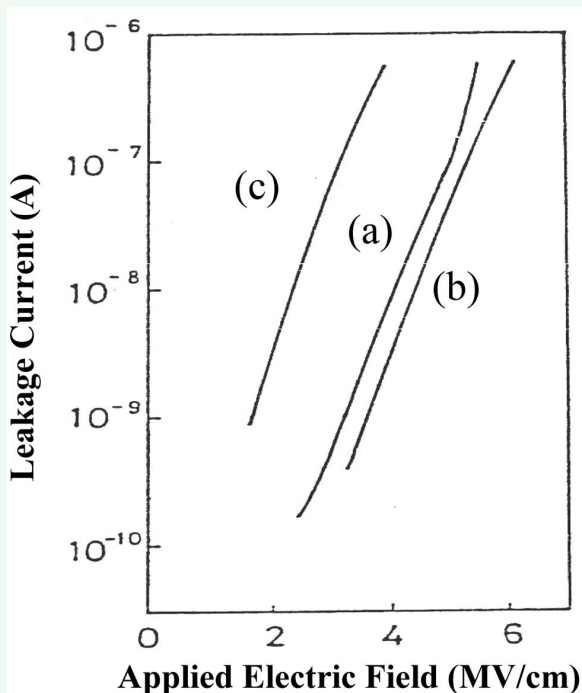
Fig. 4. Leakage current - applied electric field characteristics of storage capacitors. (a) poly-Si- \text{SiO}_2 -poly-Si, (b) poly-Si- \text{SiO}_2/\text{Si}_3\text{N}_4(\text{ON}) -poly-Si, (c) poly-Si- \text{Ta}_2\text{O}_5 -poly-Si.
