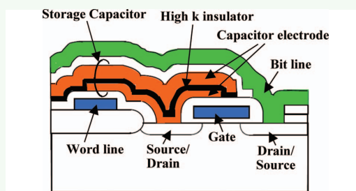
Fig. 1. Basic structure of stacked capacitor cell (STC).
