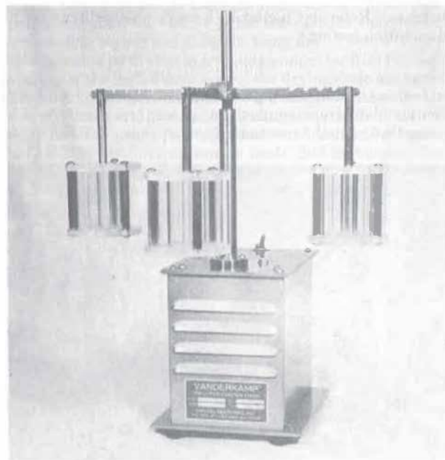
Fig 90-5. Vanderkamp Tablet Disintegration Tester (courtesy, Van-Kel).
