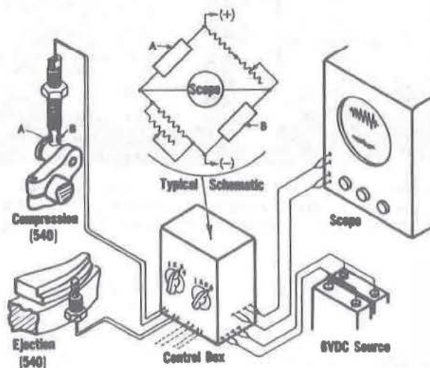
Fig 90-25. Upper photo: High-speed rotary press equipped with strain gauges; Lower photo: layout showing arrangement of electronic components (courtesy, Upjohn).
