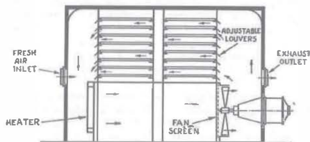
Fig 90-9. Cross section of tray dryer.
