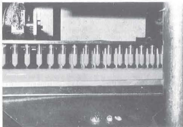
Fig 90-31. Manufacturer of hard gelatin capsules by dipping stainless steel pins into gelatin solutions (courtesy, Lilly).
