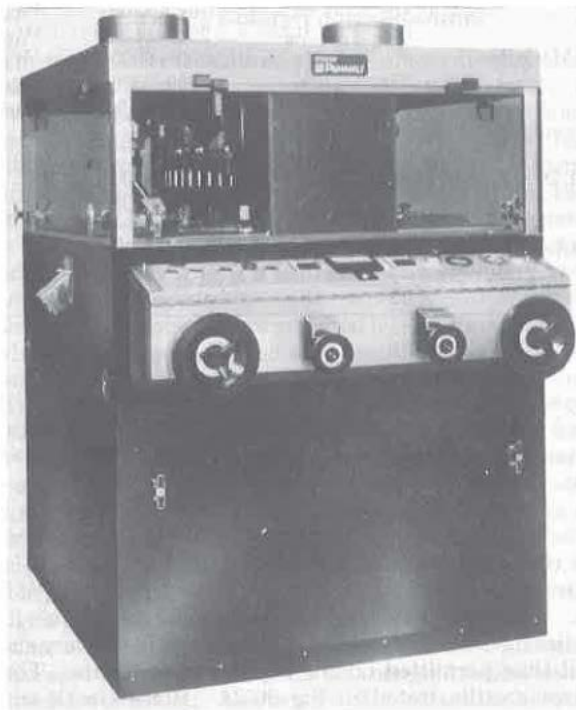
Fig 90-19. Model 747 High Speed Press, double-sided rotary compacting press designed to produce at speeds over 10,000/min (courtesy, Stokes/Pennwalt).
