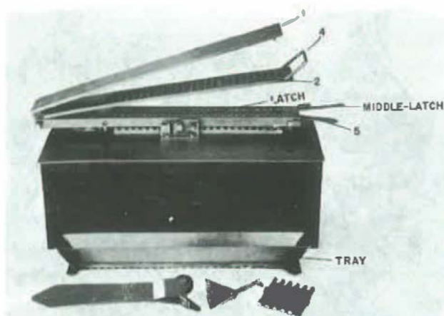
Fig 90-33. Hand-operated capsule machine (courtesy, ChemiPharm).
