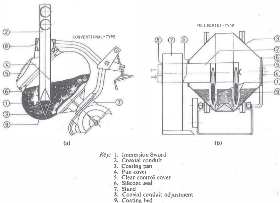
Fig 91-5. Schematic diagram of the immersed sword apparatus for use in either (a) a conventional pan or (b) a Pellegrini pan.
