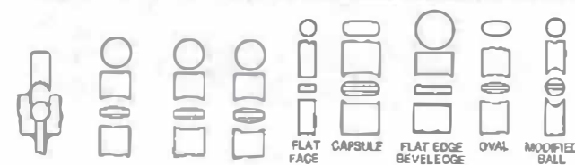
Fig 90-14. Concave punches.
