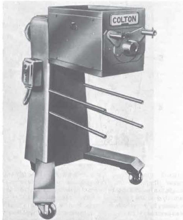
Fig 90-8. Rotary granulator and sifter (courtesy, Vector/Colton).
