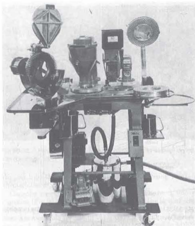
Fig 90-36. Type 8 capsule-filling machine (courtesy, Lilly).
