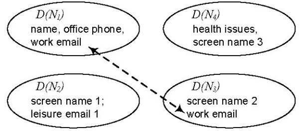
Fig. 3. Discretionary privacy model.
