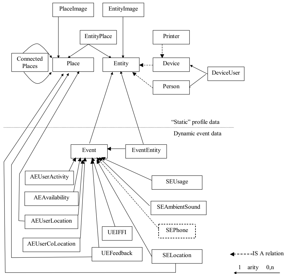
Figure 5: Database schema
