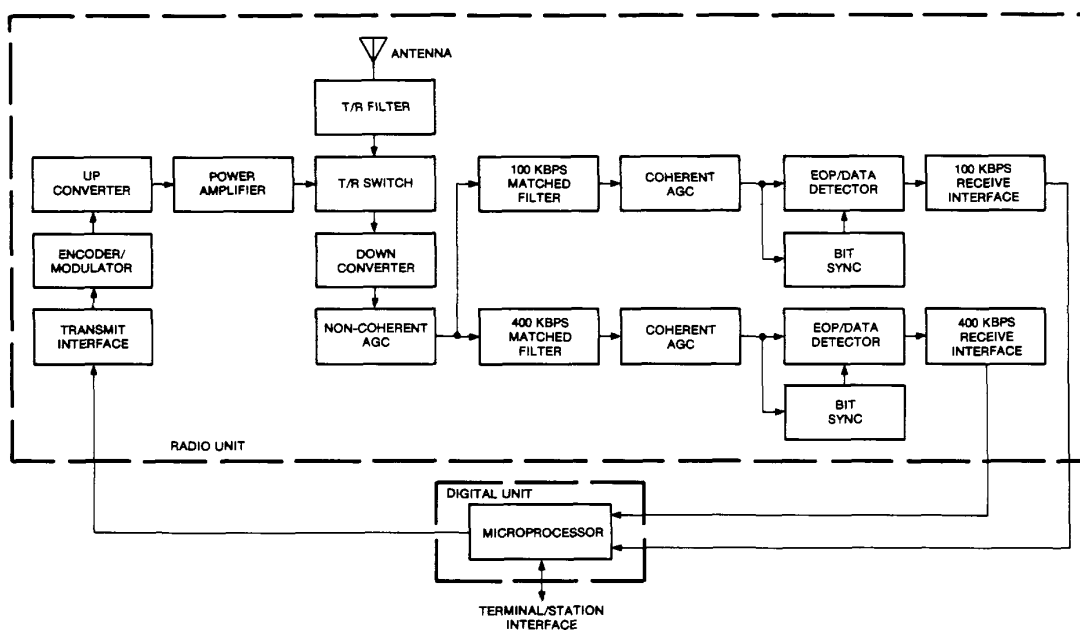
Fig. 13. Experimental packet radio configuration.
