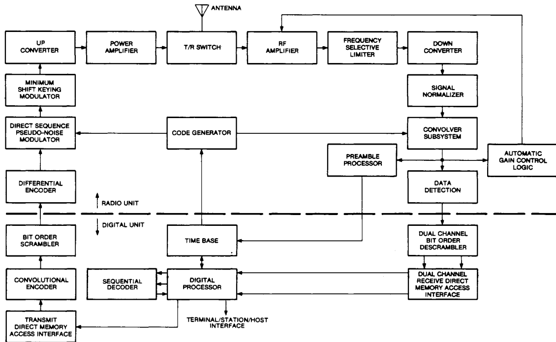
Fig. 14. Upgraded packet radio configuration.
