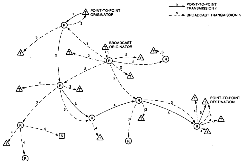
Fig. 9. Point-to-point and broadcast routing.
