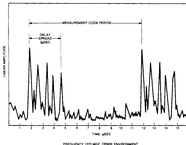
Fig. 3. Received multipath energy.
