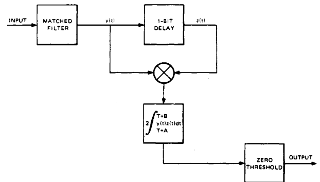
Fig. 18. DPSK receiver using post-detection integration.
