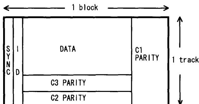
Fig. 6 Error Correction Code Configuration
