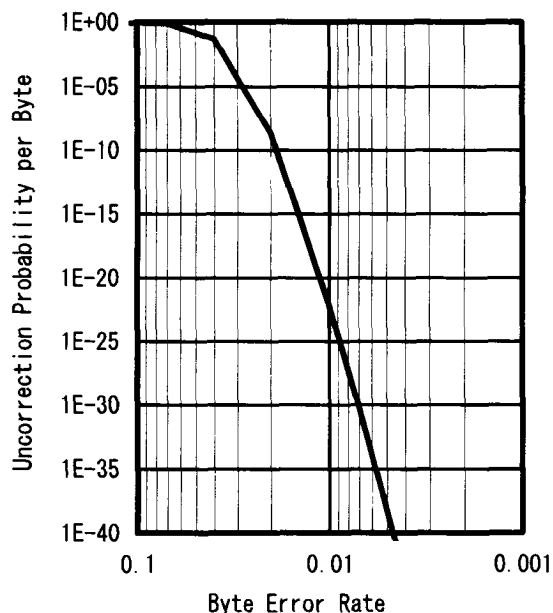
Fig. 7 Error Correction Capability
