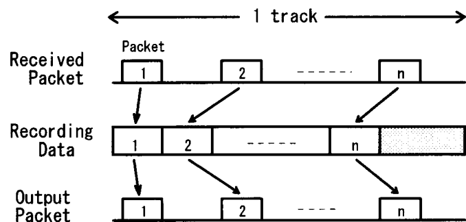
Fig. 4 Packet Transmission Timing
