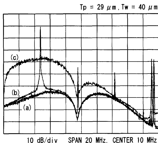
Fig. 9 Power Spectrum of The Reproduced Signal
