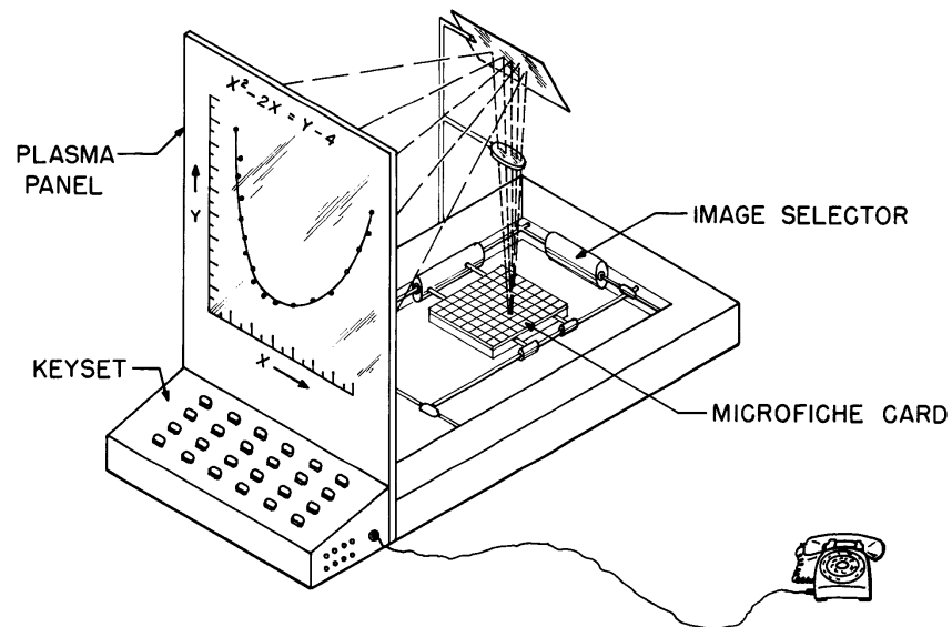
Fig. 3. Proposed Student Terminal
