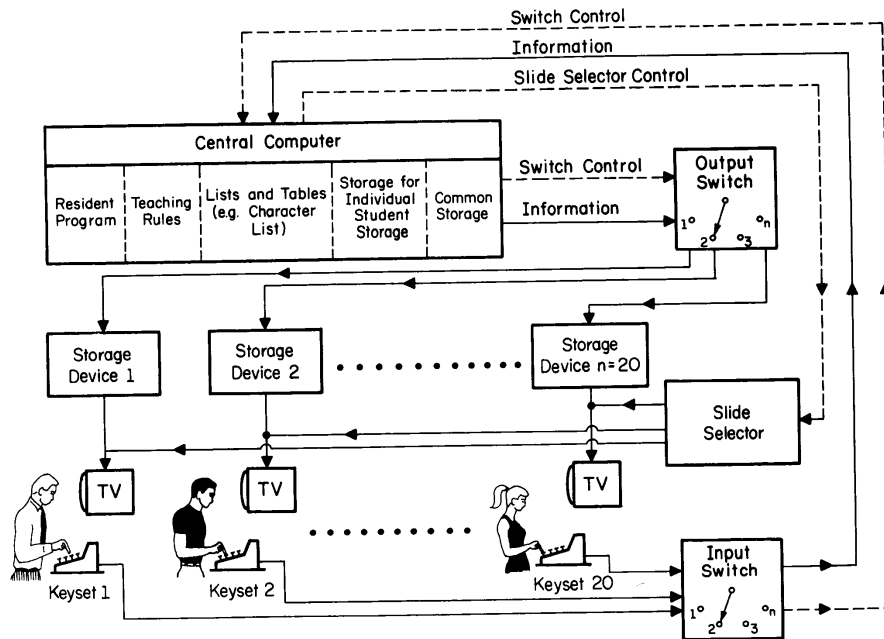
Fig. 1. Present PLATO System Block Diagram
