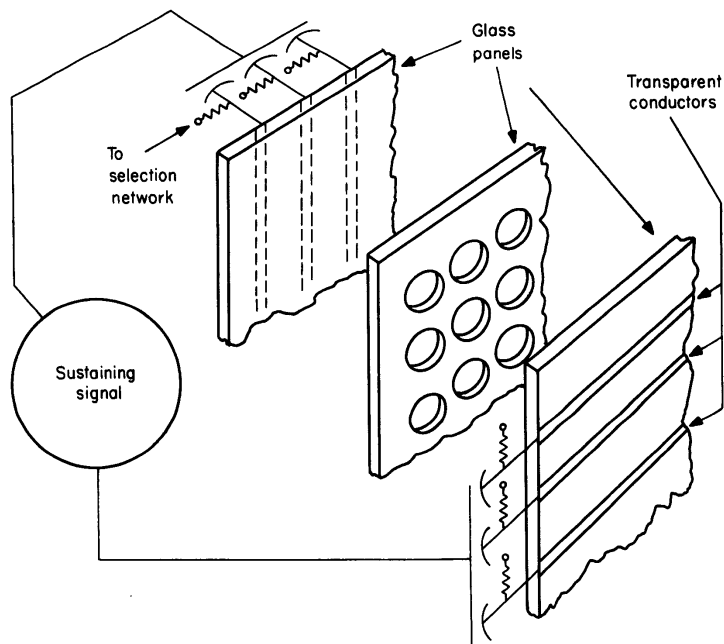
Fig. 2. Plasma Display Panel
