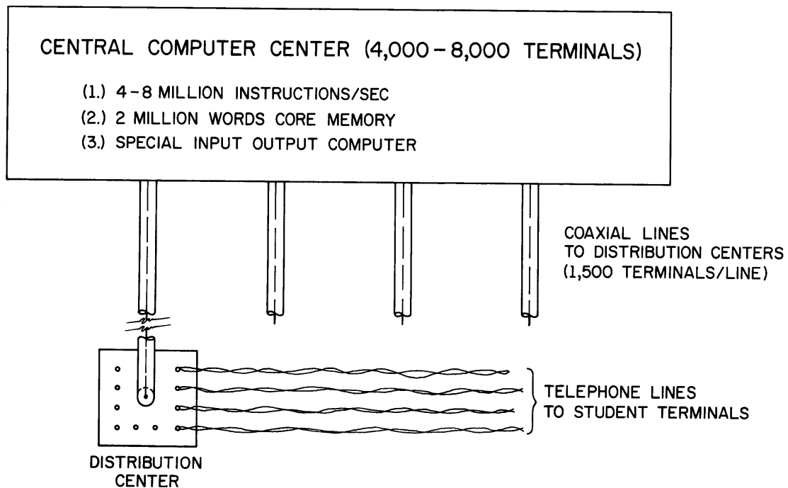
Fig. 4. Block Diagram of Proposed Distribution System
