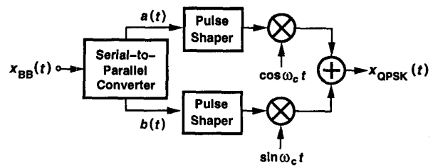
Fig. 9. QPSK modulation with pulse shaping.
