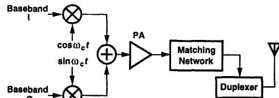
Fig. 16. Direct-conversion transmitter.
