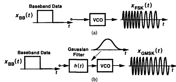
Fig. 1. Generation of (a) FSK and (b) GMSK signals. the VCO and x_{BB}(t) the baseband signal.
