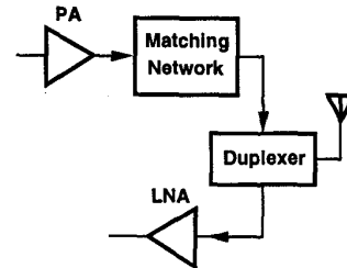
Fig. 10. PA/antenna interface.
