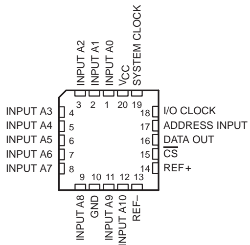
FN PACKAGE (TOP VIEW)
