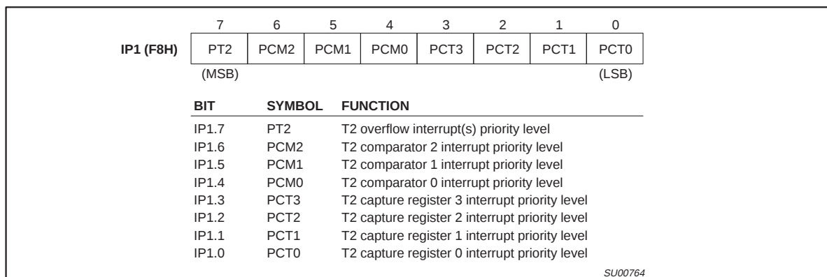
Figure 31. Interrupt Priority Register (IP1)
