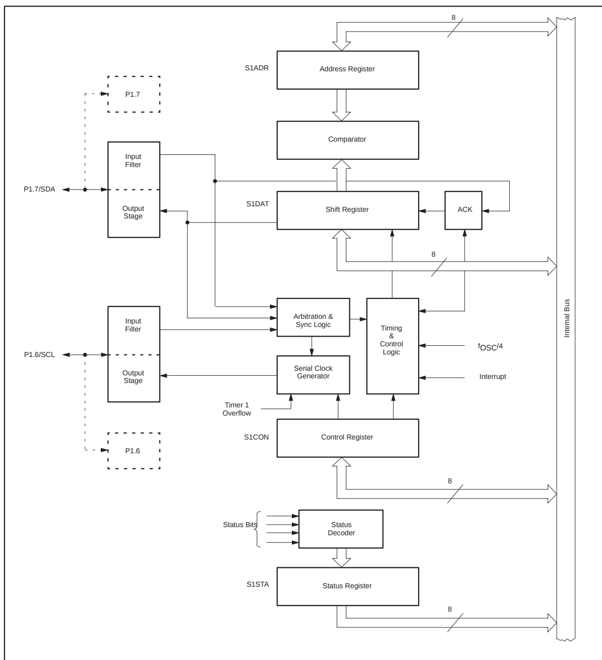
Figure 12. I²C Bus Serial Interface Block Diagram
