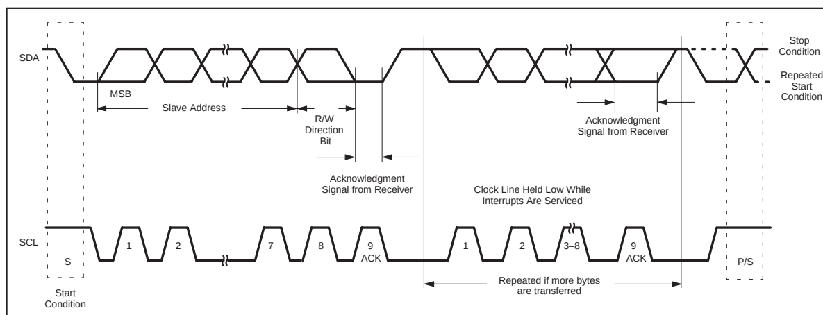
Figure 11. Data Transfer on the I²C Bus
