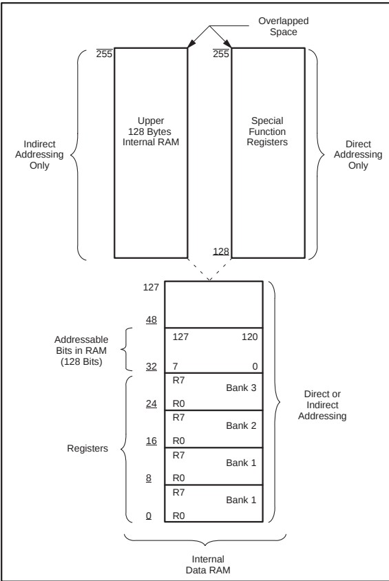
Figure 42. Internal Data Memory Address Space
