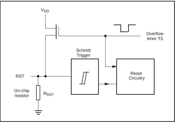
Figure 25. On-Chip Reset Configuration
