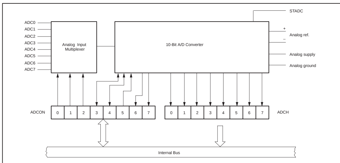
Figure 34. Functional Diagram of Analog Input Circuitry
