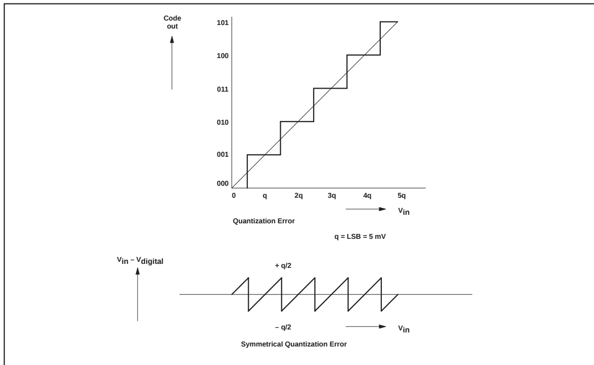
Figure 40. Effective Conversion Characteristic
