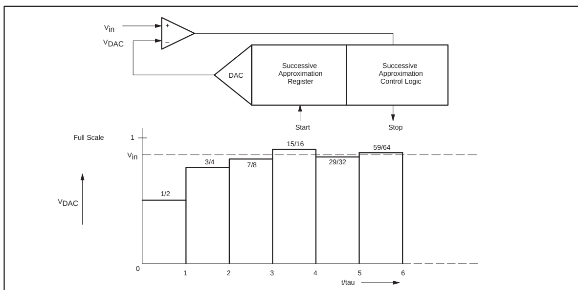
Figure 35. Successive Approximation ADC
