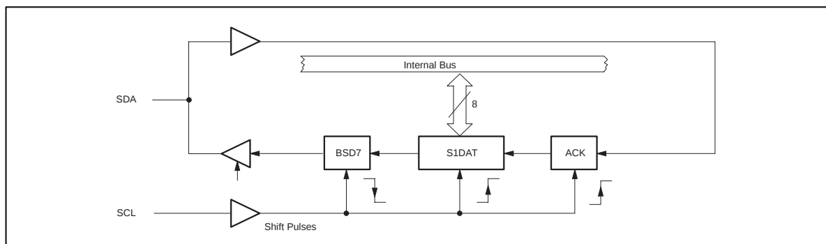
Figure 15. Serial Input/Output Configuration
