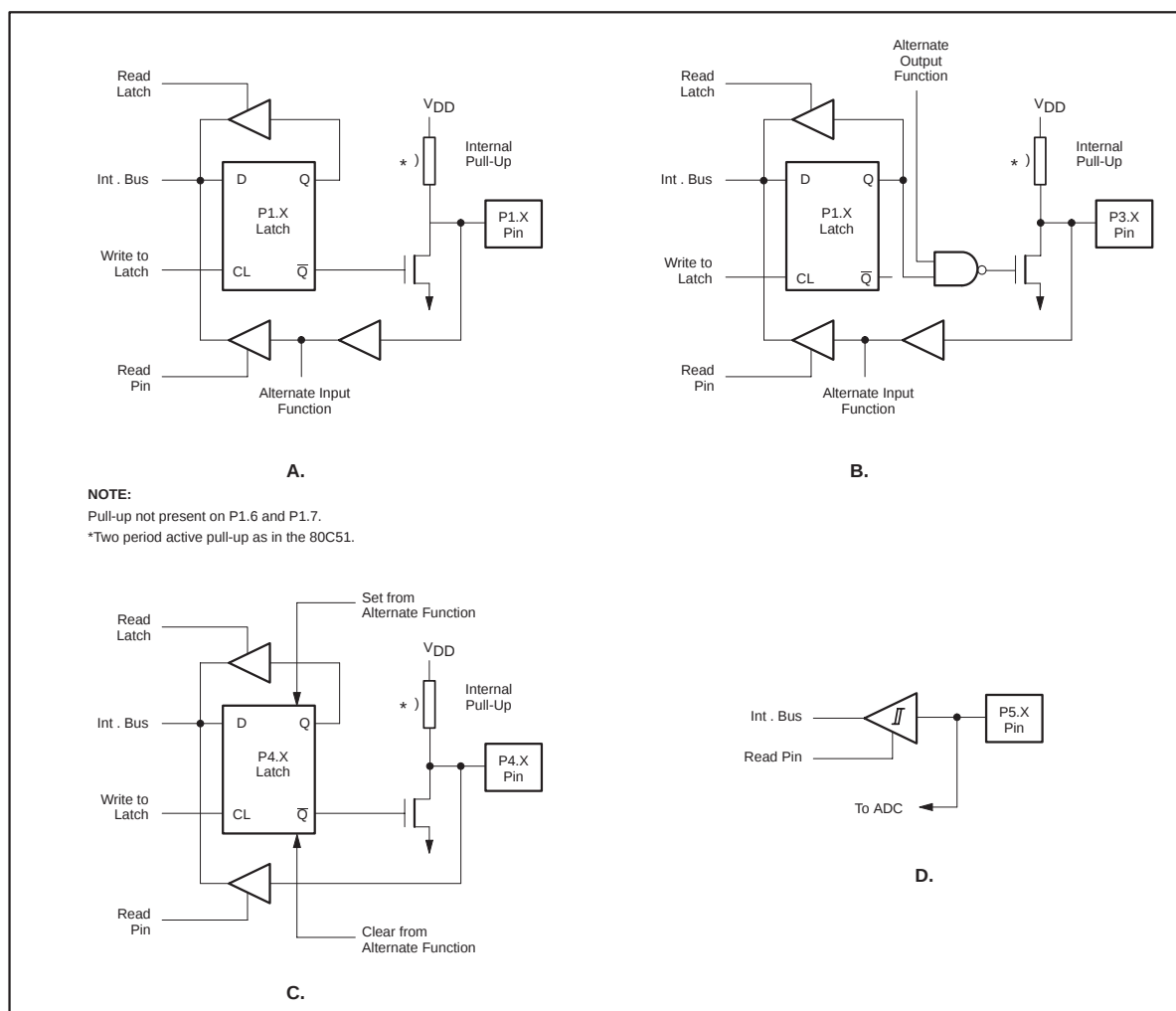
Figure 32. Port Bit Latches and I/O Buffers
