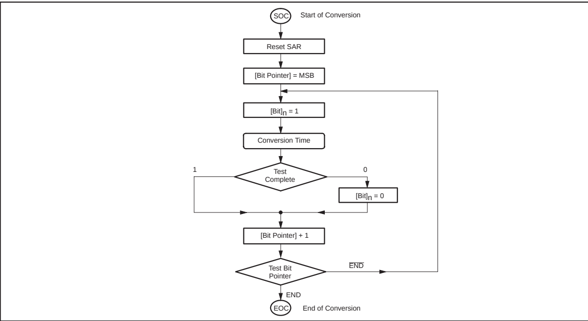
Figure 36. A/D Conversion Flowchart
