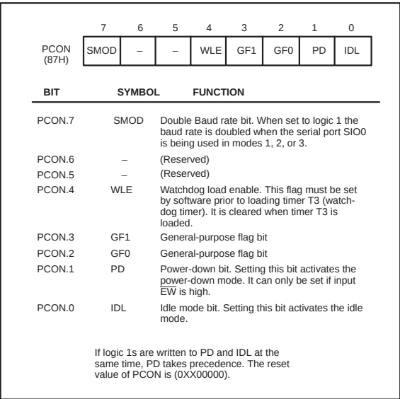
Figure 41. Power Control Register (PCON)
