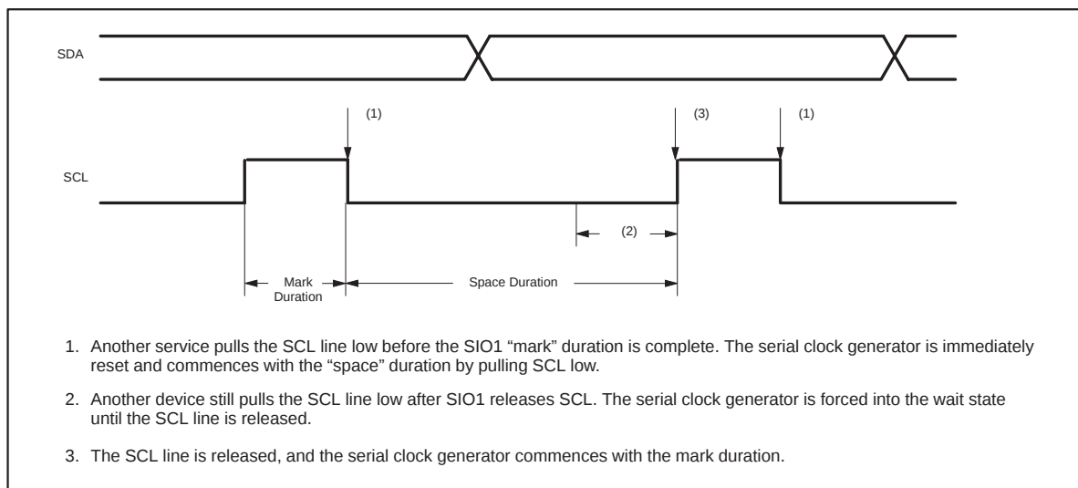
Figure 14. Serial Clock Synchronization
