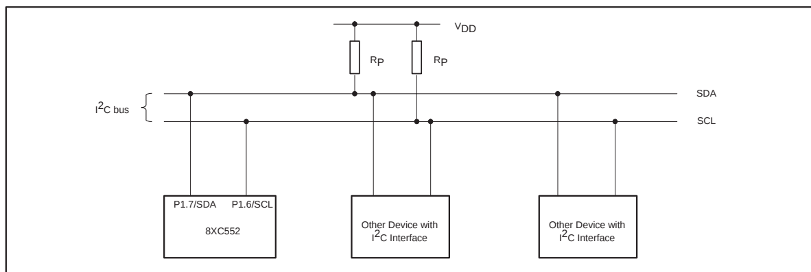
Figure 10. Typical I²C Bus Configuration
