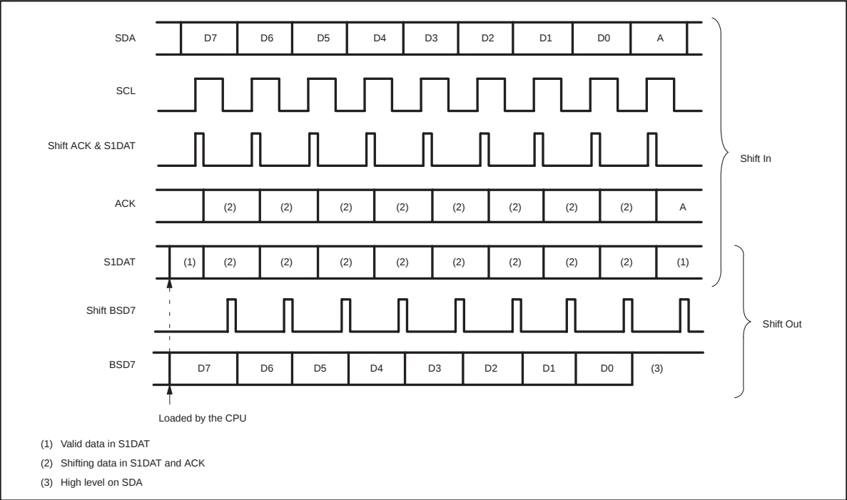
Figure 16. Shift-in and Shift-out Timing
