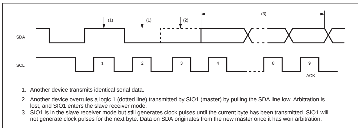
Figure 13. Arbitration Procedure
