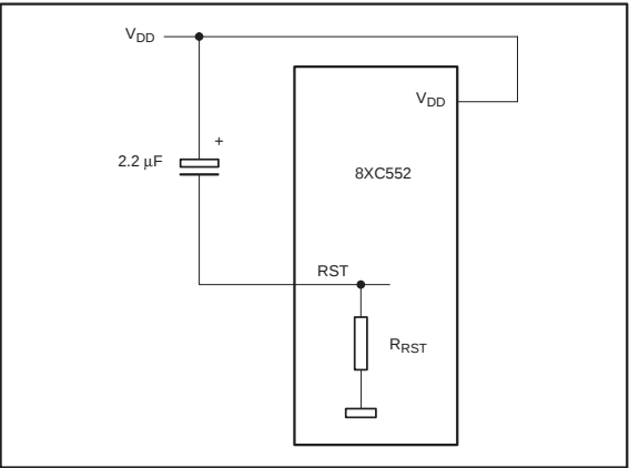
Figure 26. Power-On Reset
