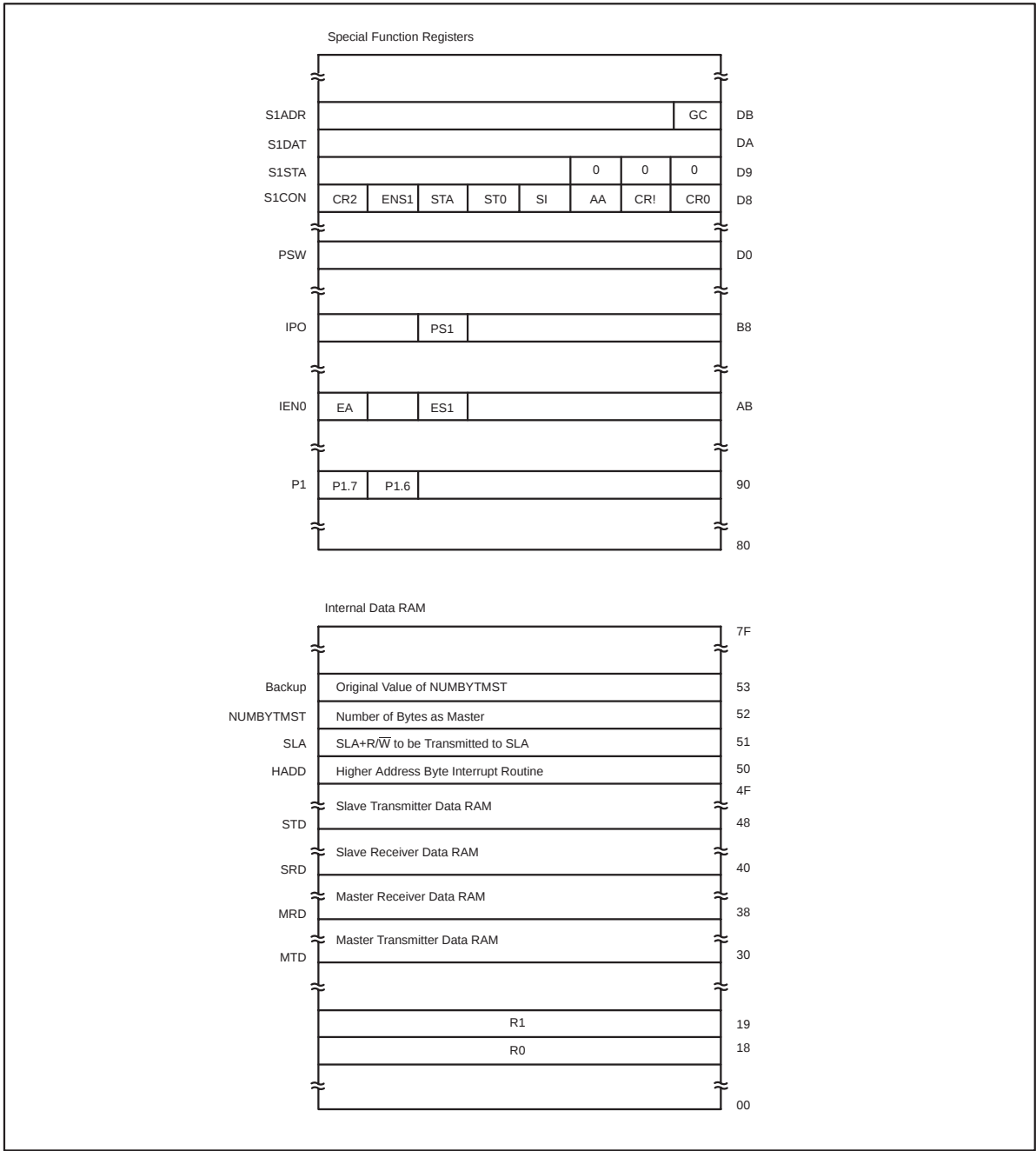
Figure 24. SIO1 Data Memory Map
