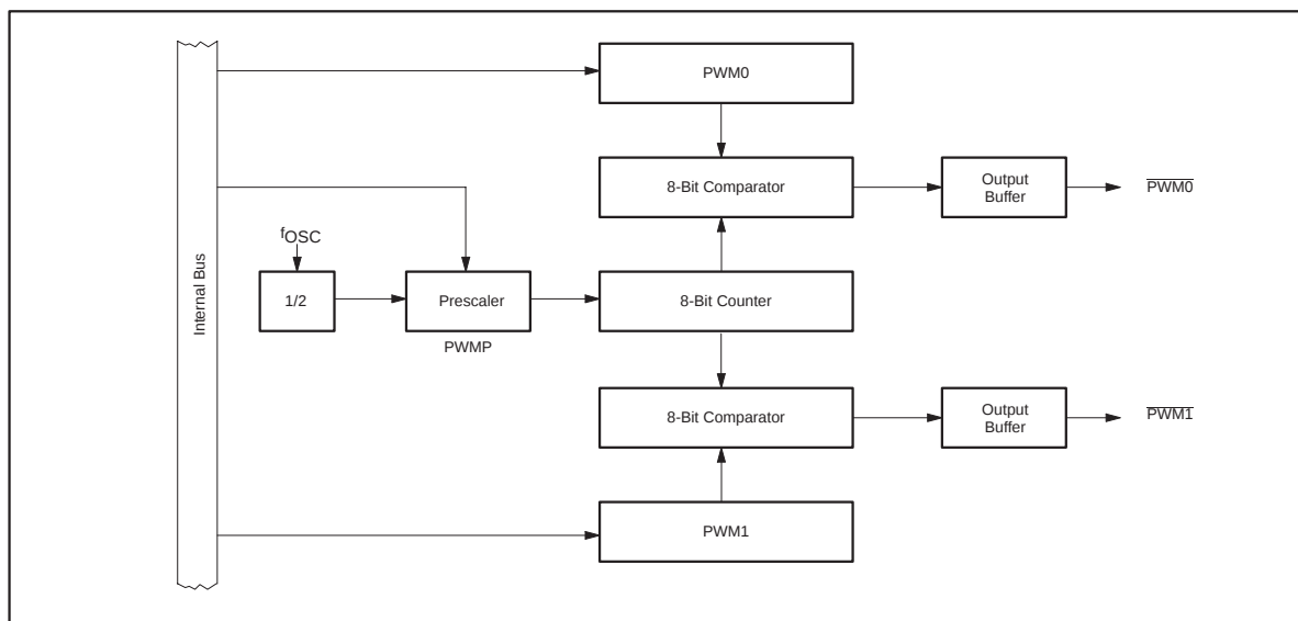
Figure 33. Functional Diagram of Pulse Width Modulated Outputs
