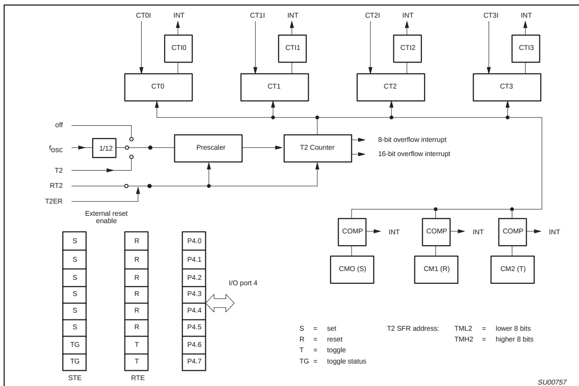
Figure 4. Block Diagram of Timer 2
