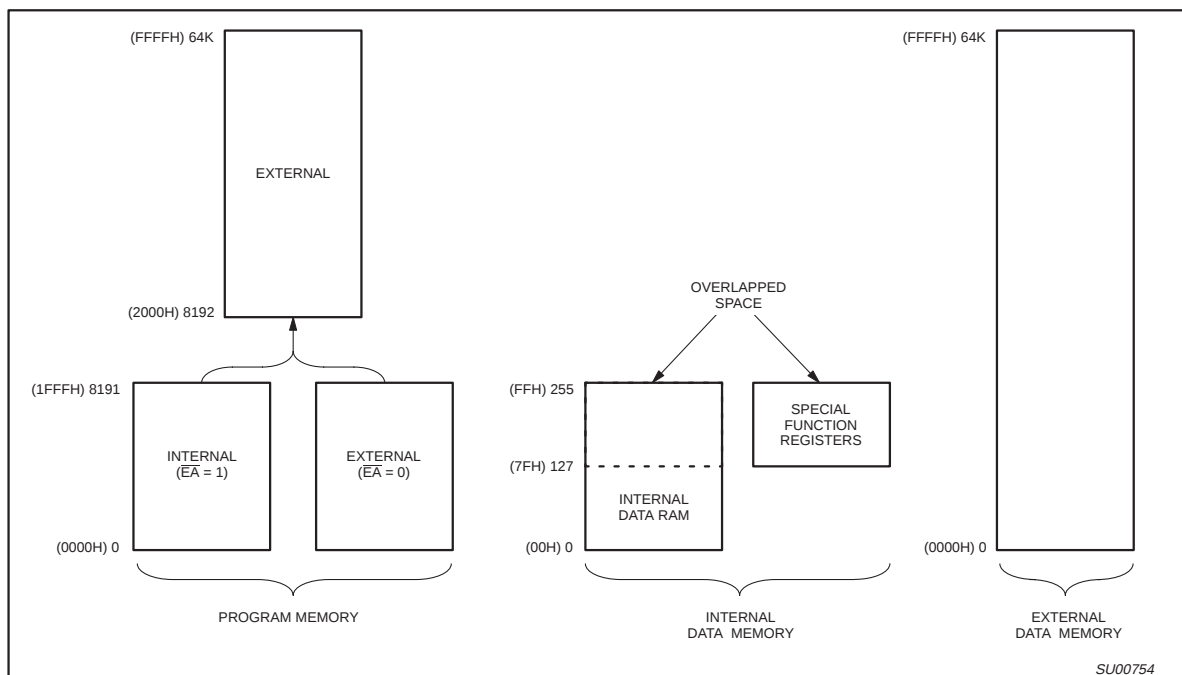
Figure 1. Memory Map
