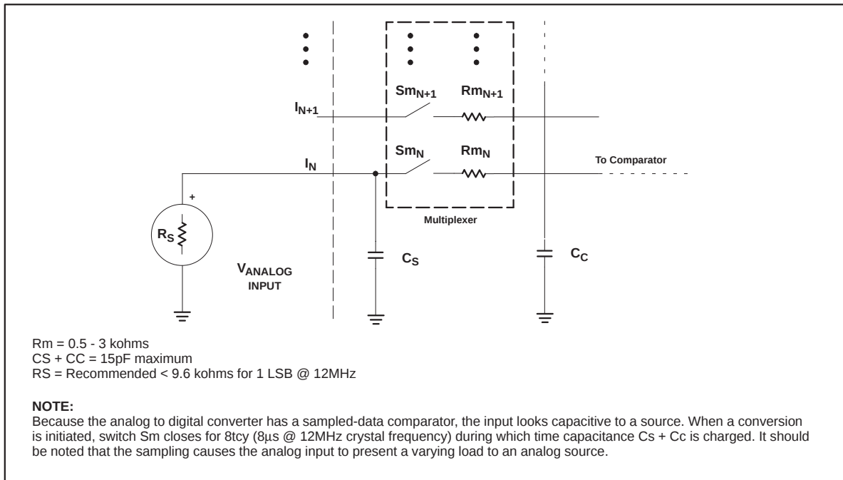
Figure 39. A/D Input: Equivalent Circuit
