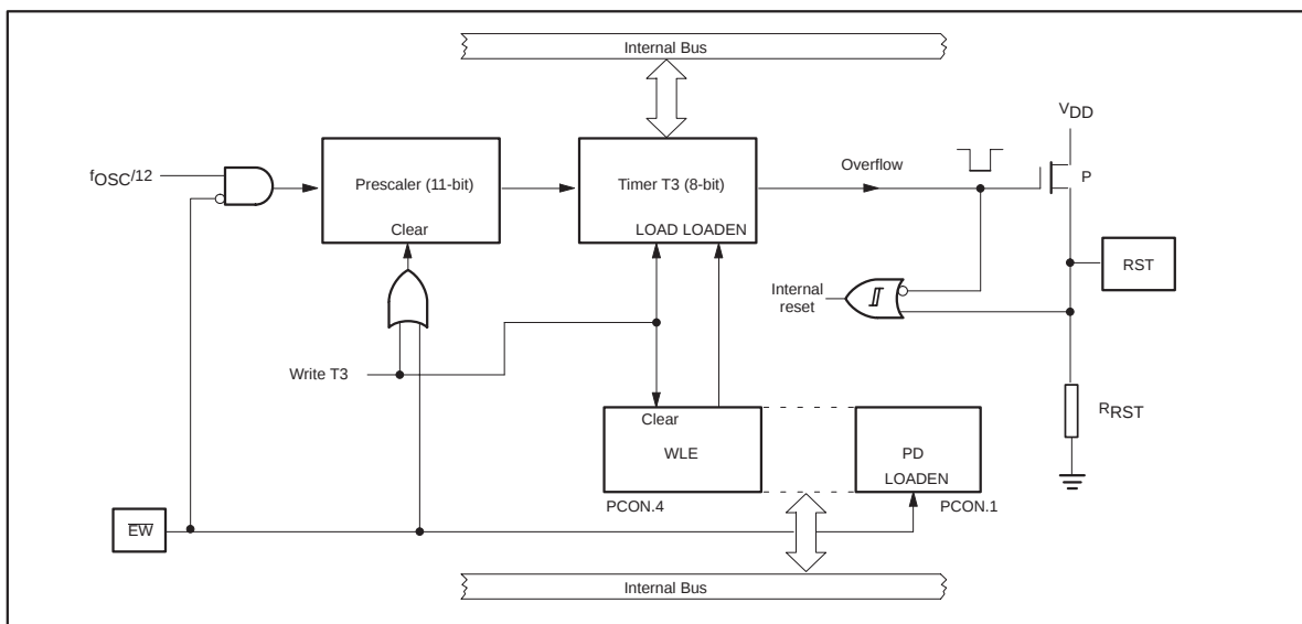
Figure 9. Watchdog Timer
