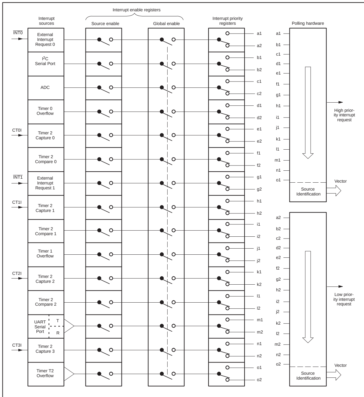
Figure 27. The Interrupt System
