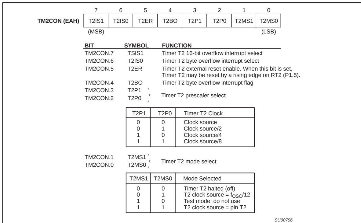
Figure 3. T2 Control Register (TM2CON)
