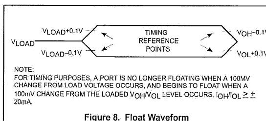
Figure 8. Float Waveform
