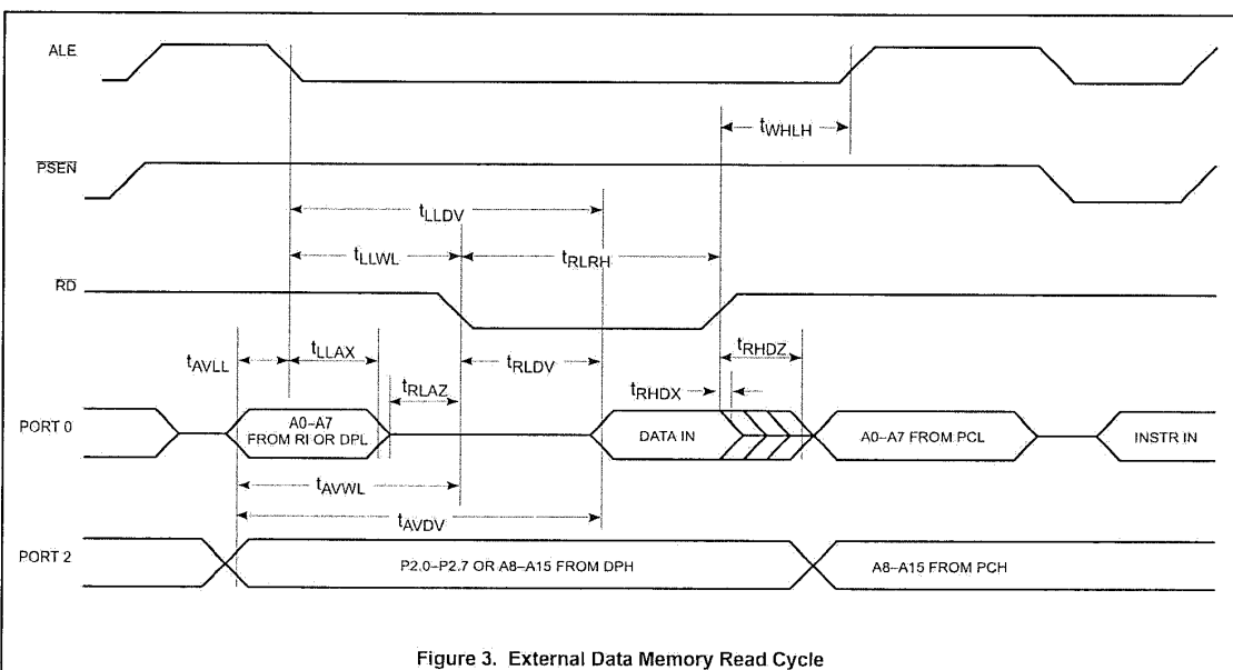
Figure 3. External Data Memory Read Cycle
