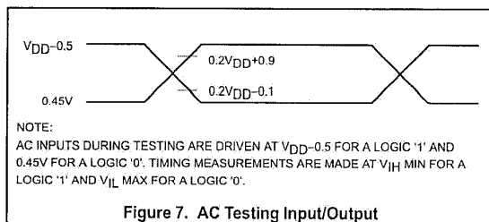
Figure 7. AC Testing Input/Output
