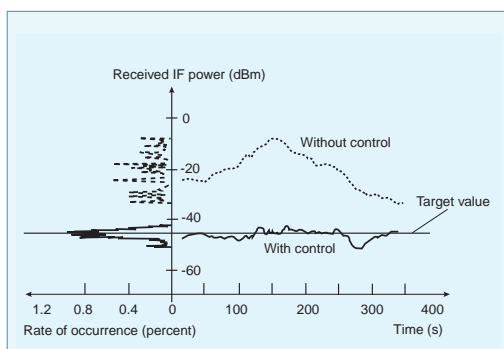
Fig. 4 Performance of open-loop transmission power control.
