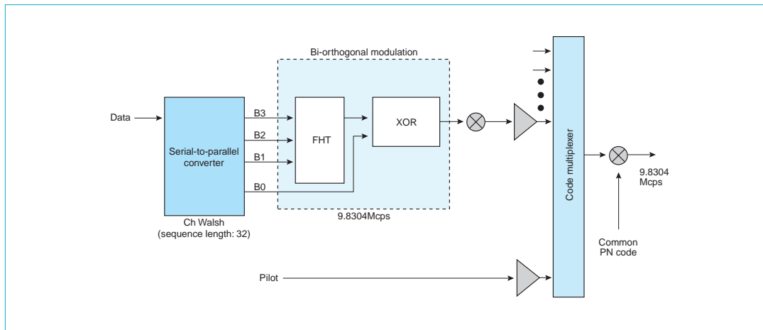
Fig. 2 Block diagram of modulator.
