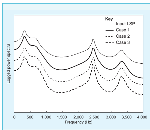
Fig. 3 Examples of spectrum after postfilters.
