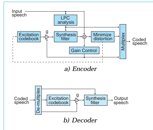
Fig. 1 Block diagram of CELP speech coder.
