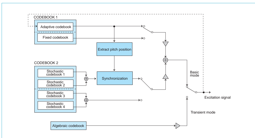
Fig. 2 Excitation signal generation of PPS CELP.
