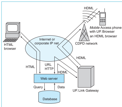
Fig. 3 Description of a Network using UP.Link.
