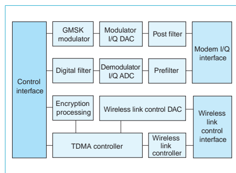
Fig. 3 Baseband IC configuration.
