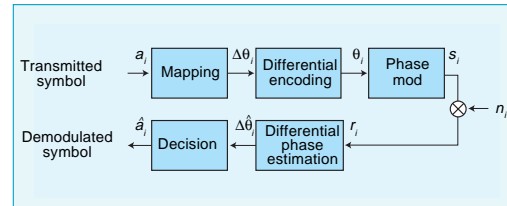
Fig. 1 Communication system model.
