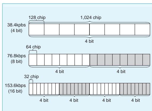
Fig. 1 Variable rate transmission method. Data rates of 307.2 kbps and higher are achieved by multiplexing several of the signals shown.
