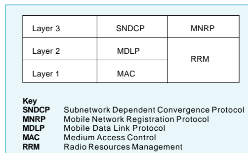
Fig. 2 OSI reference model.
