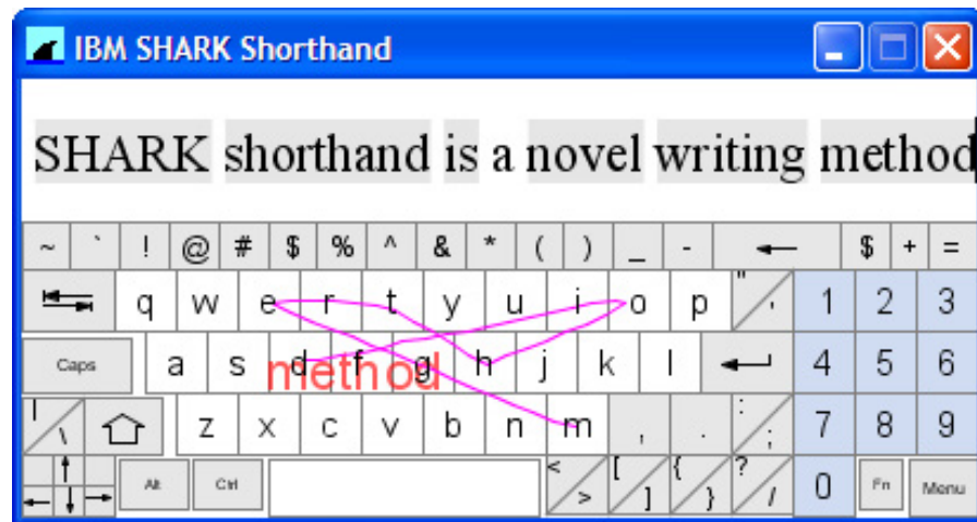
Fig. 3.6 A screenshot of the SHARK word-gesture keyboard in 2005: the gesture represents the word method based on a QWERTY layout.
