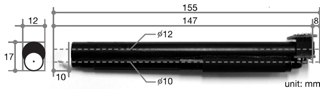
Figure 4: The design of PhantomPen.
