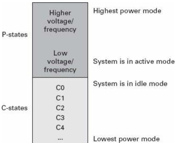
Figure 7.4 P-states and C-states
