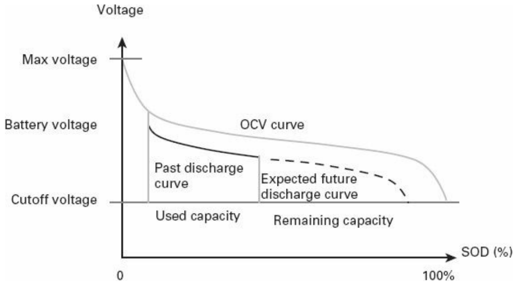
Figure 3.8 Relationship between the OCV and the SOD
