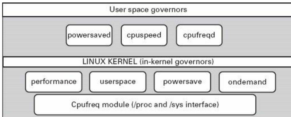
Figure 7.6 Overview of the Linux CPU frequency subsystem
