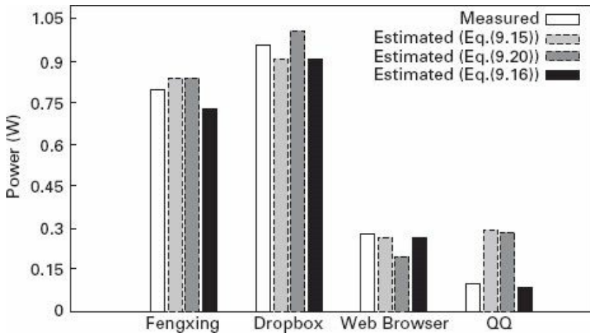
Figure 9.6 Power consumption of four Android applications on a Nexus S
