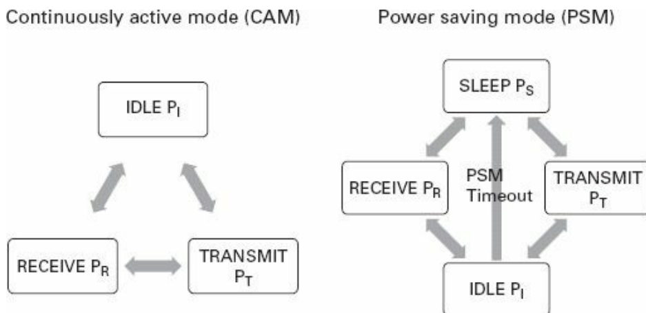
Figure 7.8 Power state machine of the WNI with the PSM Adaptive or the CAM enabled
