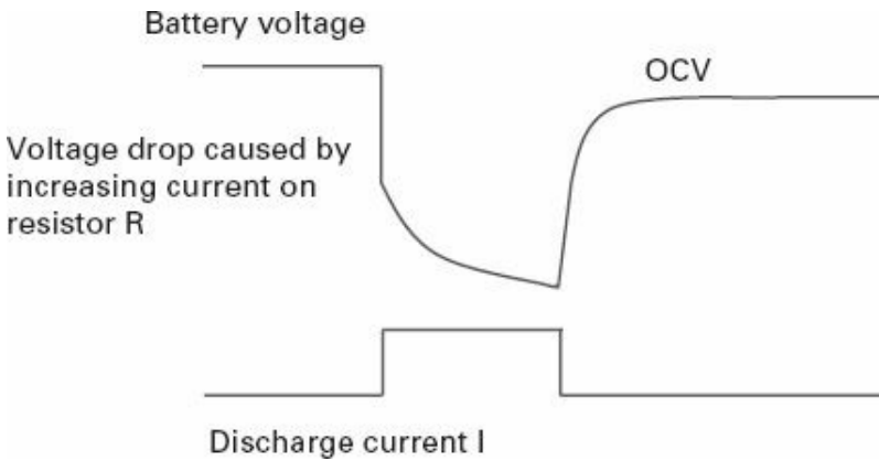
Figure 3.9 The voltage drop in OCV with increasing current
