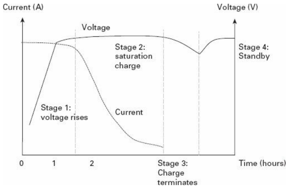
Figure 3.2 Four charging stages
