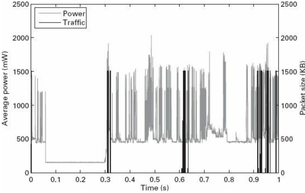
Figure 9.4 Synchronized I/O graph and power consumption on Nexus S
