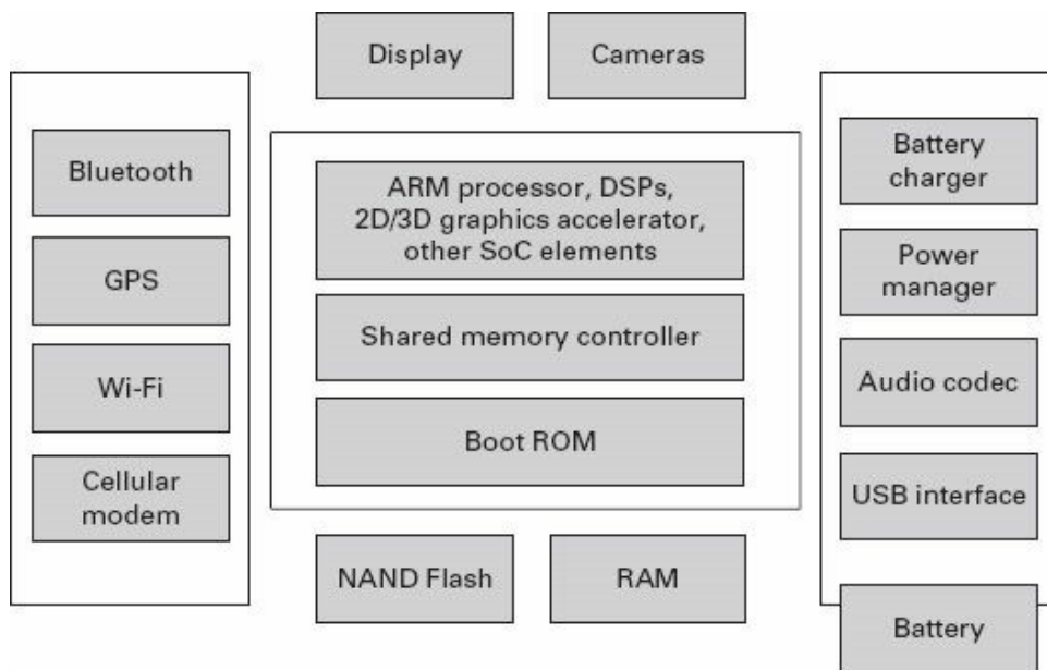
Figure 1.7 Overview of typical smartphone subsystems
