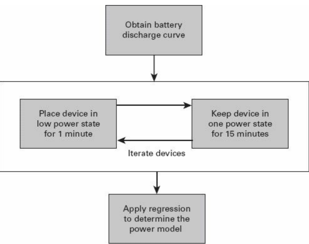
Figure 10.1 Overview of the PowerBooter model
