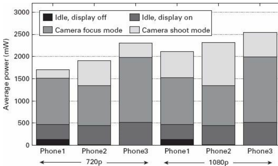
Figure 7.20 Smartphone power consumption during video recording
