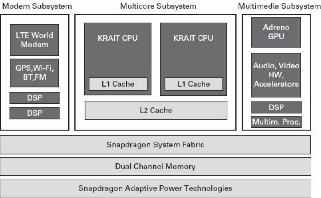
Figure 7.1 Overview of the Snapdragon SoC
