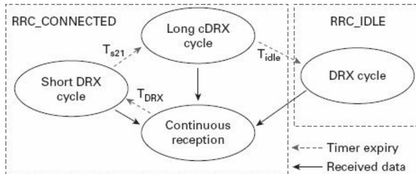
Figure 7.15 LTE state diagram with cDRX/cDTX
