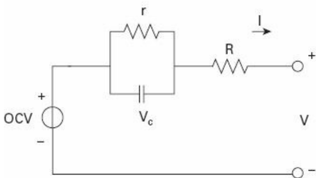
Figure 3.6 The basic Thevenin model
