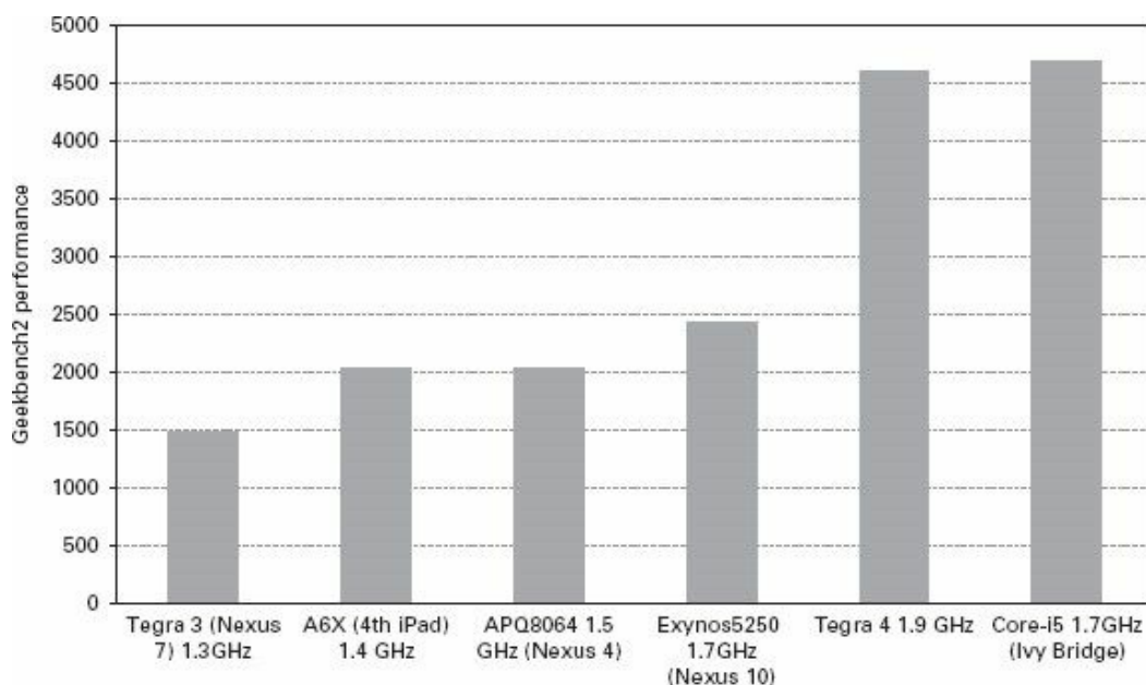
Figure 7.2 Comparison of mobile CPU and SoC performance
