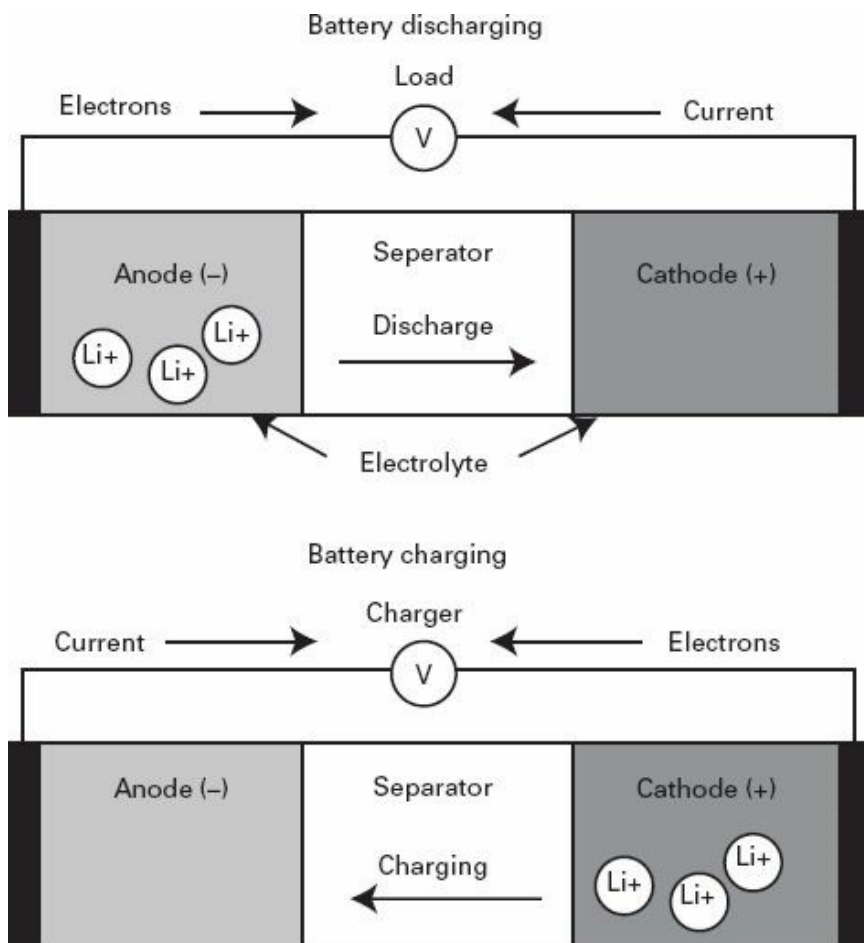
Figure 3.1 Overview of Li-Ion battery charging and discharging
