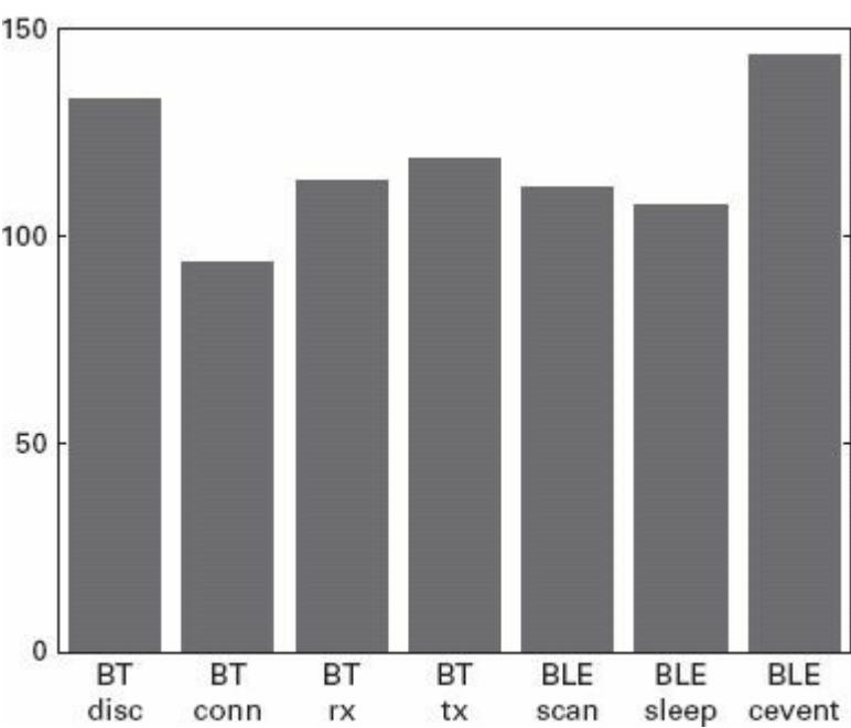
Figure 7.10 Average power of different Bluetooth power modes
