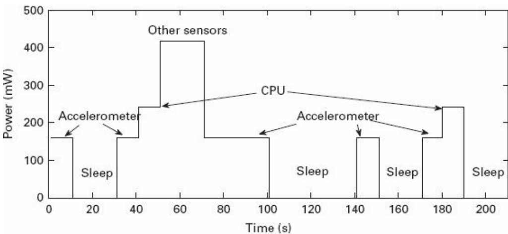
Figure 15.5 Powerdraw of a sample application
