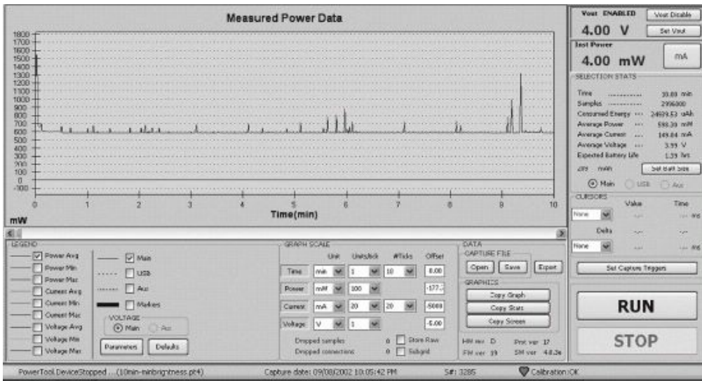
Figure 4.5 A screenshot of the PowerTool software, measuring the energy use of a smartphone while powering it at 4 V
