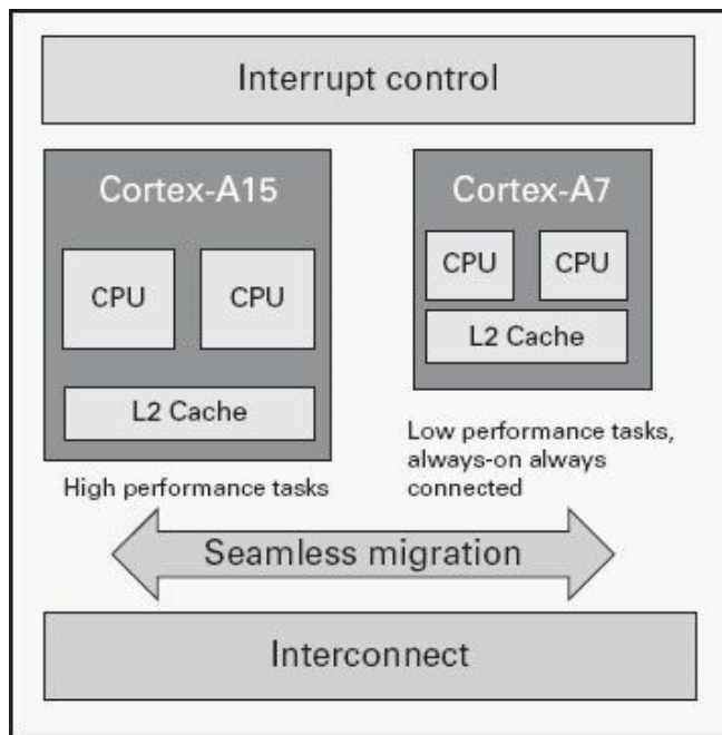
Figure 7.7 Overview of the big.LITTLE architecture
