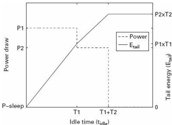
Figure 7.14 Tail energy with 3G having two timers, P1 and P2 corresponding to the power draw in the CELL_DCH and CELL_FACH states, respectively
