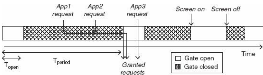
Figure 12.7 NSRM gating mechanism
