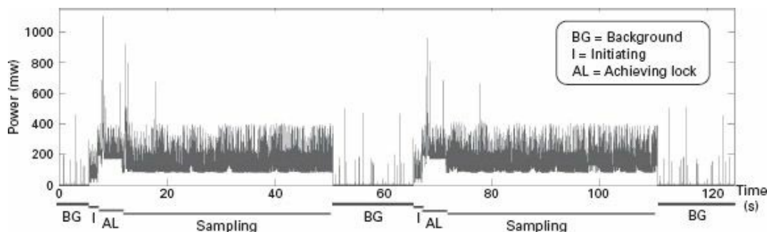
Figure 7.18 Energy measurements from GPS sensor
