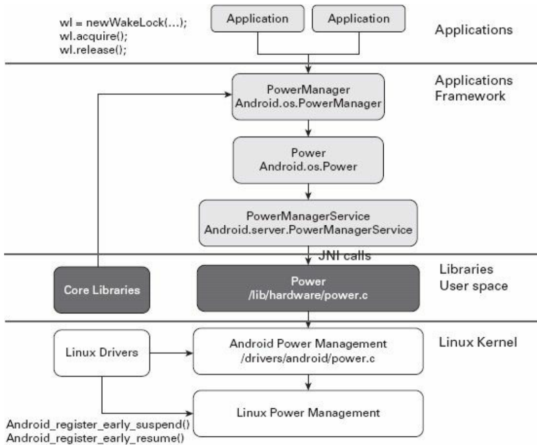
Figure 8.4 The Android power-management system
