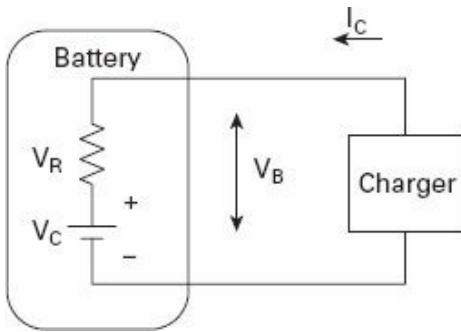
Figure 3.3 Charger circuit
