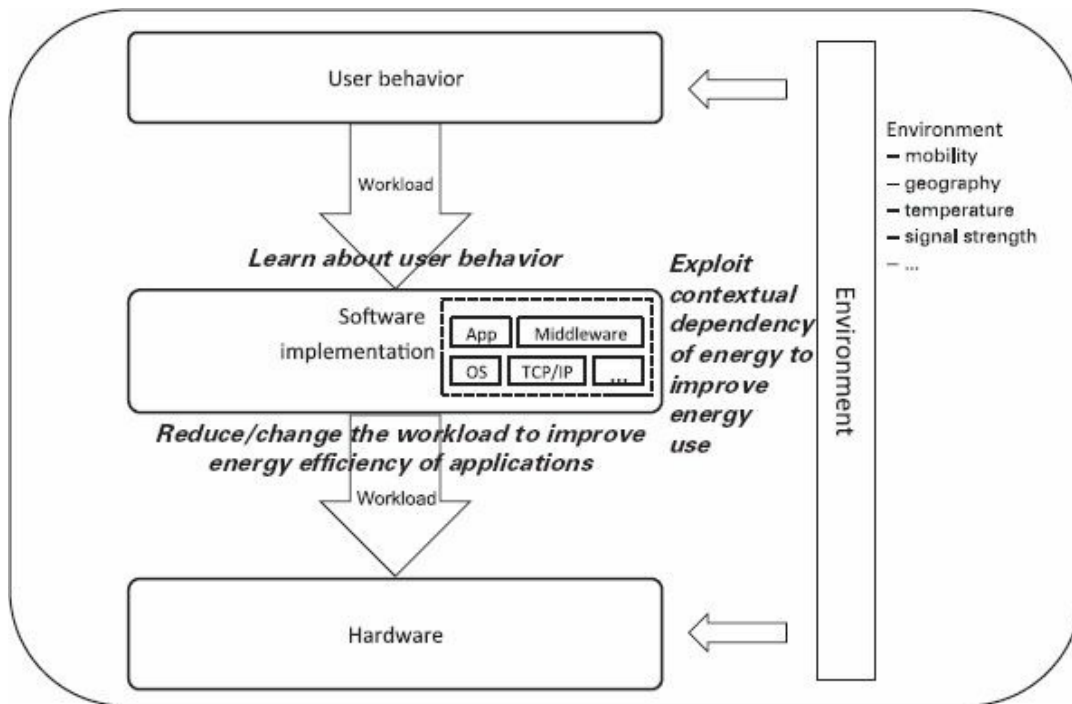
Figure 11.1 How to further reduce the energy expenditure of applications
