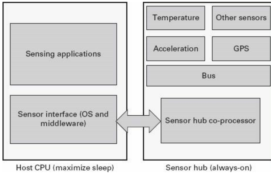
Figure 7.19 Overview of a sensor hub
