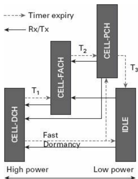
Figure 7.12 3G state transitions and power consumption
