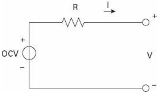
Figure 3.5 The basic Rint model
