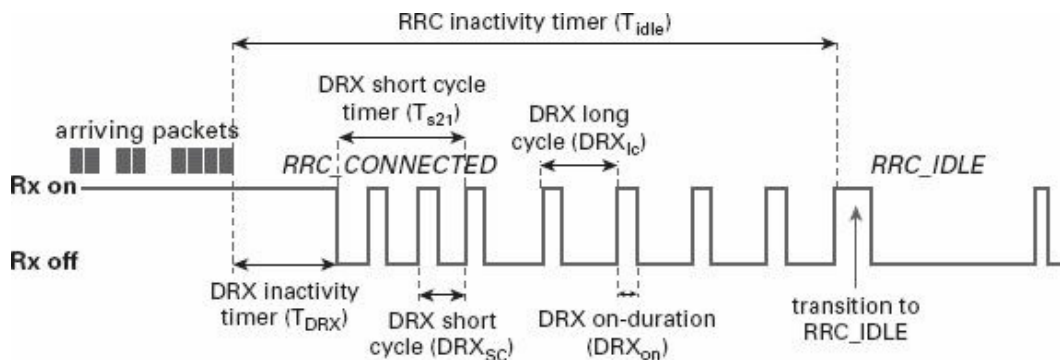
Figure 7.16 Timers and radio activity in cDRX of LTE
