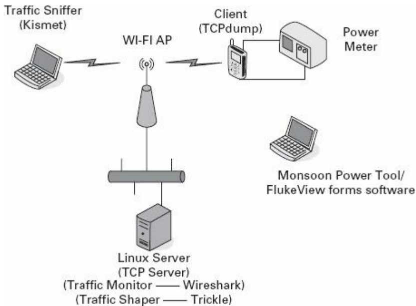
Figure 9.5 Experimental setup
