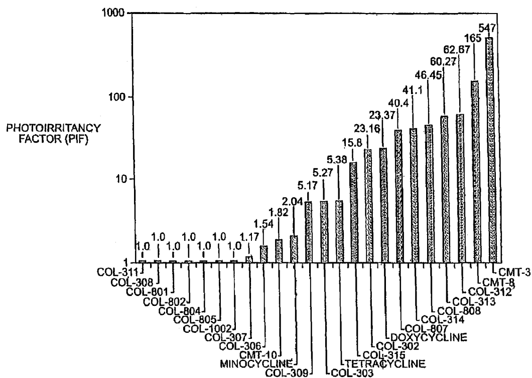
FIG. 1 PHOTOTOXICITY INDEX
