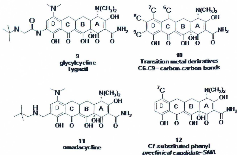
Figure 7. Third-generation tetracyclines.
