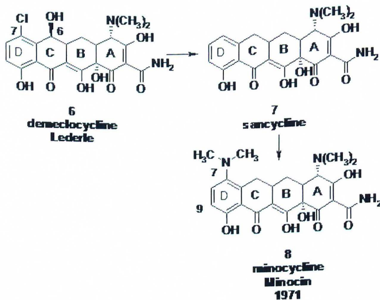
Figure 5. Semisynthesis routes for the second-generation tetracyclines chosen by the Chas. Pfizer Co. for doxycycline (5), and Lederle Laboratories for minocycline (8). The chemical name is followed by the year approved by the FDA.
