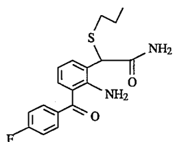
Compound 1 2-Amino-3-(4-fluorobenzoyl)-alpha-(n-propylthio)-phenylacetamide
