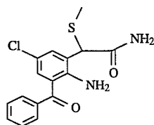
Compound 4 2-Amino-3-benzoyl-5-chloro-alpha-(methylthio)-phenylacetamide
