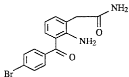
Compound 15 2-Amino-3-(4-bromobenzoyl)-phenylacetamide
