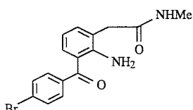
Compound 16 2-Amino-3-(4-bromobenzoyl)-N-methyl-phenylacetamide
