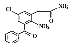
Compound 10 2-Amino-3-benzoyl-5-chlorophenylacetamide
