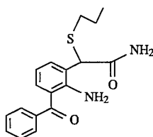
Compound 2 2-Amino-3-benzoyl-alpha-(n-propylthio)-phenylacetamide
