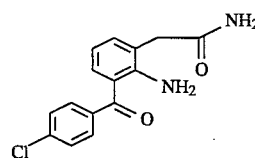
Compound 9 2-Amino-3-(4-chlorobenzoyl)-phenylacetamide
