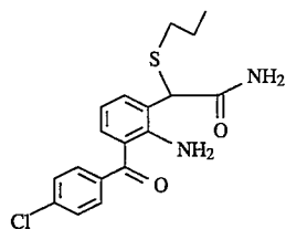
Compound 3 2-Amino-3-(4-chlorobenzoyl)-alpha-(n-propylthio)-phenylacetamide
