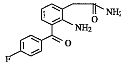
Compound 7 2-Amino-3-(4-fluorobenzoyl)-phenylacetamide
