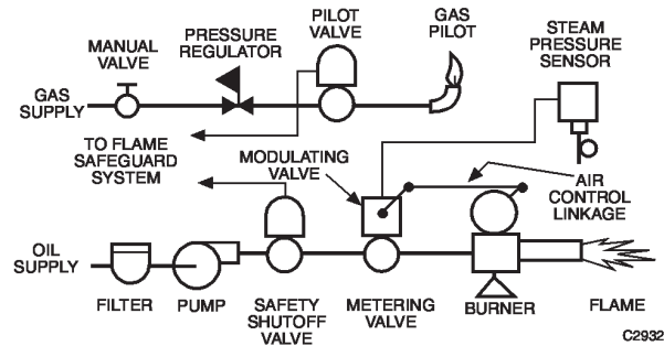
Fig. 44. Combustion Control for Rotary Oil Burner.
