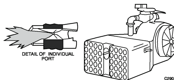
Fig. 43. Multiport Forced-Draft Gas Burner.
