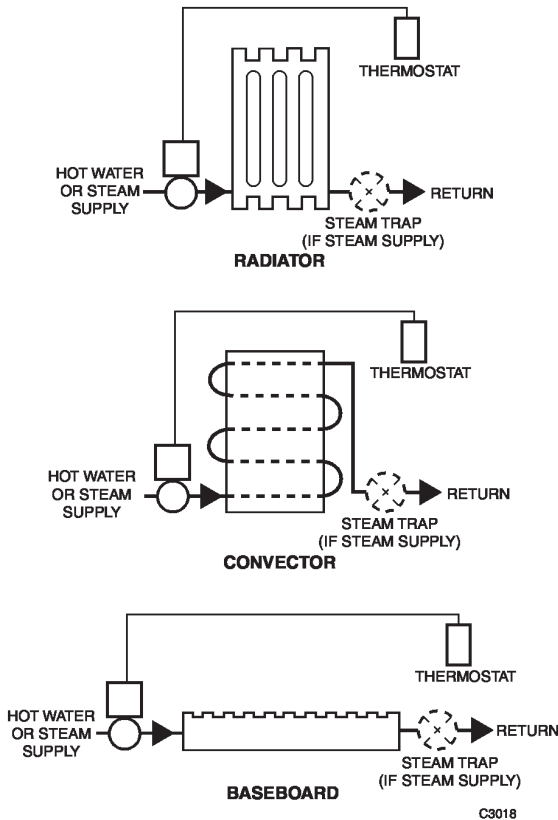
Fig. 12. Natural Convection Units.
