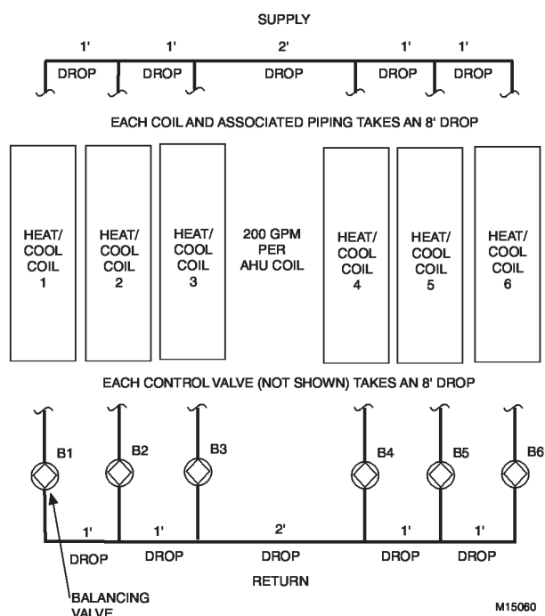
Fig. 73 Typical Example Loads.
