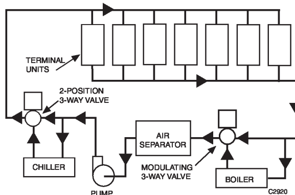
Fig. 99. Two-Pipe Dual-Temperature System.
