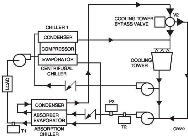
Fig. 22. Schematic of Combination Absorption/Centrifugal Chiller System Water Piping.
