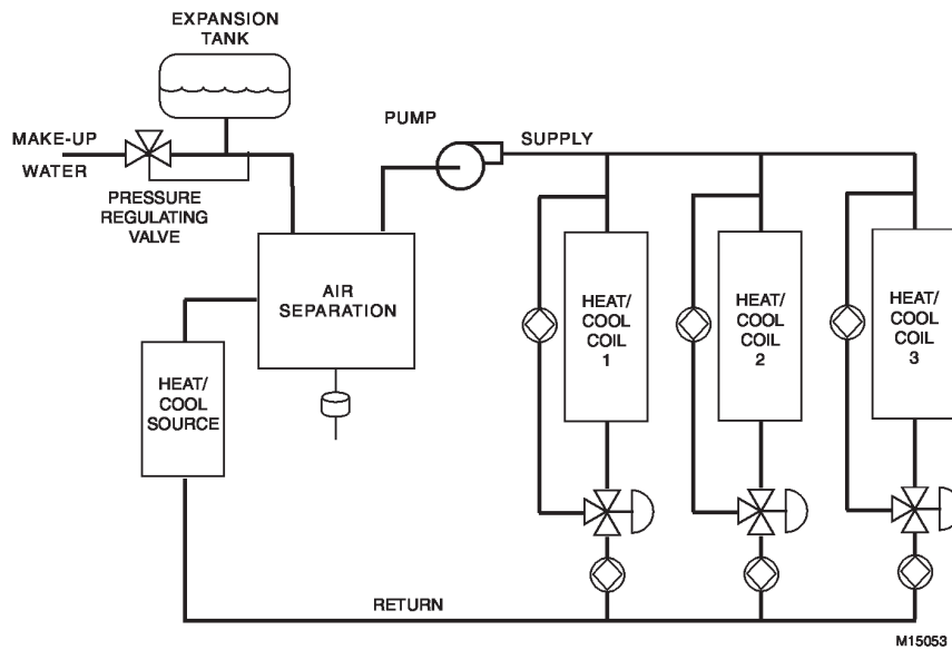
Fig. 51. Typical Water Distribution System.
