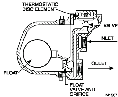
Fig. 104. Float and Thermostatic Trap.
