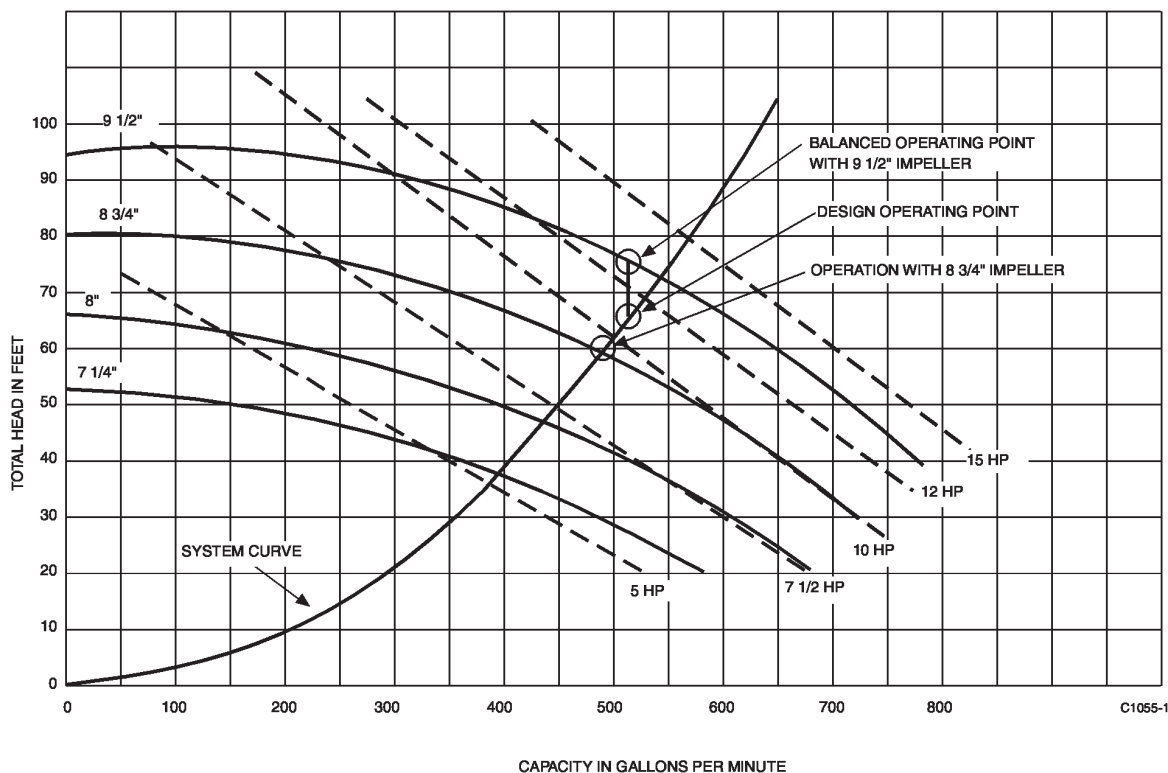
Fig. 57. Matching Pump to System.
