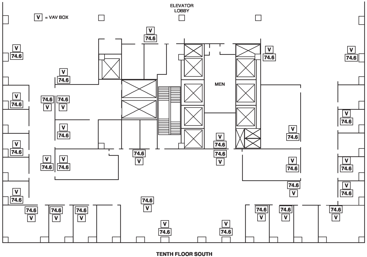
Fig. 39. ATU System Floor Plan Graphic
