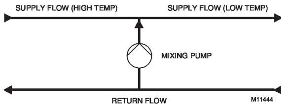
Fig. 128. Principle Of A Mixing Station.
