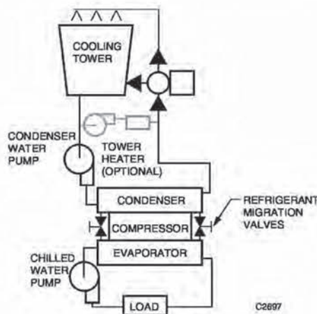
Fig. 33. Free Cooling Using Refrigerant Vapor Migration.
