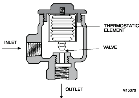
Fig. 103. Thermostatic Trap.
