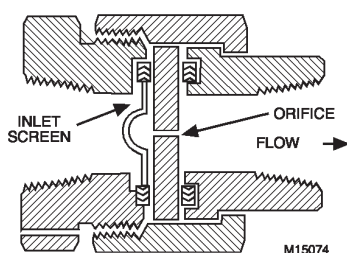
Fig. 107. Orifice Trap.
