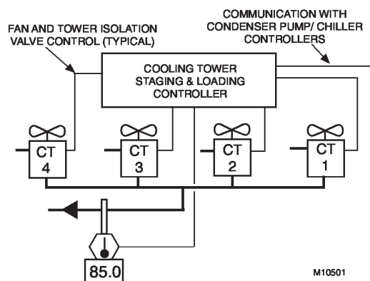
Fig. 18. Digital control of Sequenced Cooling Towers.
