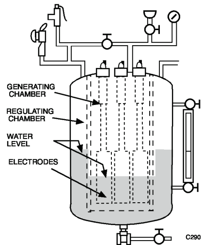
Fig. 40. Electrode Steam boiler.
