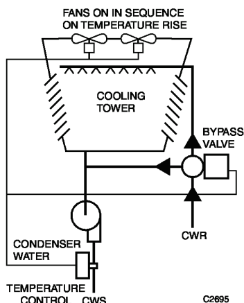
Fig. 27. Cooling Tower Control.
