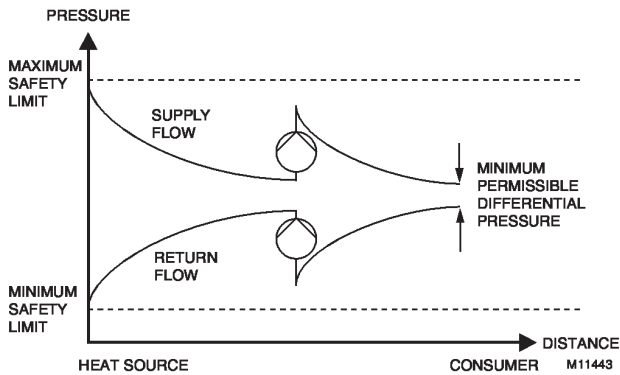
Fig. 127. Network Pressure Profile.
