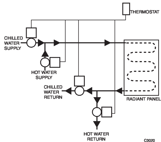
Fig. 14. Heating/Cooling Radiant Panel.
