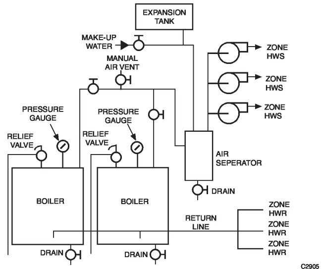
Fig. 47. Typical Piping for Multiple-Zone Heating System.
