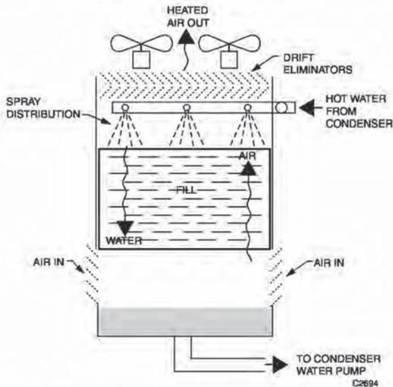
Fig. 25. Cooling Tower, Showing Water-Air Counterflow.
