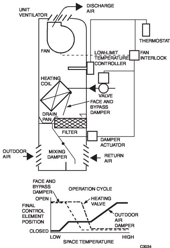
Fig. 25. Unit Ventilator Cycle II Control (Face and Bypass Model).
