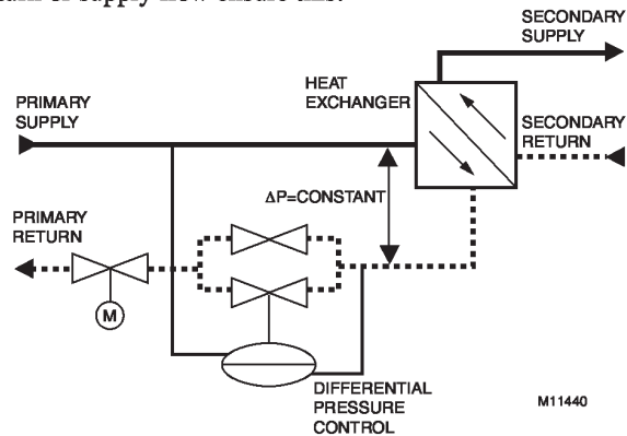
Fig. 132. Primary Side of Indirect Heat Transfer Substation.
