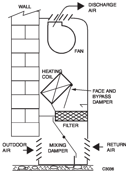
Fig. 21. Draw-Through Unit Ventilator.
