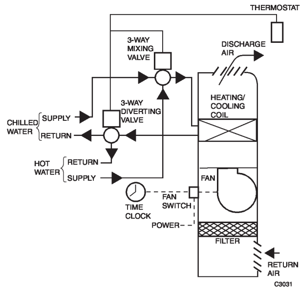
Fig. 35. Four-Pipe Heating/Cooling Fan Coil Unit.
