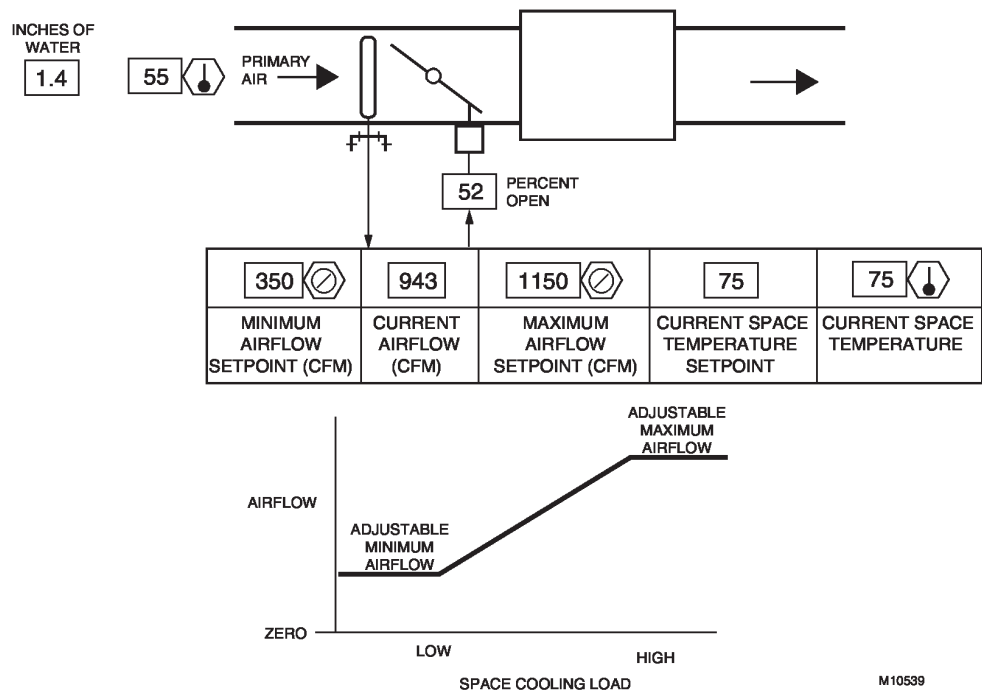
Fig. 5. Variable Air Volume Single-Duct Air Terminal Unit.
