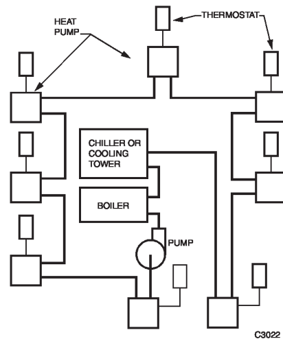
Fig. 37. Heat Pump Closed-Loop System.
