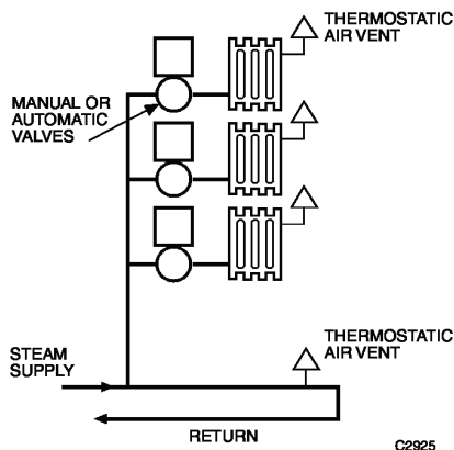
Fig. 110. One-Pipe System.
