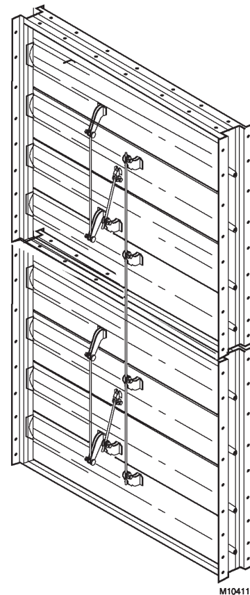
Fig. 15. Drive Blade Linkage for Vertical Multiple Section Damper Assembly.
