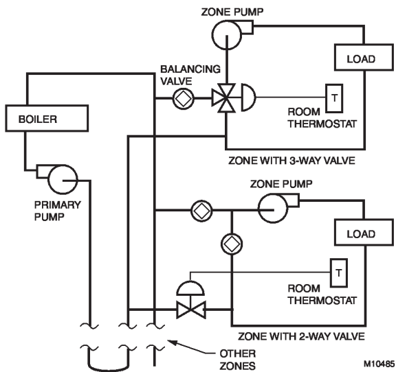
Fig. 88. Piping for Primary-Secondary Pumping.
