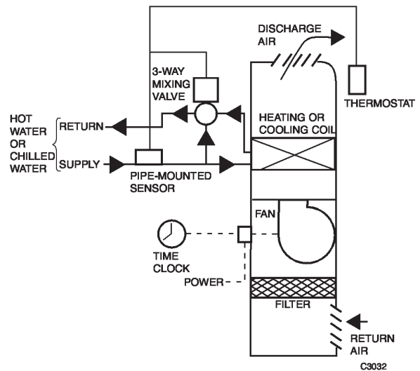
Fig. 32. Two-Pipe Heating/Cooling Fan Coil Unit.
