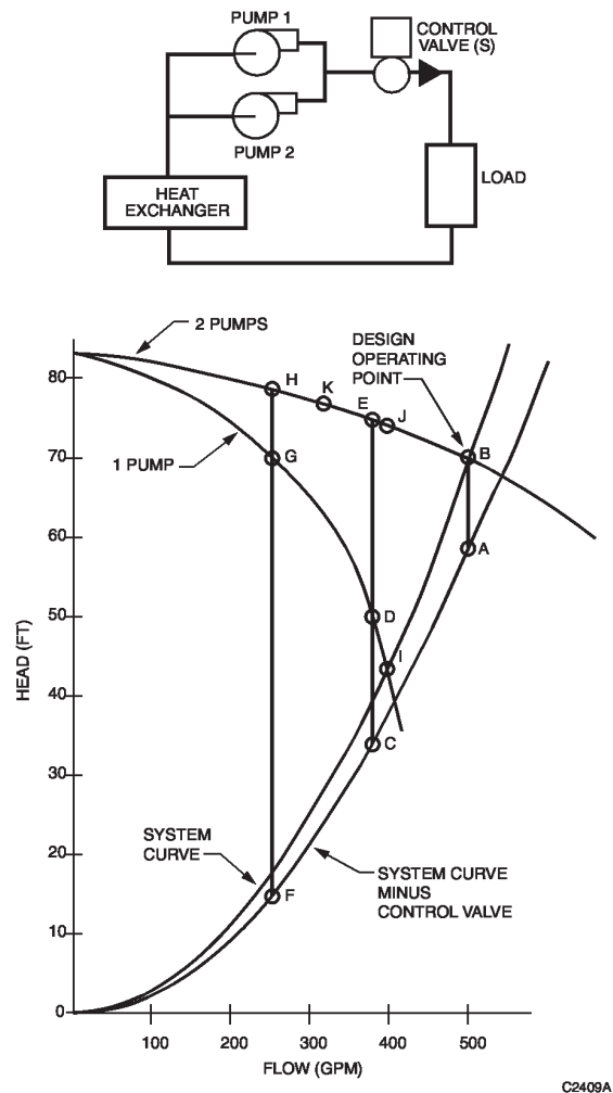
Fig. 66. System Operation with Two Pumps in Parallel.
