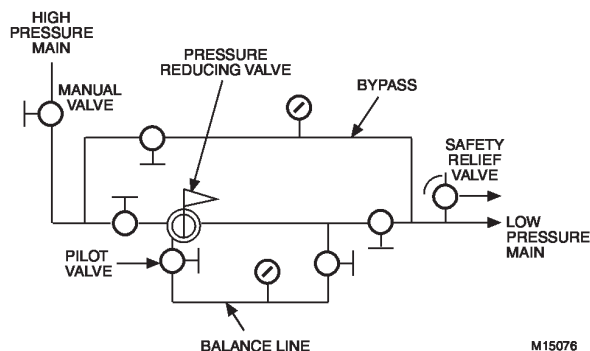
Fig. 109. PRV Station.
