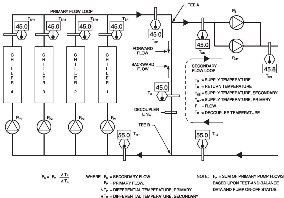
Fig. 16. Multiple Equal Sized Chillers Control Graphic.
