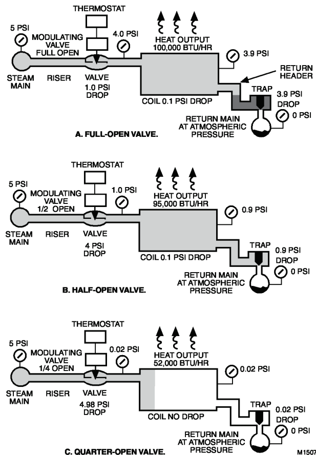
Fig. 114. Control Results with Oversized Valve.
