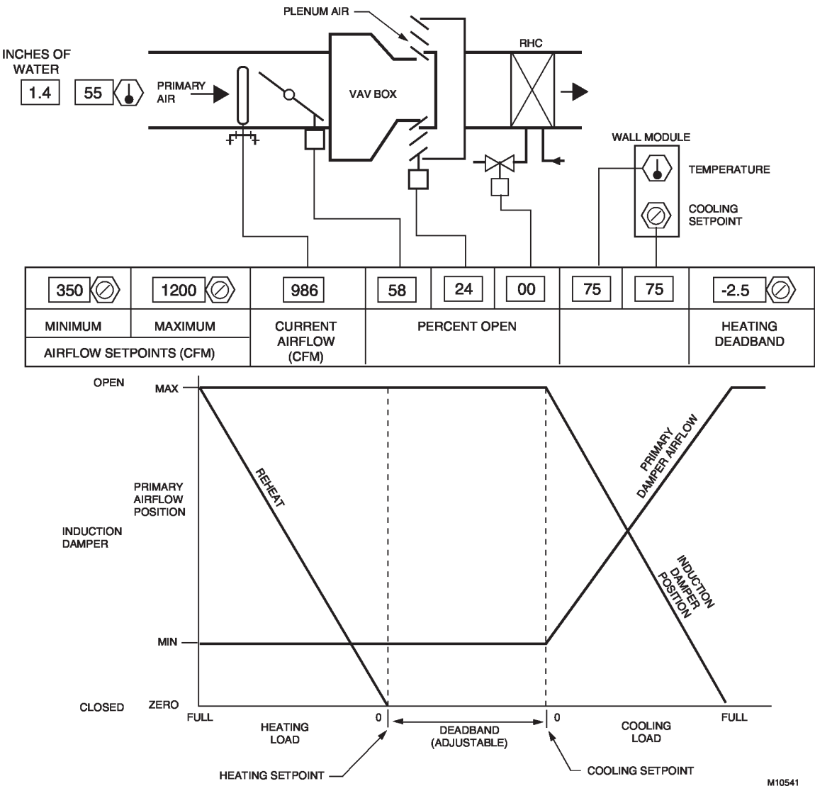
Fig. 7. Induction VAV Air Terminal Unit.
