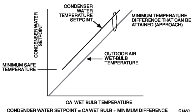
Fig. 28. Condenser Water Temperature Reset from Outdoor Wet-Bulb.
