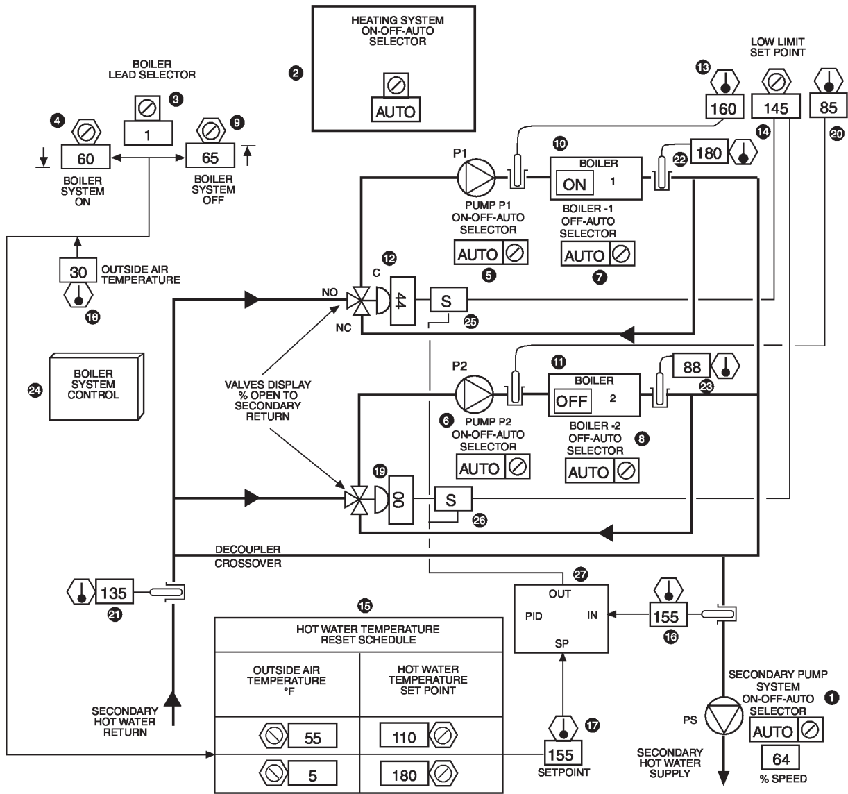
Fig. 48. Dual Boiler Plant Control Graphic
