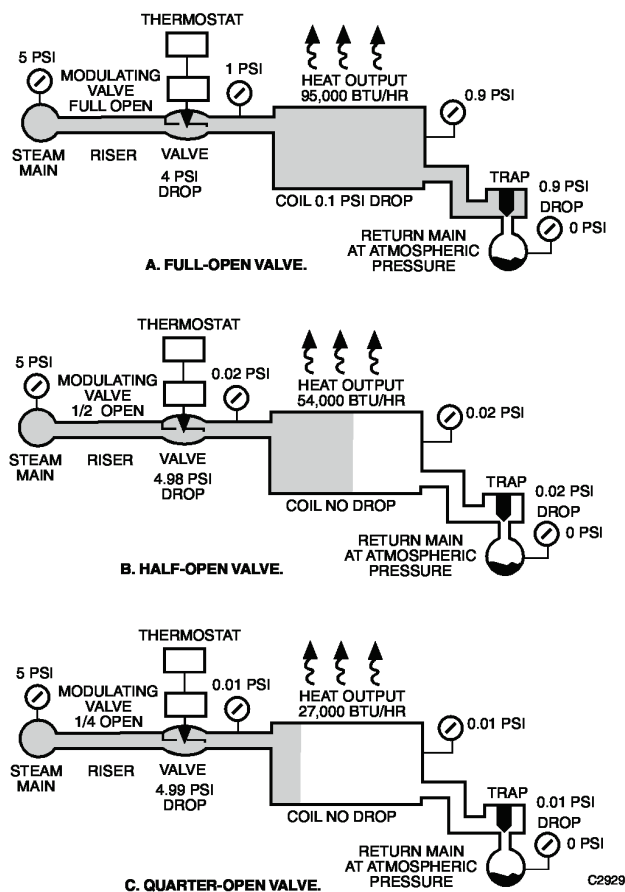
Fig. 115. Control Results with Correctly Sized Valve.
