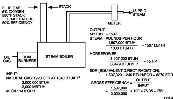
Fig. 41. Boiler Ratings and Efficiency.
