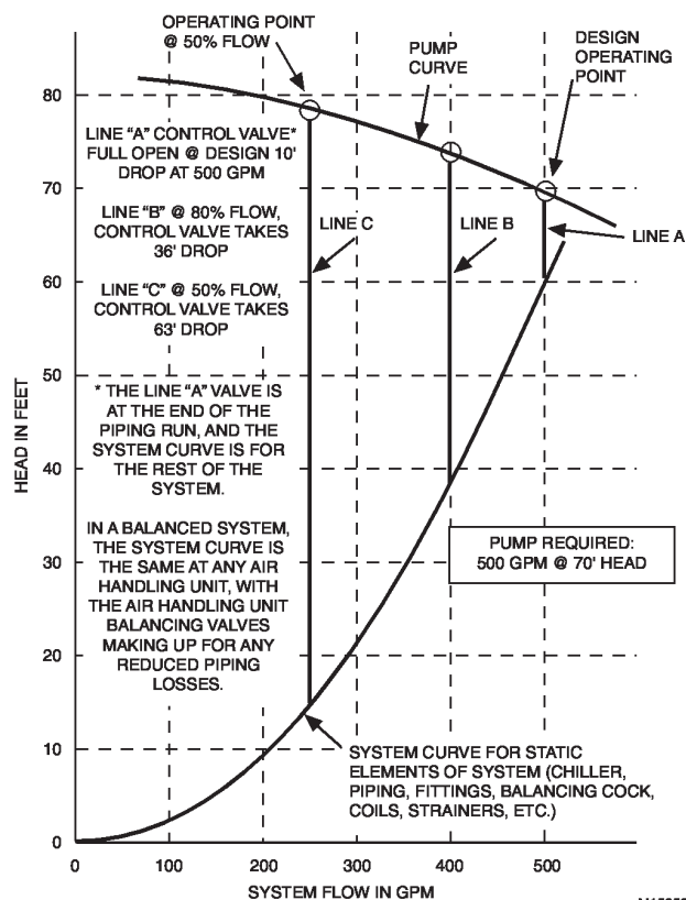
Fig. 58. Pump and System Curves and Control Valves
