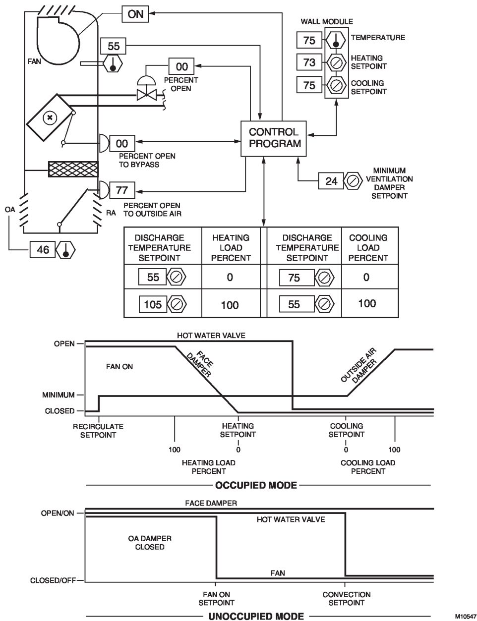
Fig. 28. Cycle II with Enhanced Digital Control.
