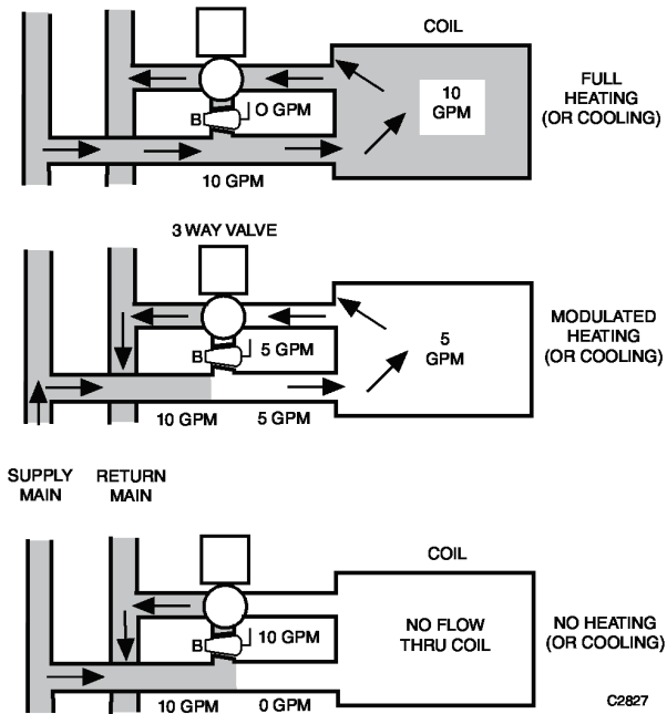
Fig. 72. Three-Way Valve Control—Coil Bypass.
