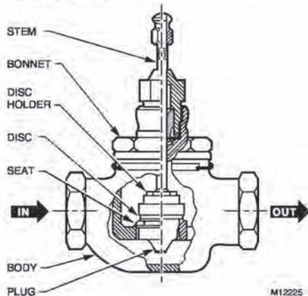
Fig. 1. Globe Valve Components.
