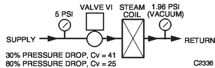
Fig. 19. Linear Valve Steam Application.
