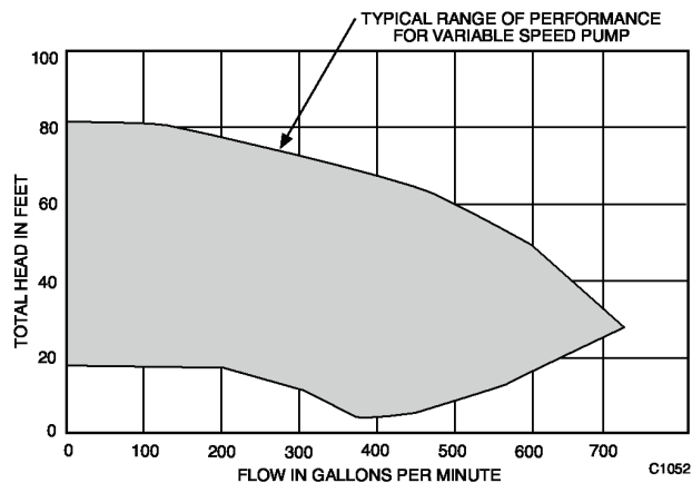
Fig. 60. Typical Variable Speed Pump Performance Range.
