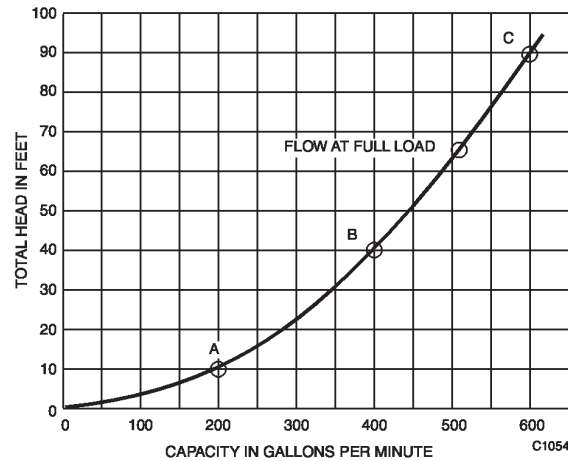
Fig. 56. System Curve for Pump Application.
