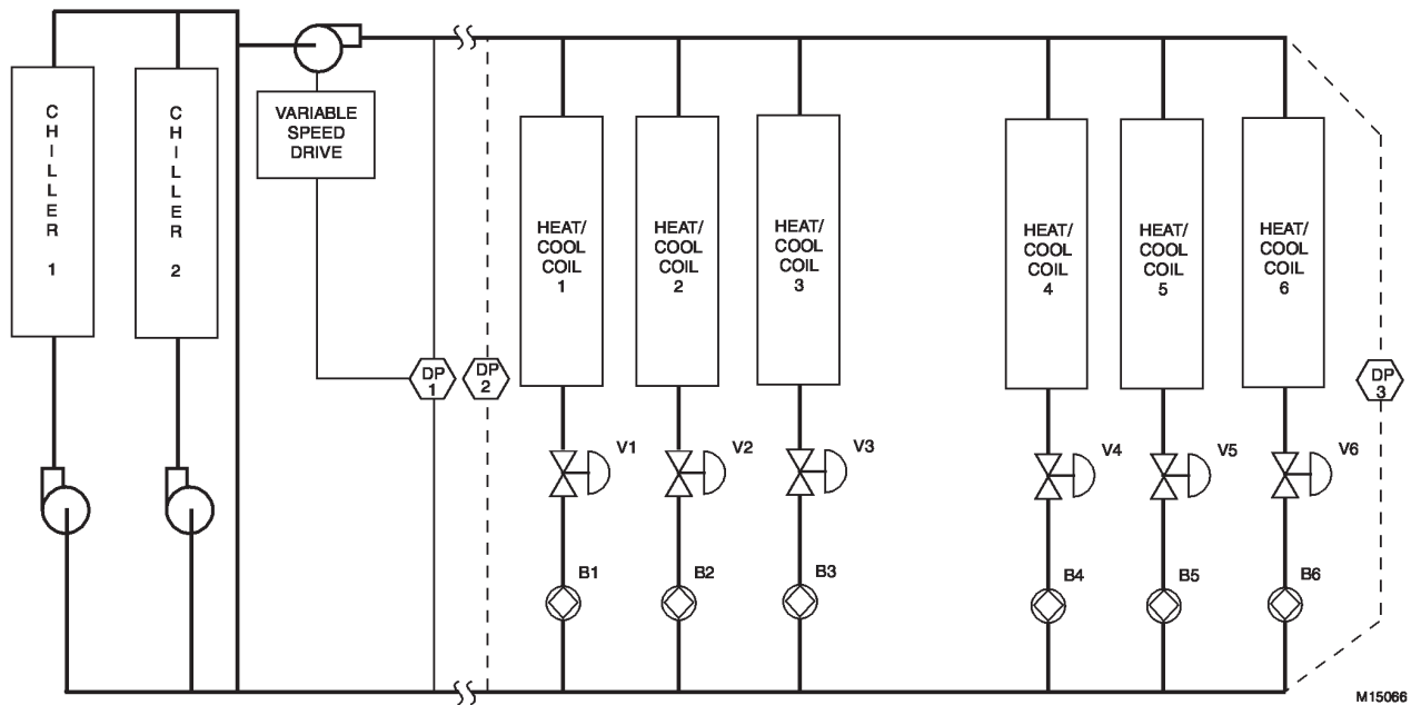
Fig. 79. Variable Speed Pump Control
