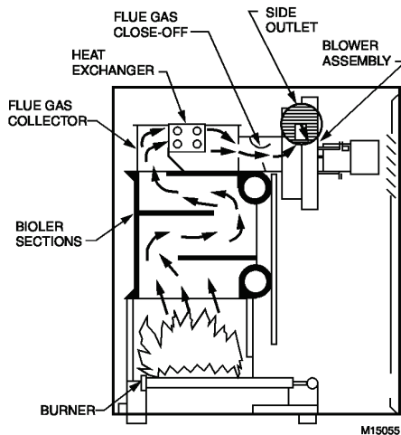
Fig. 39. High Efficiency Modular Boiler.
