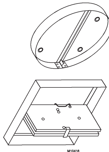
Fig. 12. Ceiling Fire Dampers.
