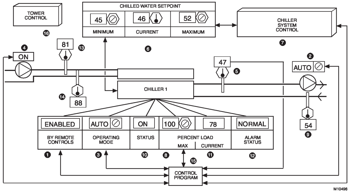
Fig. 9. Single Chiller Control Graphic.
