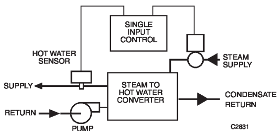
Fig. 83. Constant Temperature Hot Water Converter Control.
