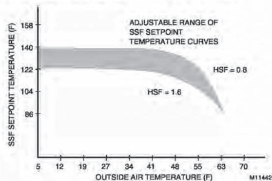
Fig. 143. SSF Temperature Reset Range.
