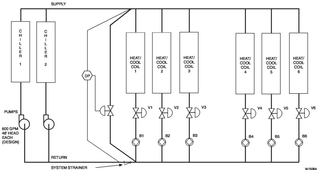
Fig. 77. Dual Pumps, Dual Chillers—Pressure Bypass
