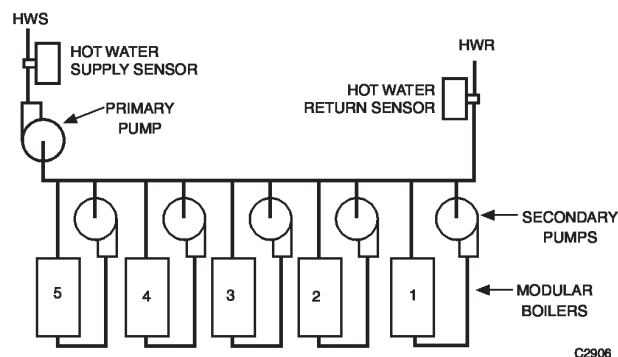
Fig. 50. Typical Primary-Secondary Piping for Modular Boilers.
