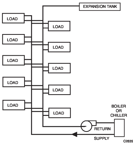
Fig. 87. Two-Pipe Direct-Return System.
