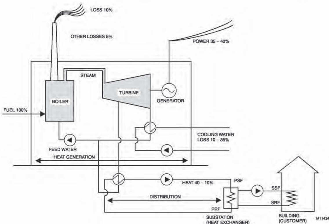
Fig. 126. District Heating Network.
