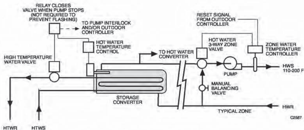
Fig. 124. HTW to HW Multizone Storage Converter.
