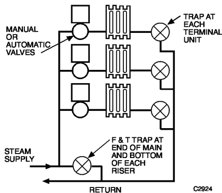
Fig. 111. Two-Pipe System.
