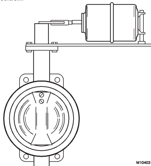
Fig. 6. Butterfly Valve.
