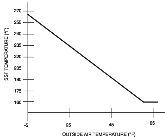
Fig. 139. SSF Temperature Reset Schedule.
