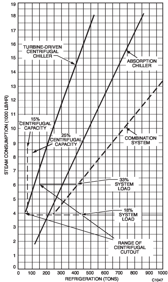
Fig. 23. Typical Steam Consumption, Individual and Combination Chillers.
