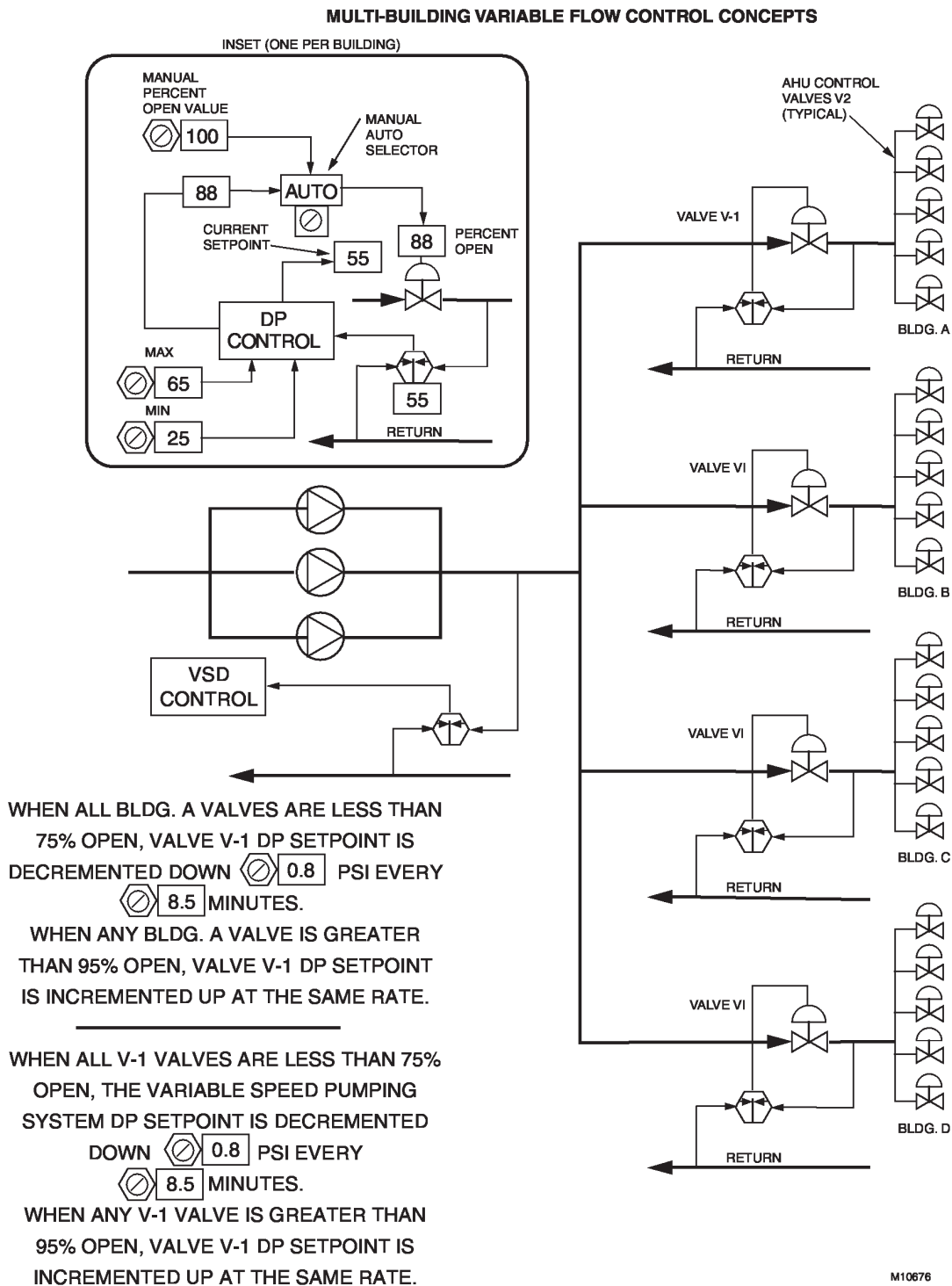
Fig. 82. Multibuilding, Variable Speed Pumping Control.
