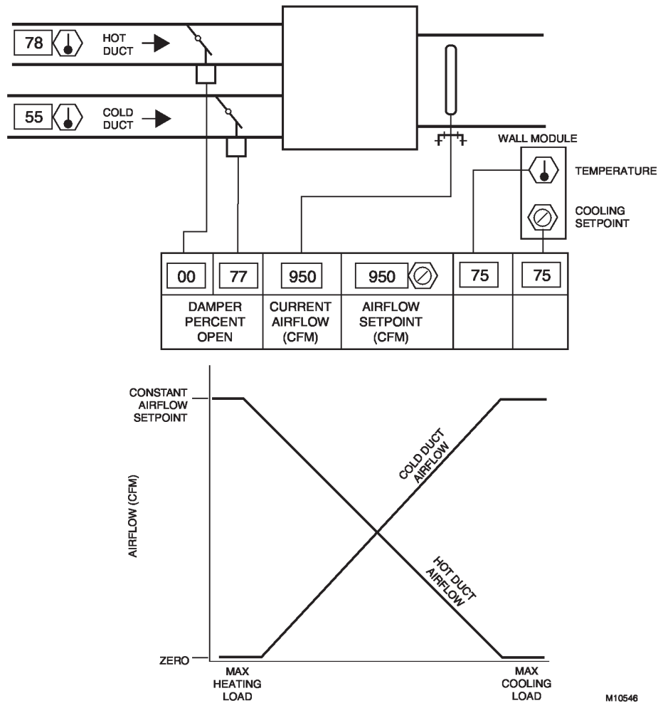
Fig. 11. Dual-Duct Constant Volume Air Terminal Unit.
