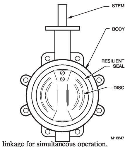
Fig. 4. Butterfly Valve.
