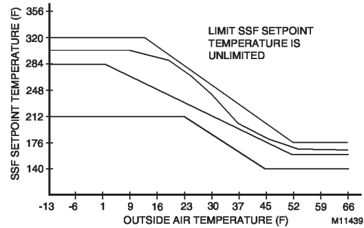
Fig. 137. Adjustment Of Temperature Curves.
