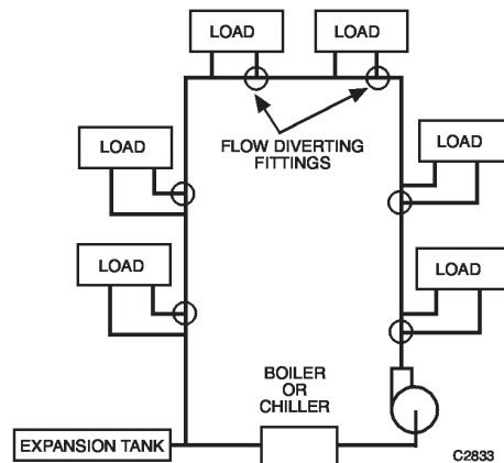
Fig. 85. One-Pipe System.
