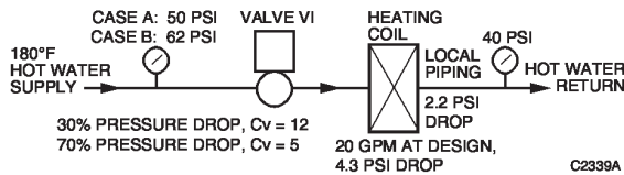
Fig. 17. Equal Percentage Valve Hot Water Application.
