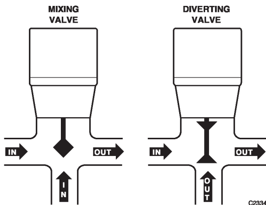
Fig. 12. Three-Way Valves.
