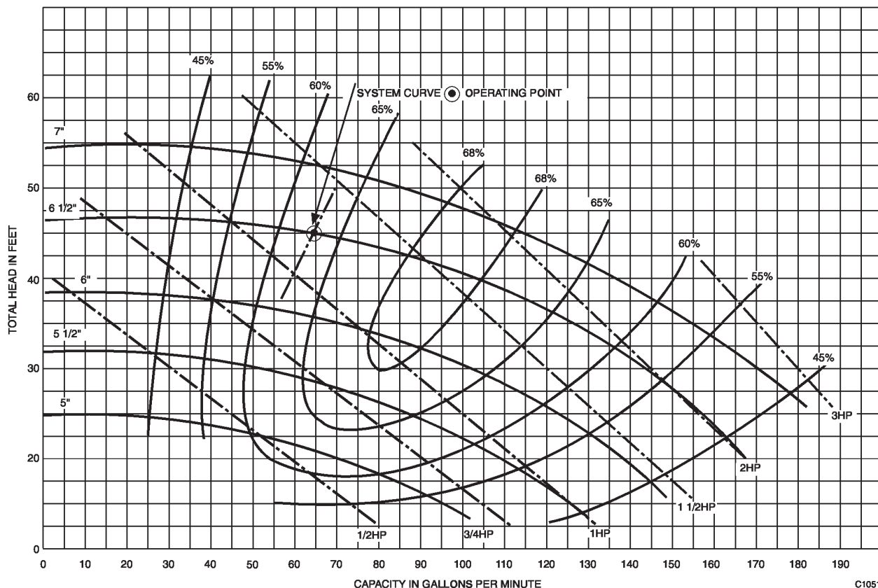
Fig. 55. Pump Curve for 1750 RPM Operation.
