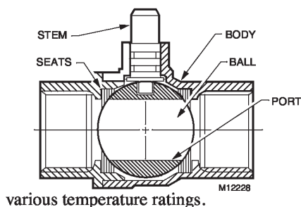
Fig. 3. Ball Valve.
