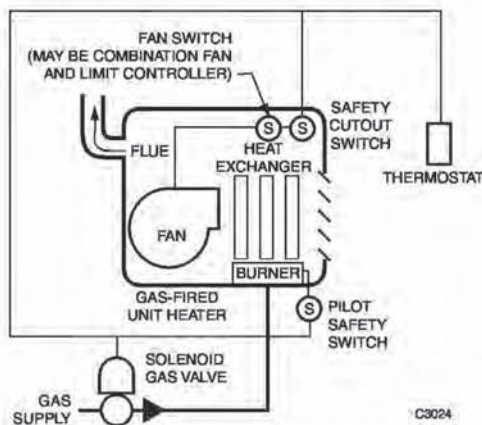
Fig. 19. Gas-Fired Unit Heater.
