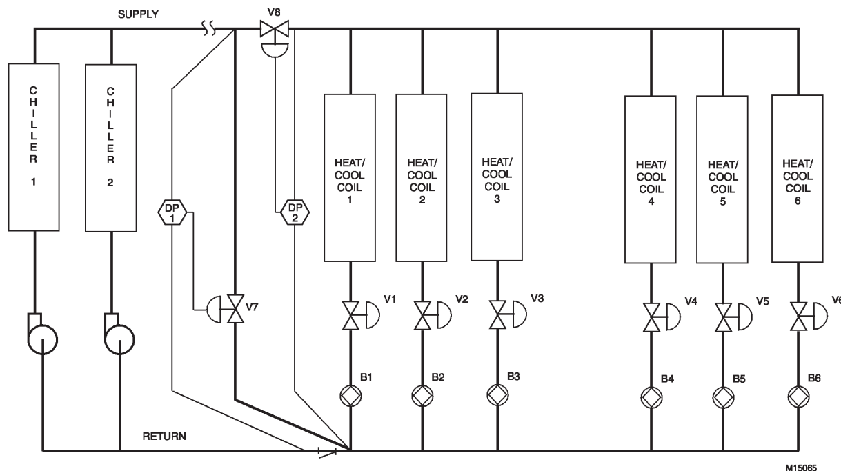
Fig. 78. High AHU Valve Differential Pressure Control
